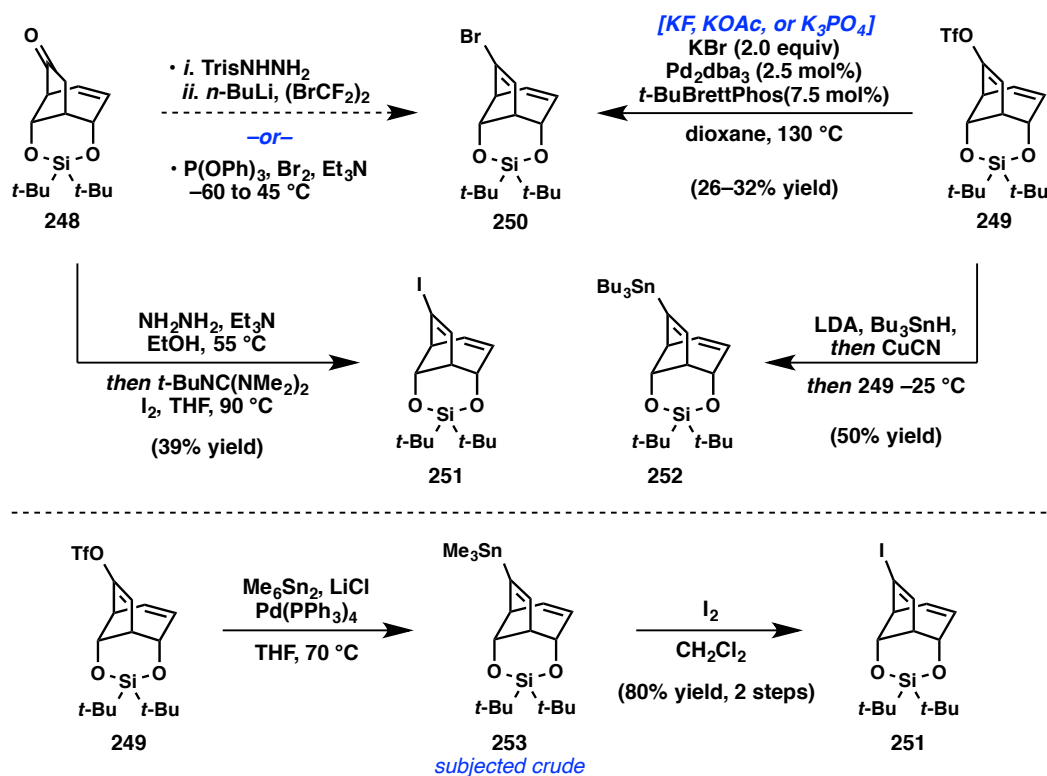
Figure 3.35. Preparation bicyclic vinyl anion precursors.
