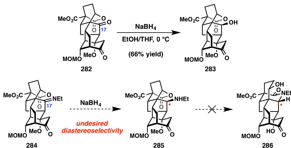
Figure 3.43. Unexpected diastereoselectivity for reduction of the C17 ketone.
