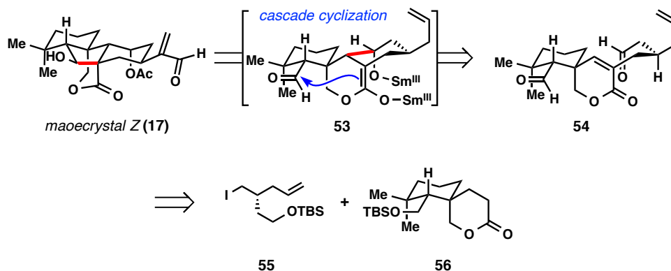
Figure 2.4. Retrosynthetic analysis of (–)-maoecrystal Z ( 17 ).
