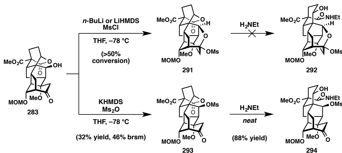
Figure 3.45. Preliminary results for mesylation and aminolysis of lactone 283 .
