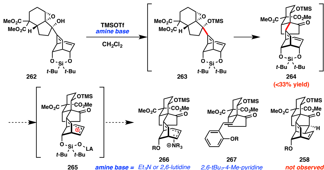
Figure 3.37. Semipinacol rearrangement of 262 and side product formation.
