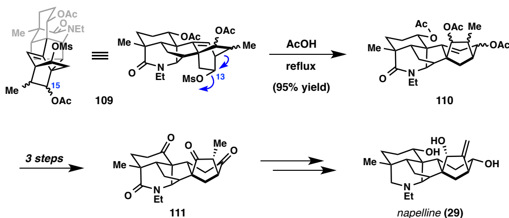
Figure 3.7. Wiesner's total synthesis of napelline ( 29 ).
