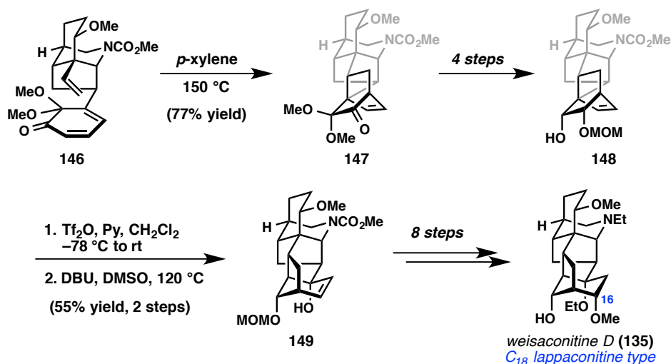
Figure 3.13. Sarpong's total synthesis of weisaconitine D ( 135 ).
