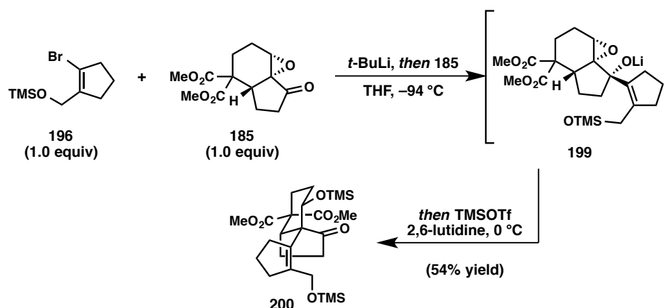
Figure 3.24. One pot 1,2-addition and semipinacol rearrangement.
