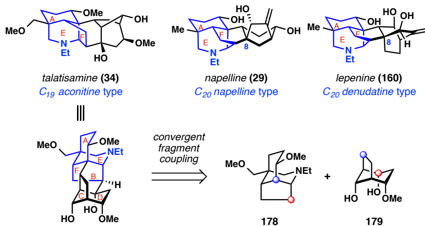
Figure 3.20. Synthetic strategy to convergently access diterpenoid alkaloids.
