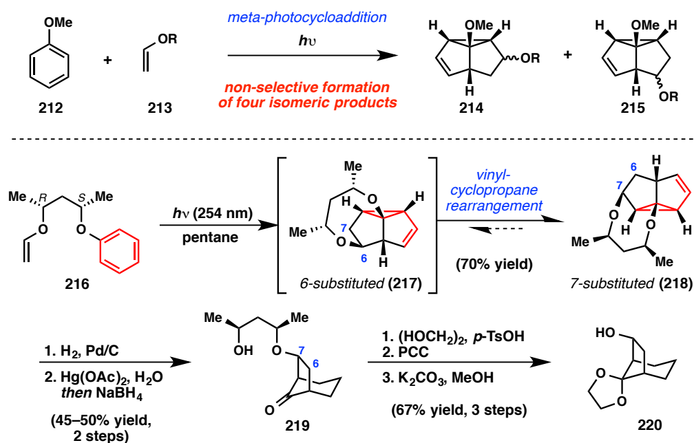
Figure 3.28. Sugimura's diastereoselective meta -photocycloaddition.
