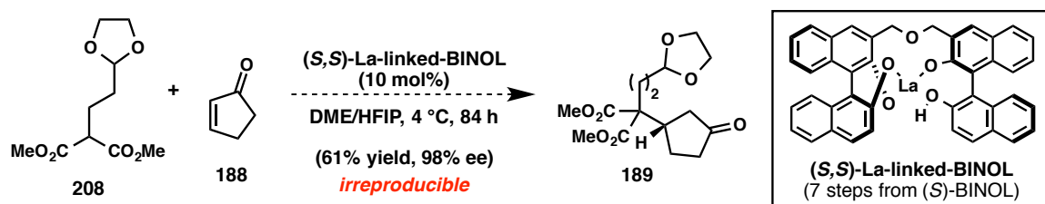
Figure 3.26. Catalytic enantioselective Michael addition of 208 and 188 .
