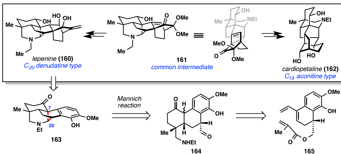
Figure 3.17. Divergent strategy for lepenine ( 160 ) and cardiopetaline ( 162 ).
