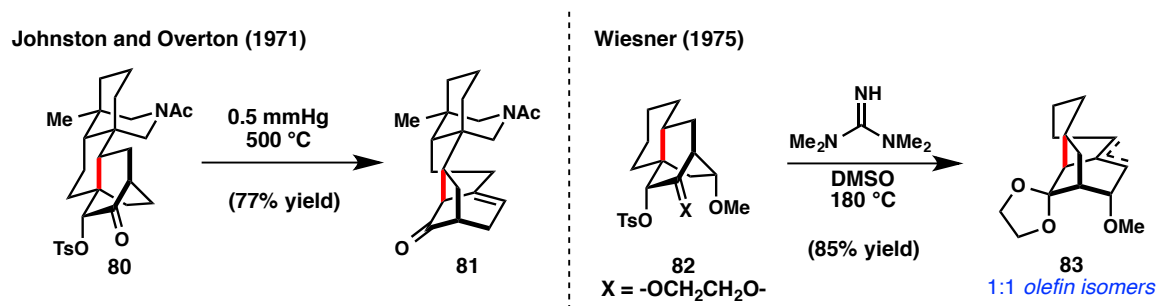
Figure 3.2. Chemical support for biomimetic Wagner–Meerwein rearrangements.
