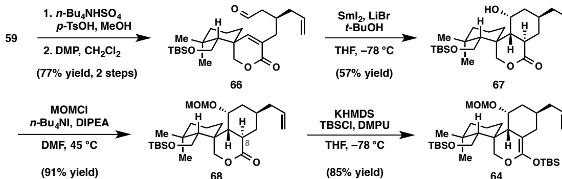
Figure 2.7. Preparation of silyl ketene acetal 64 .
