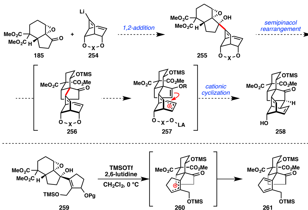
Figure 3.36. Proposed cationic cyclization for carbocyclic core 258 .
