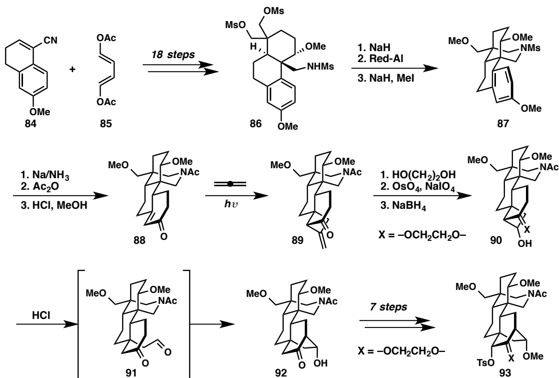
Figure 3.3. Synthesis of Wagner–Meerwein rearrangement precursor 93 .
