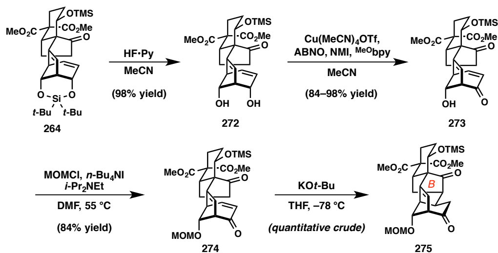
Figure 3.40. Intramolecular Michael addition for carbocyclic core 275 .
