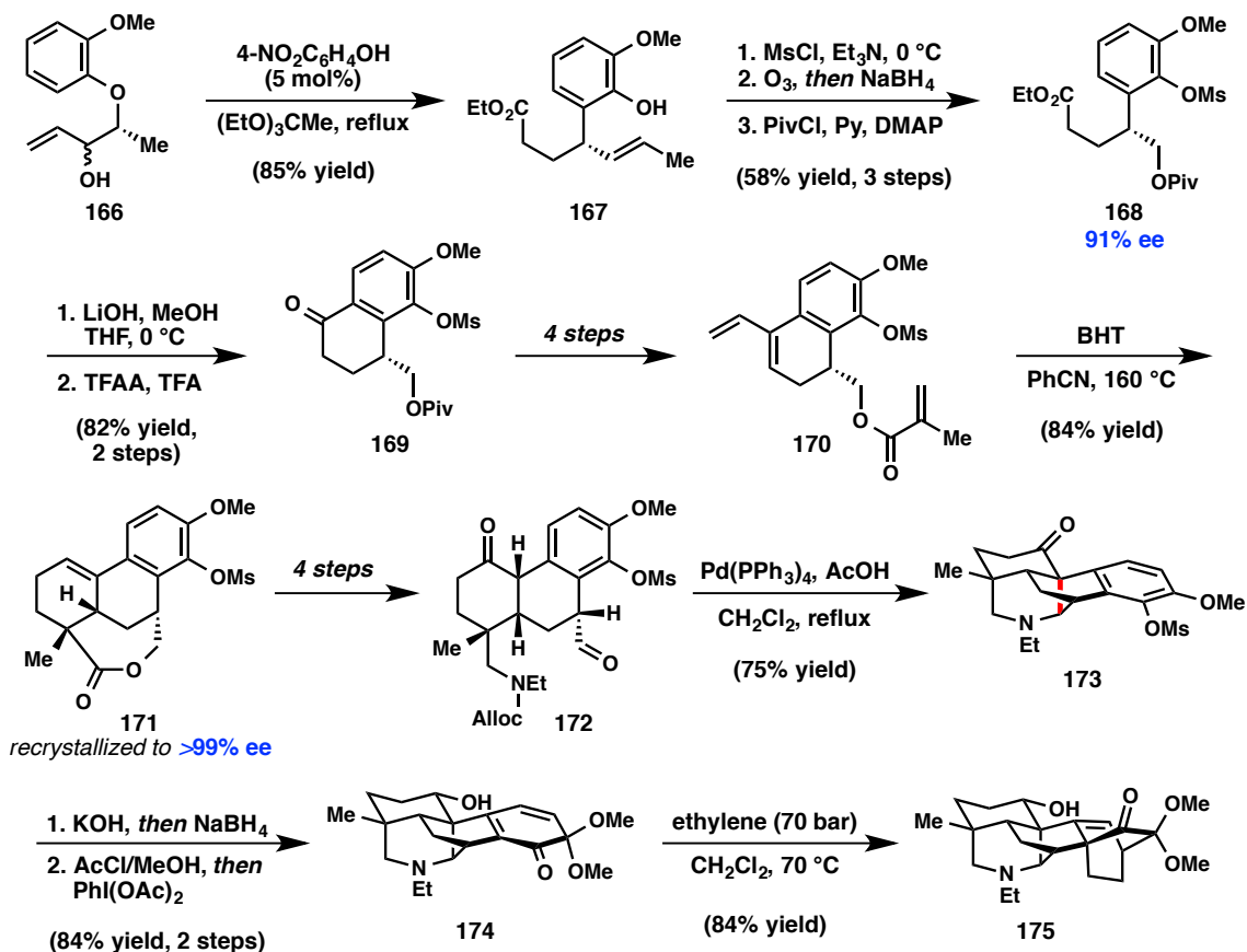
Figure 3.18. Synthesis of denudatine core 175 .
