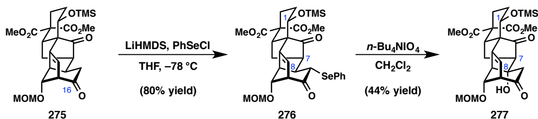
Figure 3.41. Initial investigation of oxy-Michael addition for the C8-alcohol.
