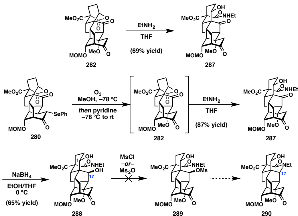
Figure 3.44. Initial investigations on lactone aminolysis.
