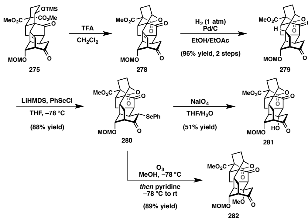
Figure 3.42. Functionalization to C8-methoxylated lactone 282 .
