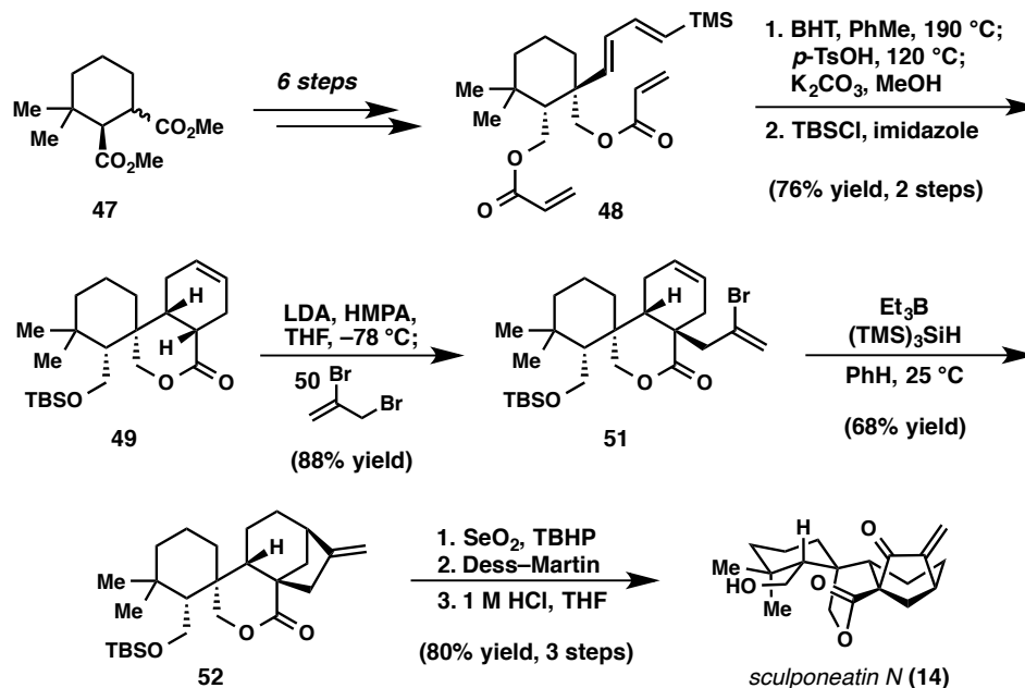
Figure 2.3. Zhai's total synthesis of sculponeatin N ( 14 ).
