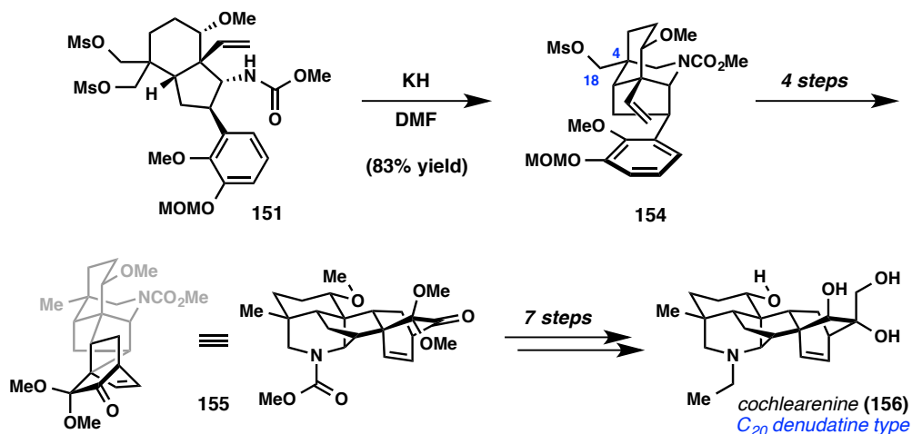
Figure 3.15. Sarpong's total synthesis of cochlearenine ( 156 ).
