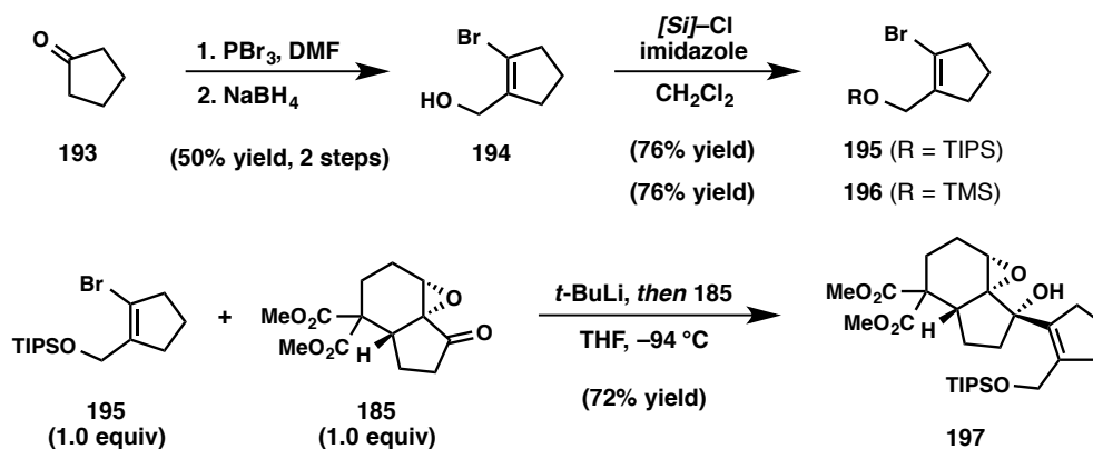
Figure 3.23. Synthesis of semipinacol rearrangement precursor 197 .
