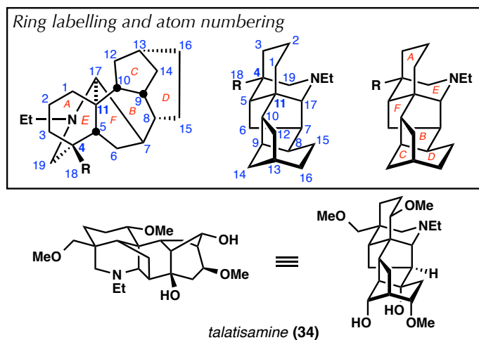
Figure 3.1. Structural depictions of C 19 -Diterpenoid Alkaloids
