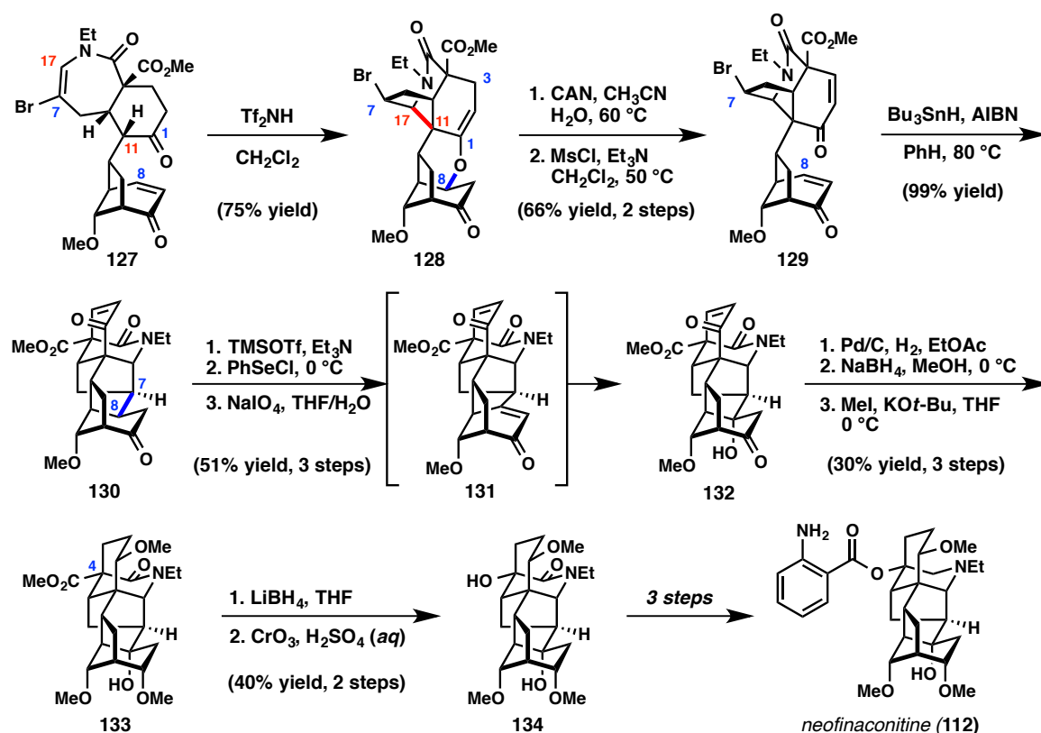
Figure 3.10. Gin's total synthesis of neofinaconitine ( 112 ).
