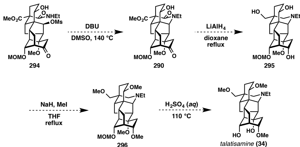
Figure 3.47. Proposed completion of talatisamine ( 34 ).
