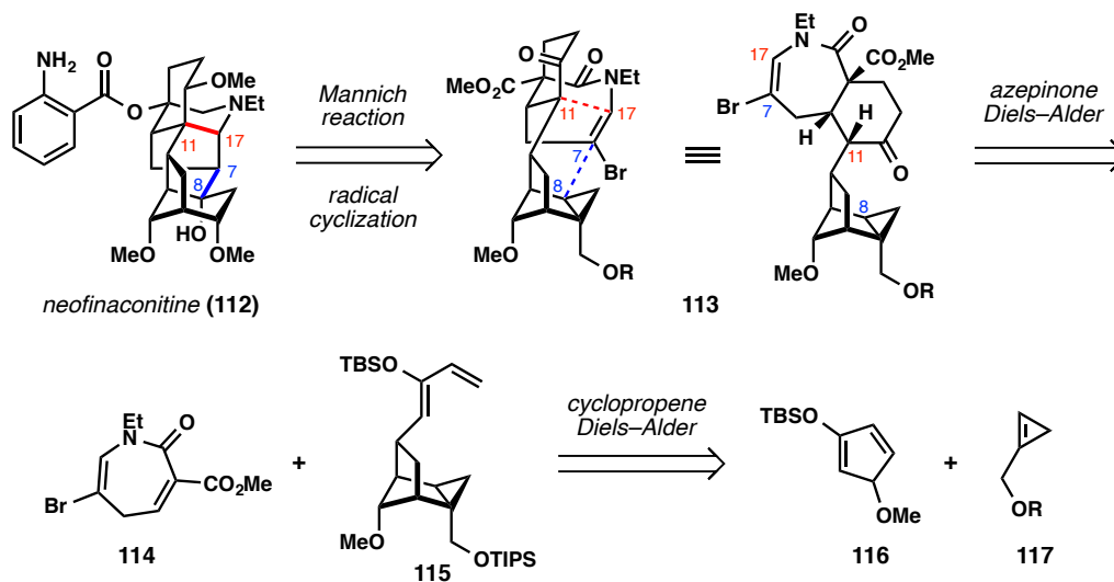
Figure 3.8. Gin's retrosynthetic analysis of neofinaconitine ( 112 ).
