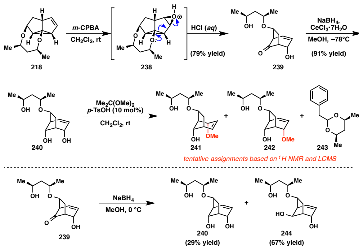
Figure 3.33. Epoxidation of photoadduct 218 and elaboration to triol 240 .
