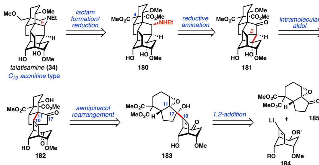
Figure 3.21. Retrosynthetic analysis of talatisamine (34).
