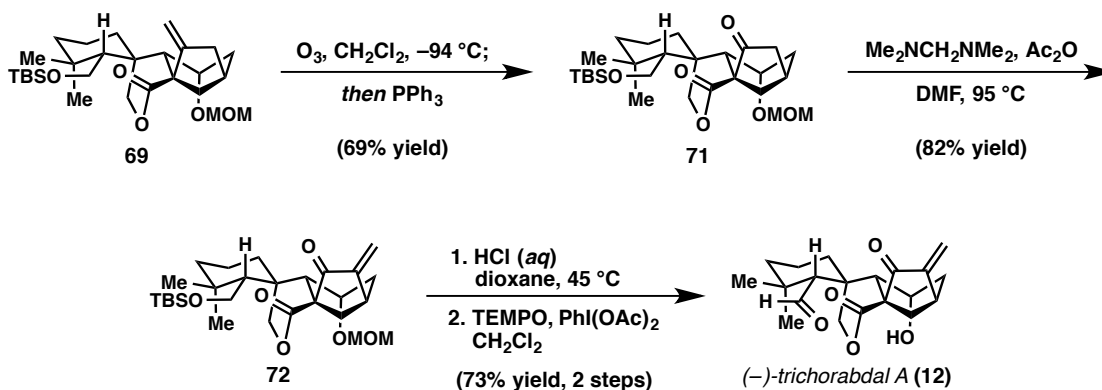
Figure 2.8. Total synthesis of (–)-trichorabdal A ( 12 ).
