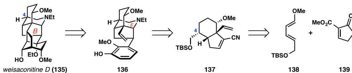
Figure 3.11. Sarpong's retrosynthetic analysis of weisaconitine D ( 135 ).
