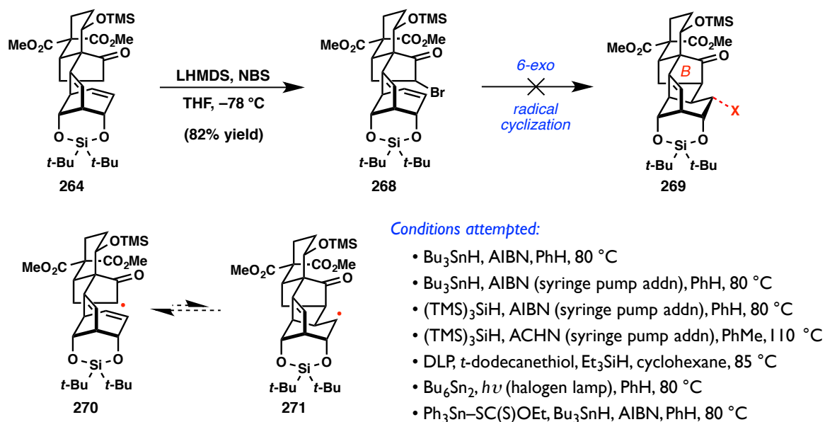
Figure 3.39. Survey of 6- exo radical cyclization conditions for pentacycle 269 .
