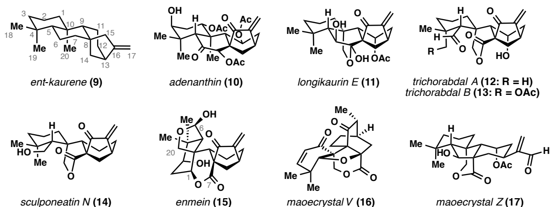
Figure 1.3. Ent -kaurene (9) and representative ent -kauranoids.
