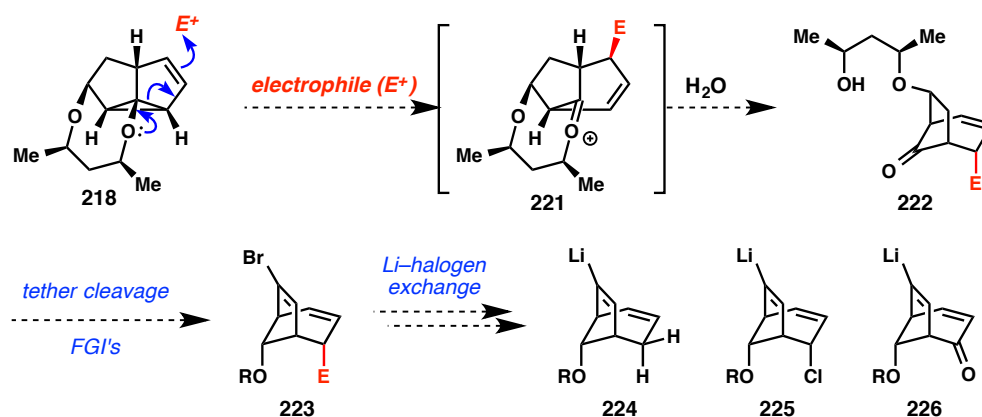
Figure 3.29. Forward plan for elaborating photoadduct 218 .
