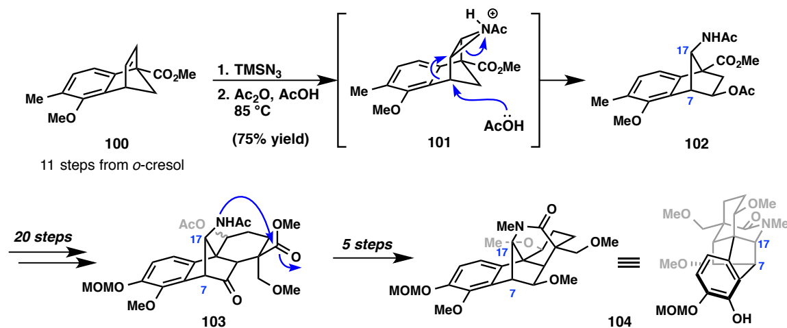
Figure 3.5. Synthesis of pentacyclic aromatic intermediate 104 .
