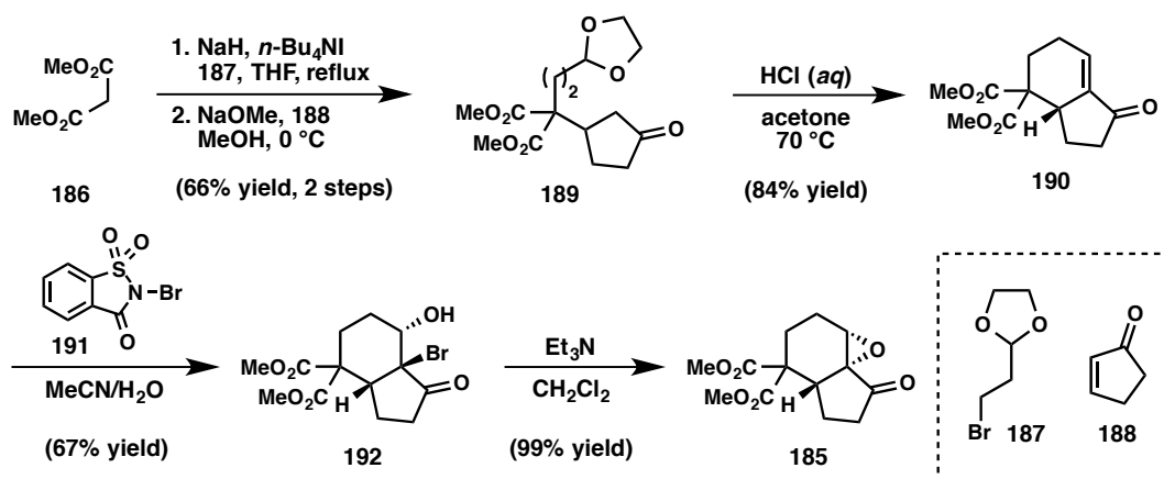
Figure 3.22. Racemic synthesis of epoxyketone 185 .
