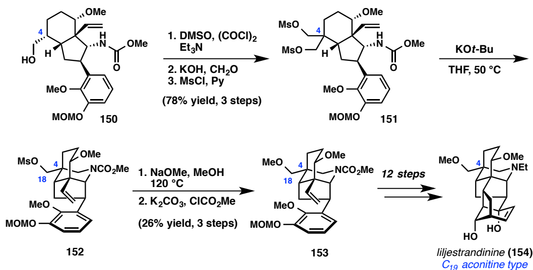
Figure 3.14. Sarpong's total synthesis of liljestrandinine ( 154 ).
