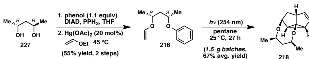
Figure 3.30. Scalable synthesis of photoadduct 218 .
