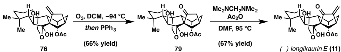
Figure 2.10. Total synthesis of (–)-longikaurin E ( 11 ).
