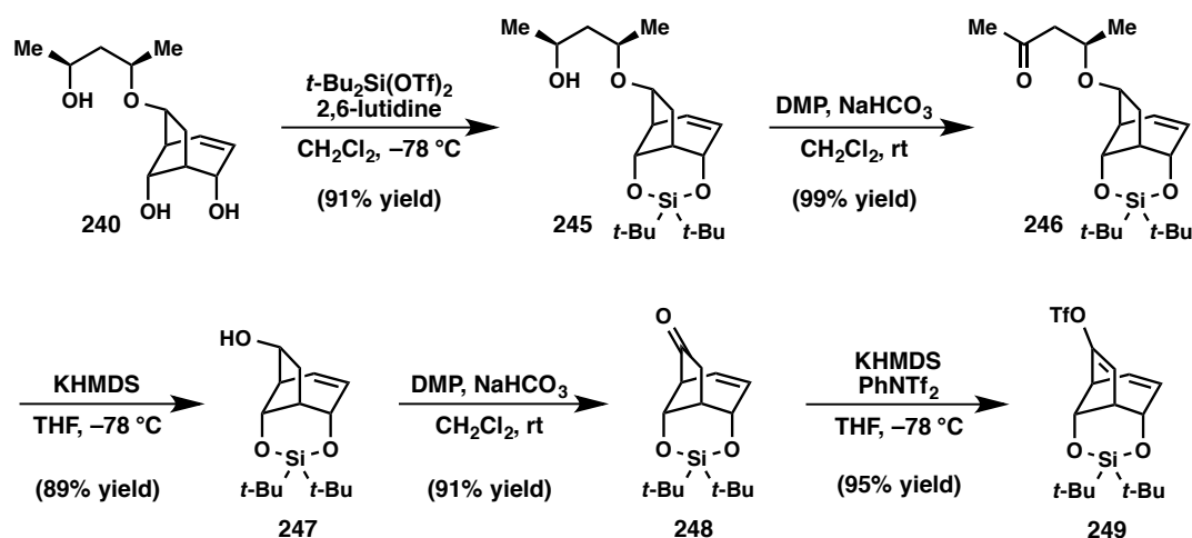
Figure 3.34. Silylene protection and advancement to bicyclic triflate 249 .
