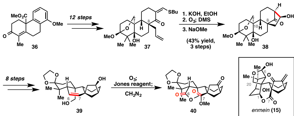
Figure 2.1. Key transformations in Fujita's relay synthesis of enmein ( 15 ).
