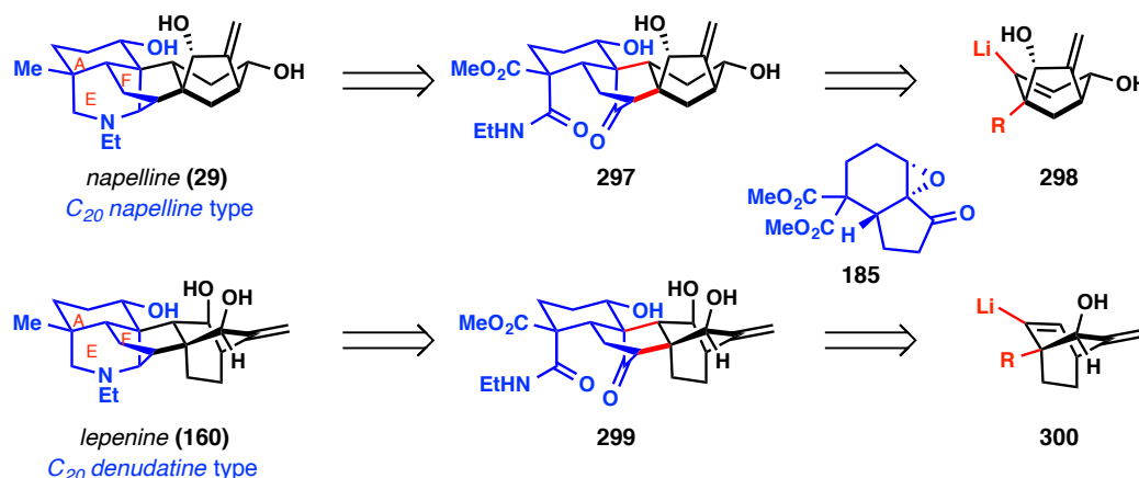
Figure 3.47. Retrosynthetic analysis of C 20 -diterpenoid alkaloids.
