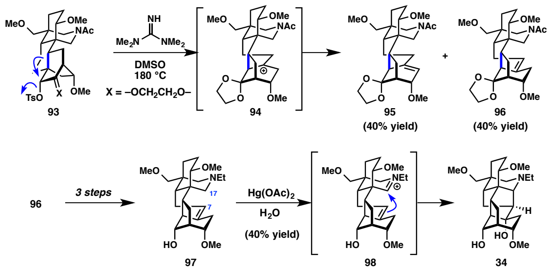
Figure 3.4. Wiesner's total synthesis of talatisamine ( 34 ).
