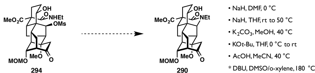
Figure 4.46. Preliminary investigations on lactam ring closure.
