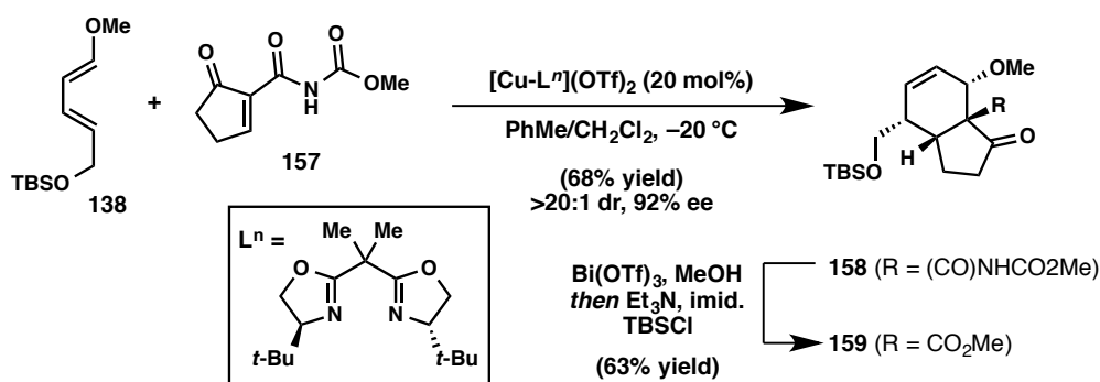
Figure 3.16. Enantioselective [4 + 2] for the synthesis of hydrindane 159 .
