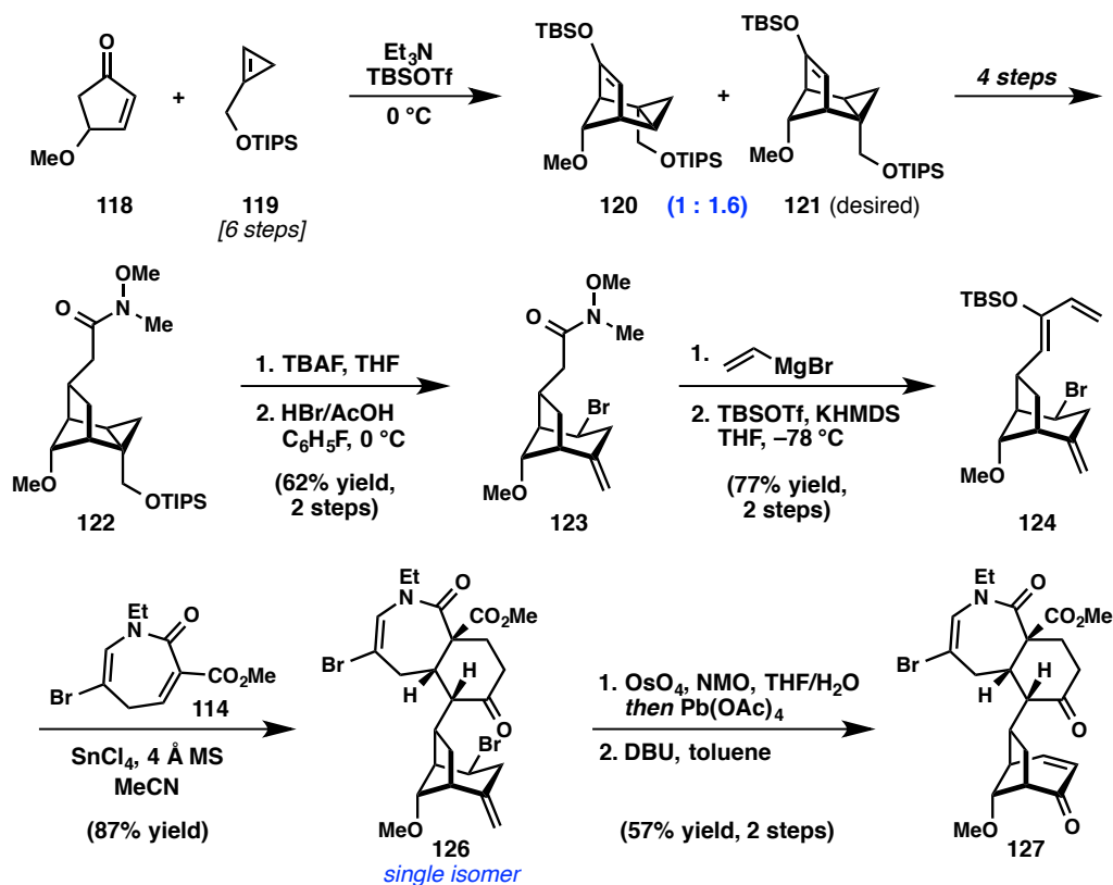
Figure 3.9. Convergent assembly of Mannich cyclization precursor 127 .
