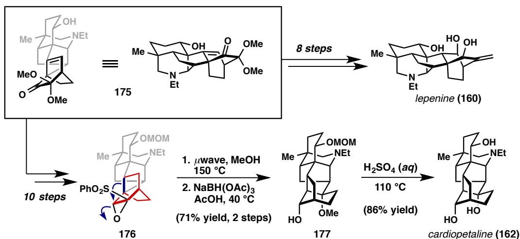
Figure 3.19. Fukuyama's total syntheses of lepenine ( 160 ) and cardiopetaline ( 162 ).
