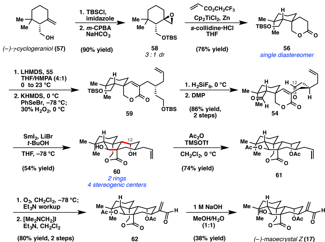
Figure 2.5. Total synthesis of (–)-maoecrystal Z ( 17 ).
