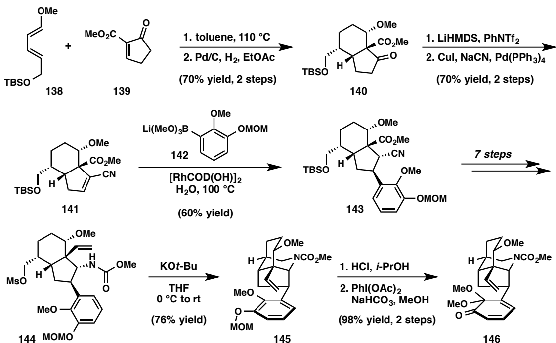
Figure 3.12. Preparation of intramolecular Diels–Alder precursor 146 .
