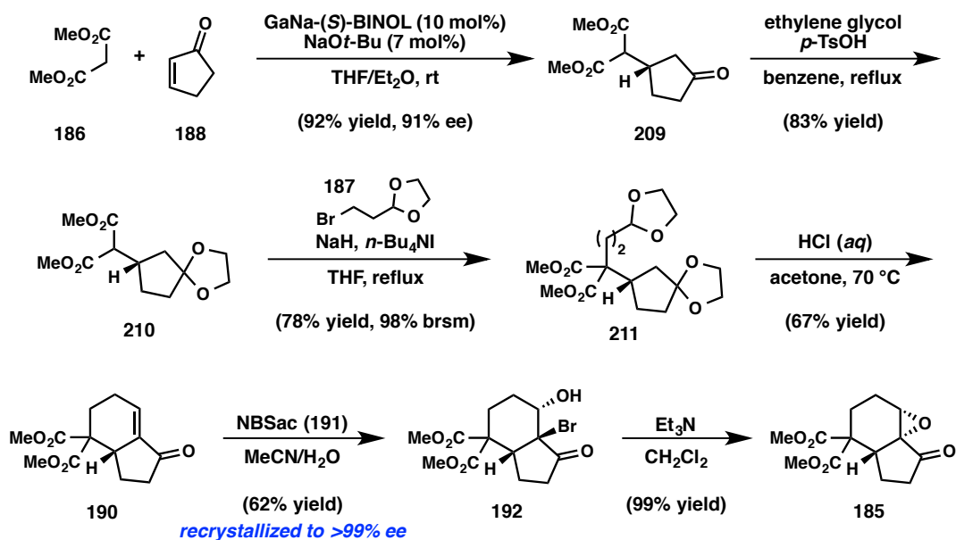
Figure 3.27. Alternative enantioselective route to epoxyketone 185 .
