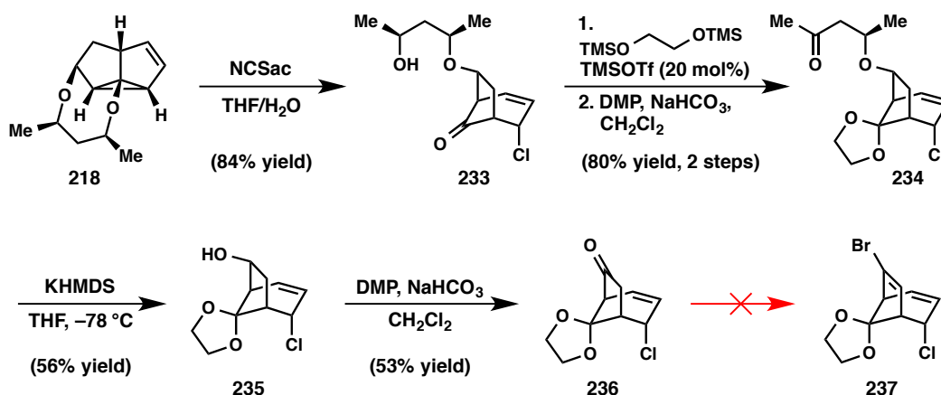
Figure 3.32. Synthesis of a chlorinated bicyclo[3.2.1]octane.
