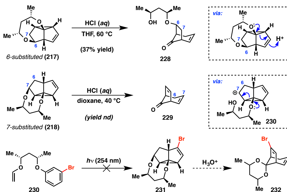
Figure 3.31. Acidolysis of meta -photoadducts.
