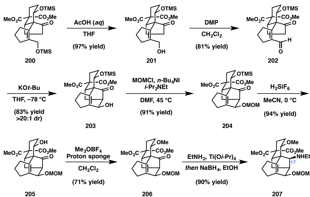
Figure 3.25. Investigations on intramolecular aldol and reductive amination steps.
