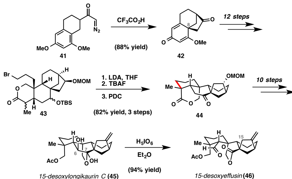
Figure 2.2. Mander's synthesis of 15-desoxy analogues.
