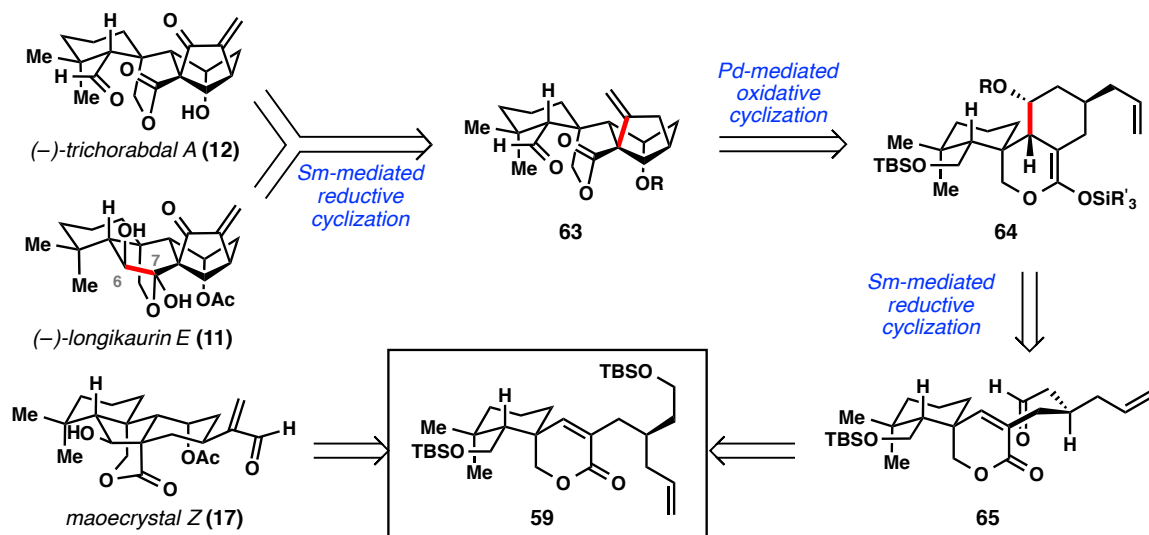
Figure 2.6. Retrosynthesis of (–)-trichorabdal A ( 12 ) and (–)-longikaurin E ( 11 ).
