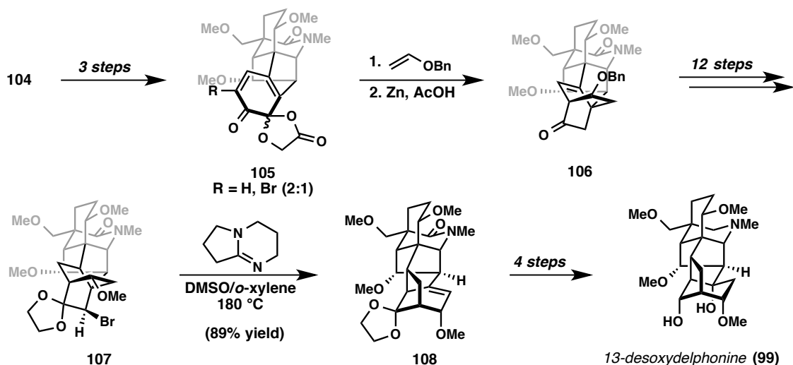
Figure 3.6. Wiesner's total synthesis of 13-desoxydelphonine ( 99 ).
