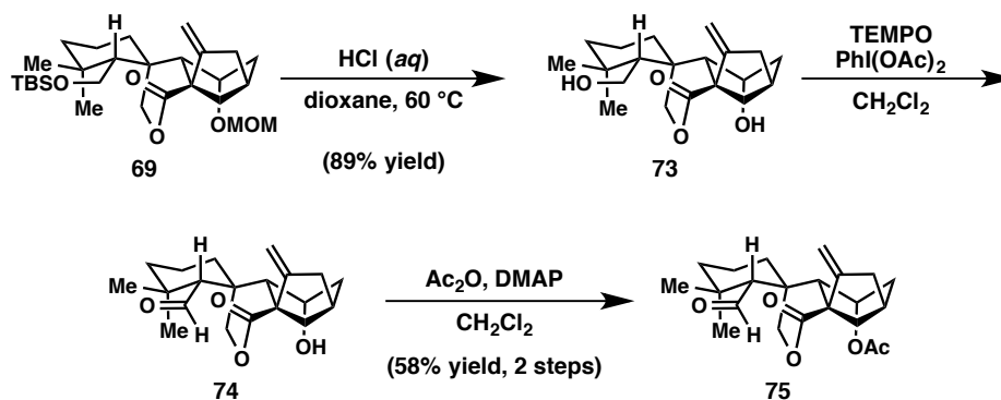
Figure 2.9. Synthesis of aldehyde-lactone 75 .
