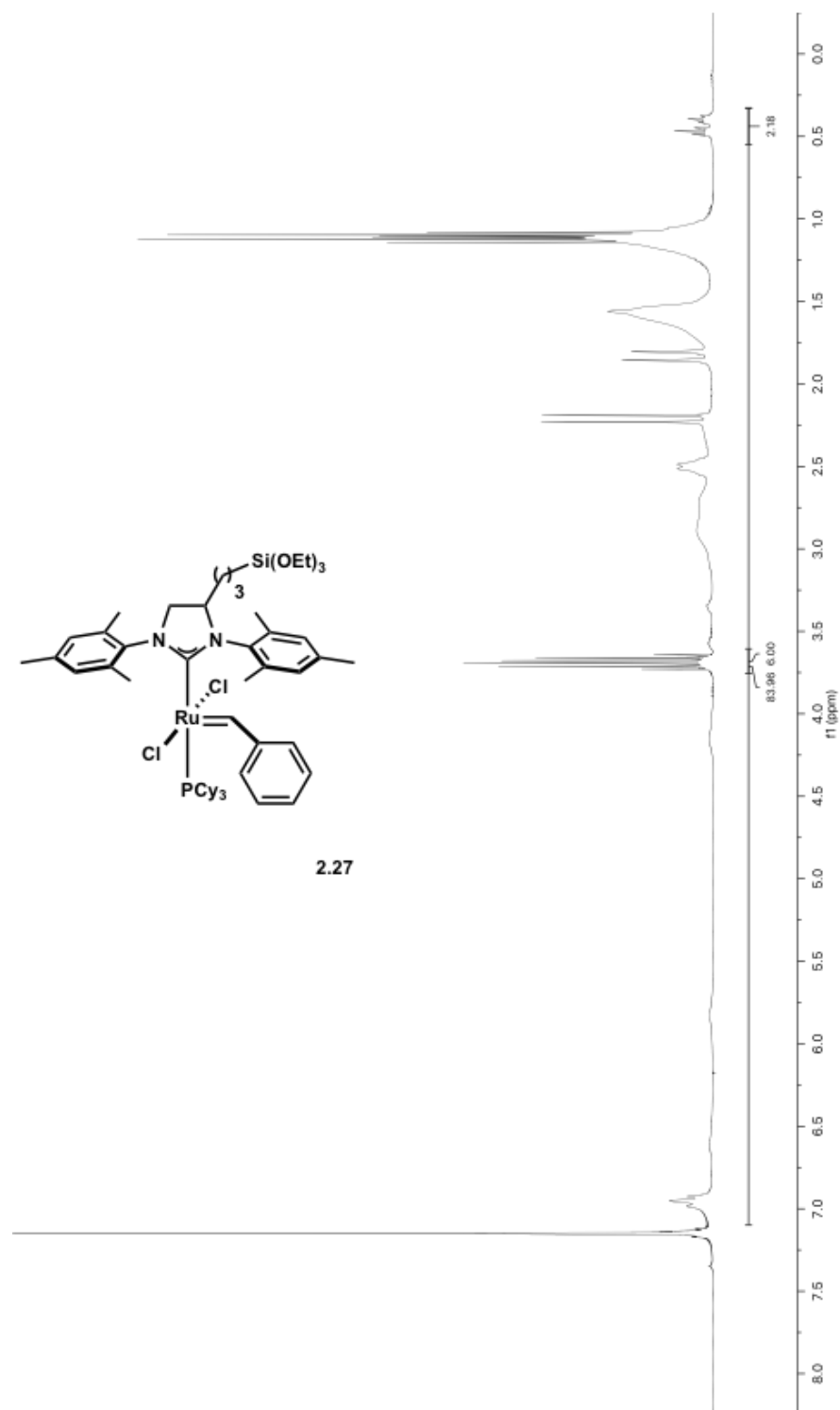
Figure A.10 | ^1\text{H} NMR Spectrum of 2.27
