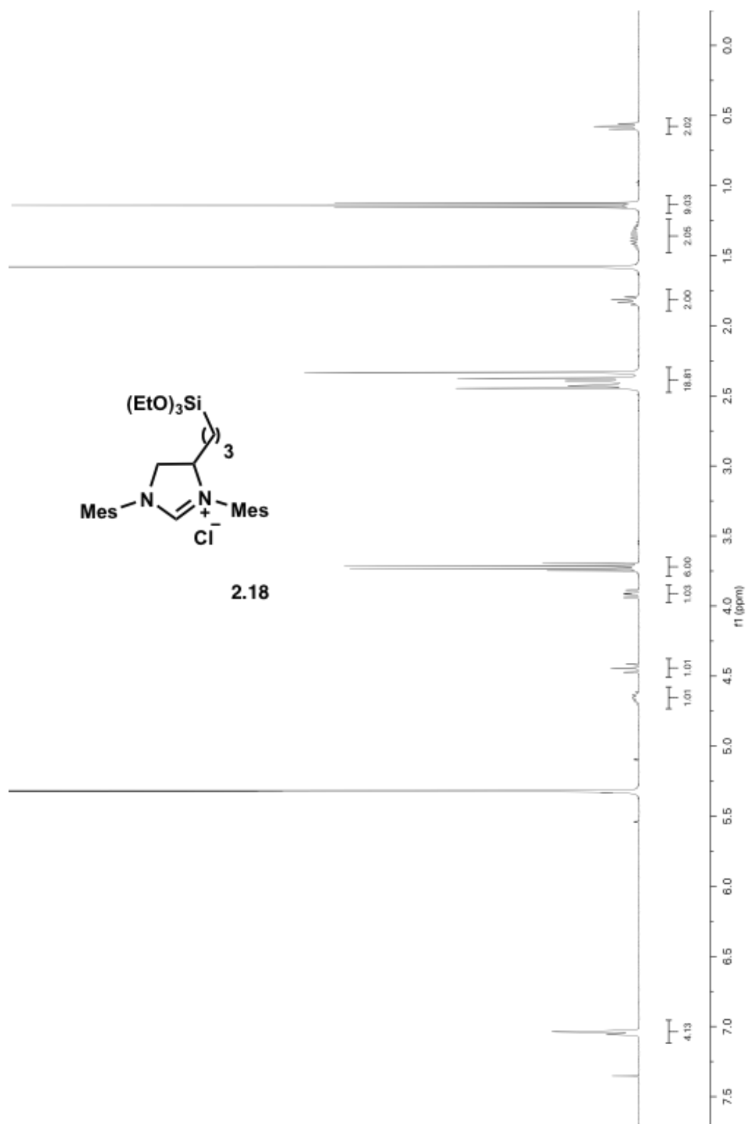
Figure A.1 | ^1\text{H} NMR spectrum for 2.18
