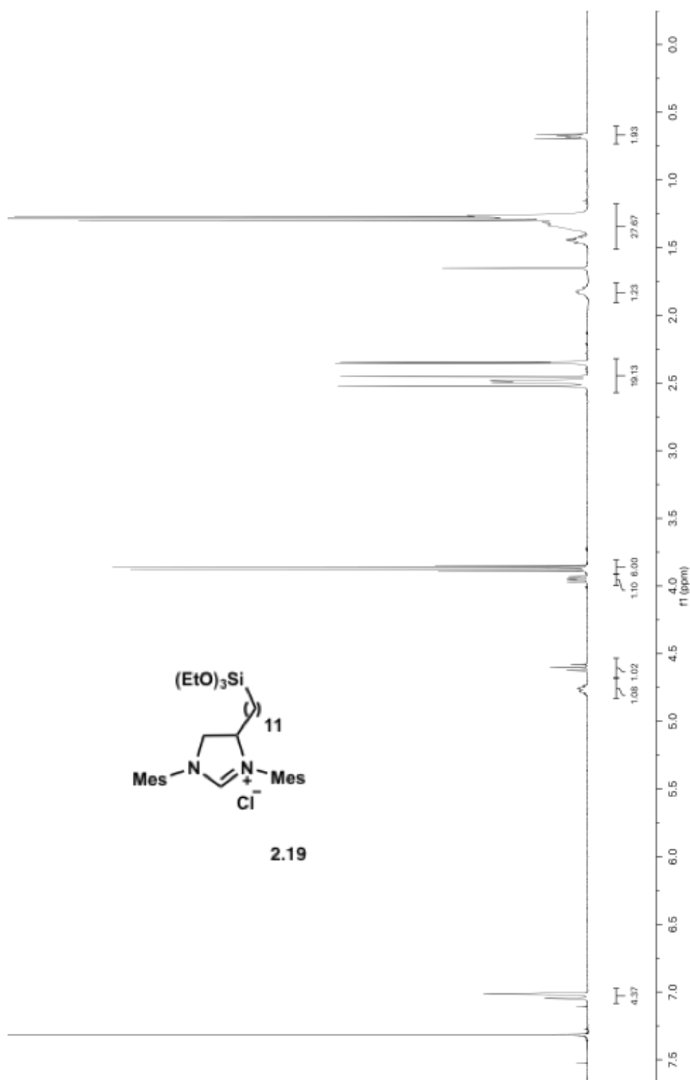
Figure A.2 | ^1\text{H} NMR spectrum for 2.19
