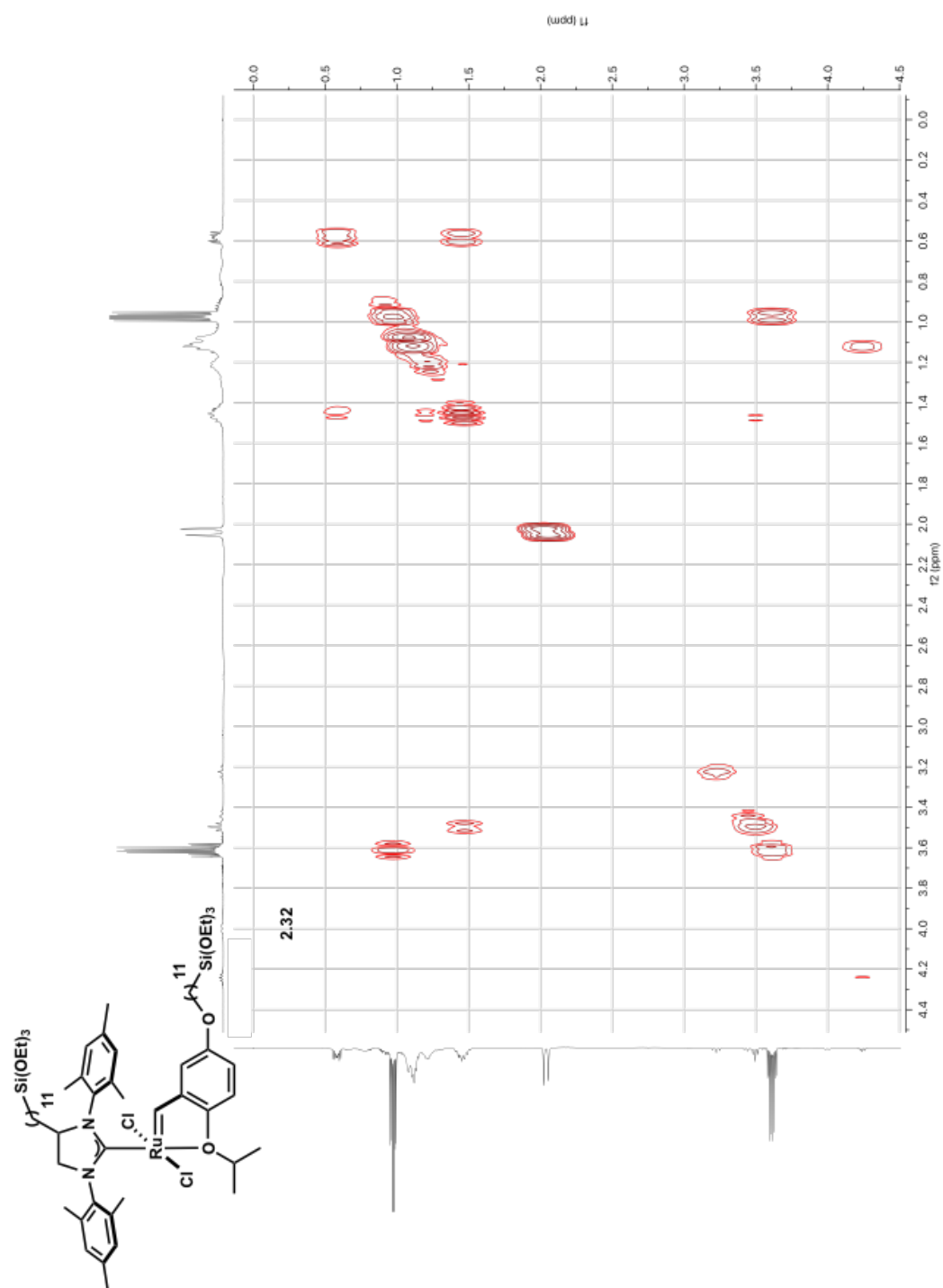
Figure A.18 | COSY NMR Spectrum of 2.32
