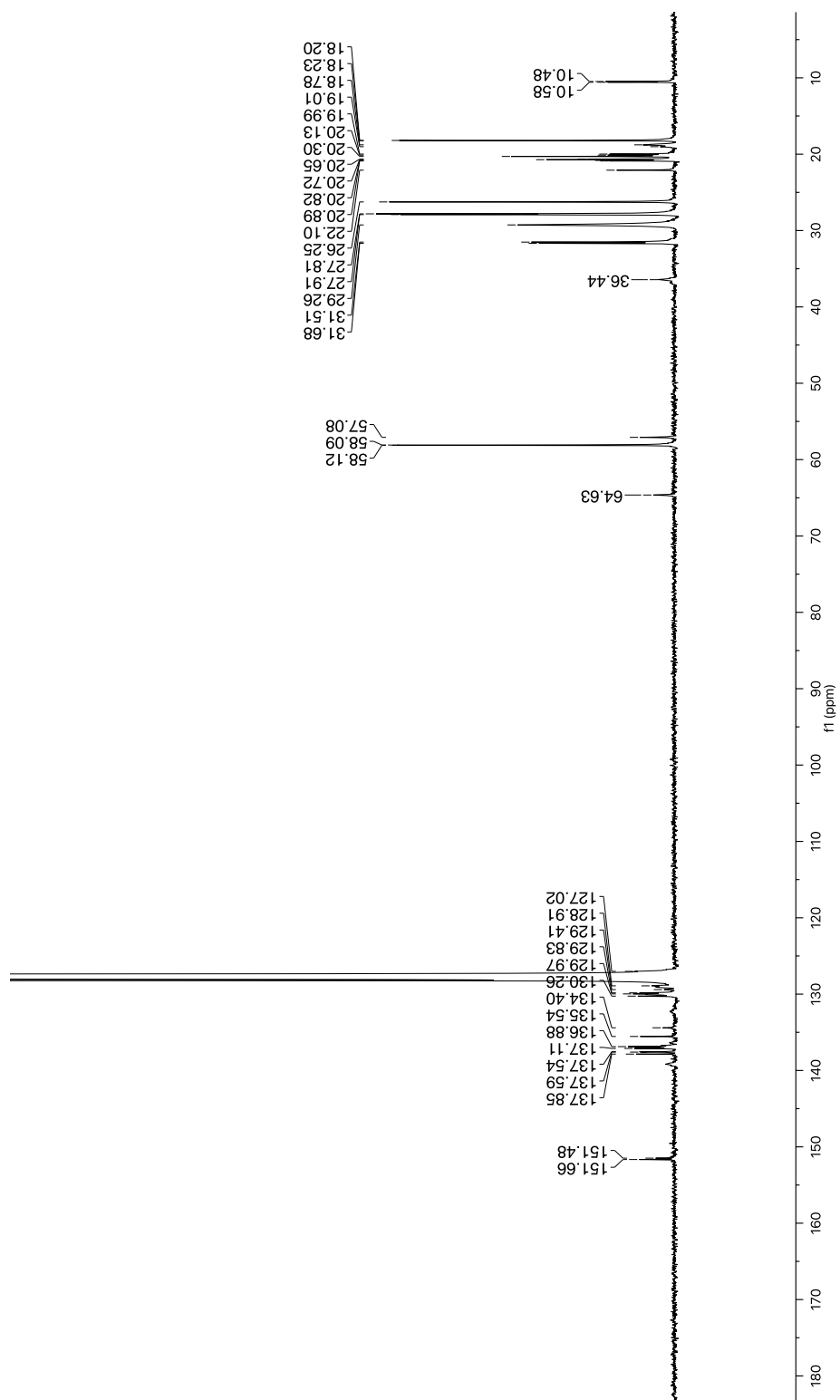
Figure A.11 | ^{13}\text{C} NMR Spectrum of 2.27
