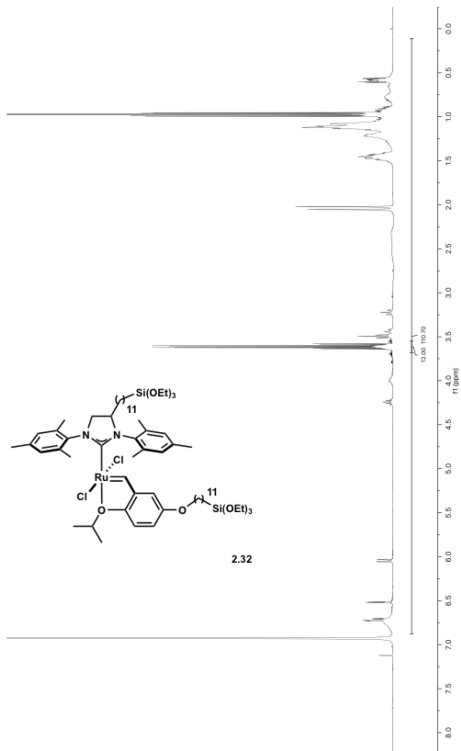
Figure A.17 | ^1\text{H} NMR Spectrum of 2.32
