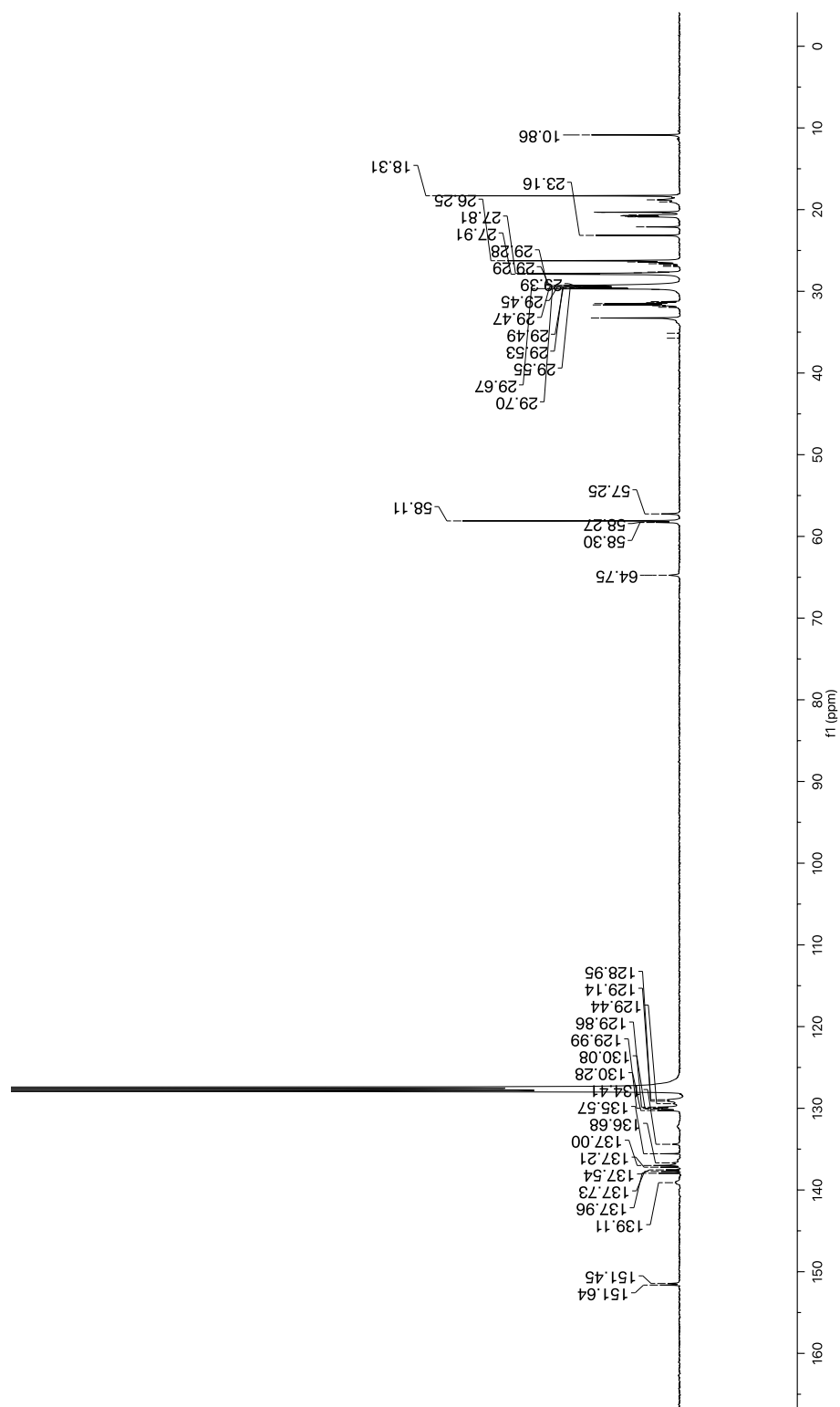
Figure A.13 | 13 C NMR Spectrum of 2.28
