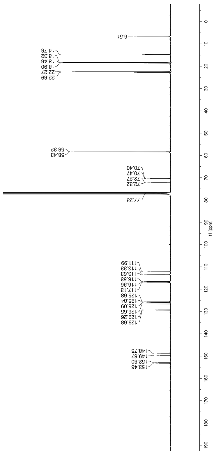
Figure A.7 | 13 C NMR Spectrum of 2.25
