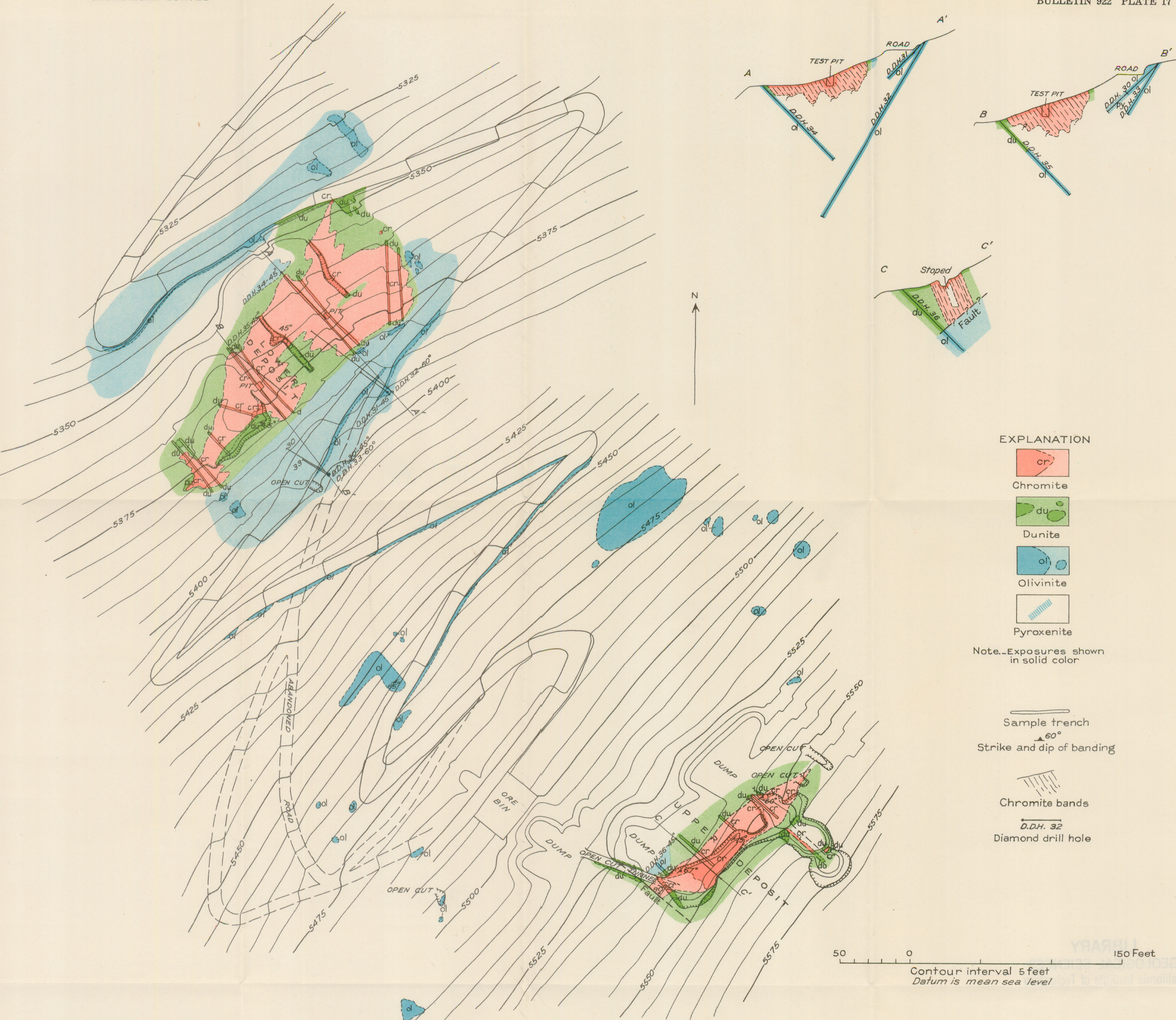
GEOLOGIC MAP AND SECTIONS OF DRY CAMP CHROMITE DEPOSIT
