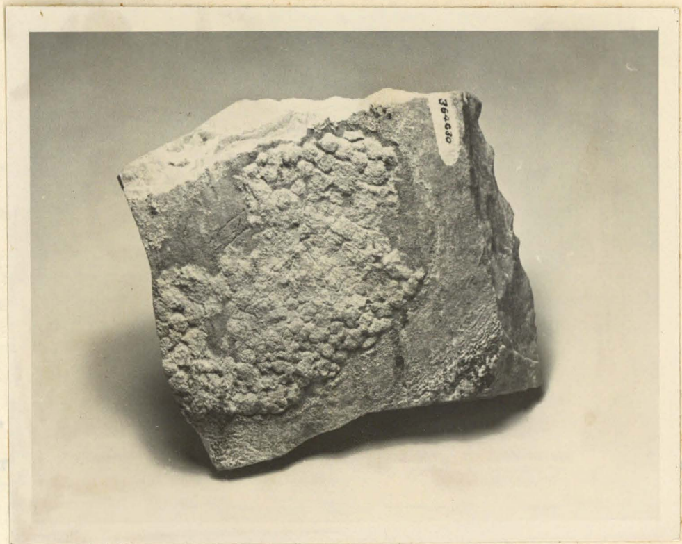
Figure 59 and 60. Incrustations on marble in the Kernville series, Mine area. Possible organic remains. One and one-half miles east of Rockhouse basin, junction of Fish creek and South Fork of the Kern river.
