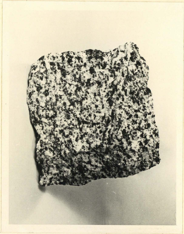
Figure 36. Typical quartz-diorite of the Sacatar unit. From the head of Sacatar canyon. Three-quarters natural size.
