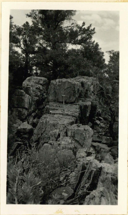
Figure 29. Outcrop of rolled gneiss, summit of 7285 hill. (T23S, R36E, sec. 6.)
