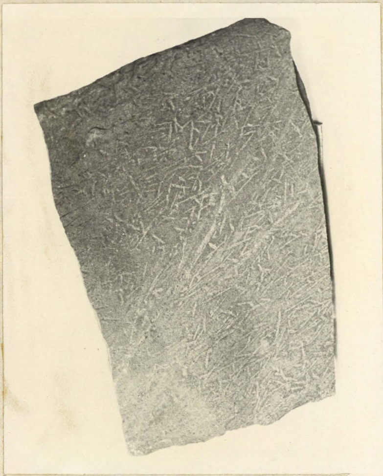
Figure 58. Graptolite-like rods in the Kernville series of the Mine area.
