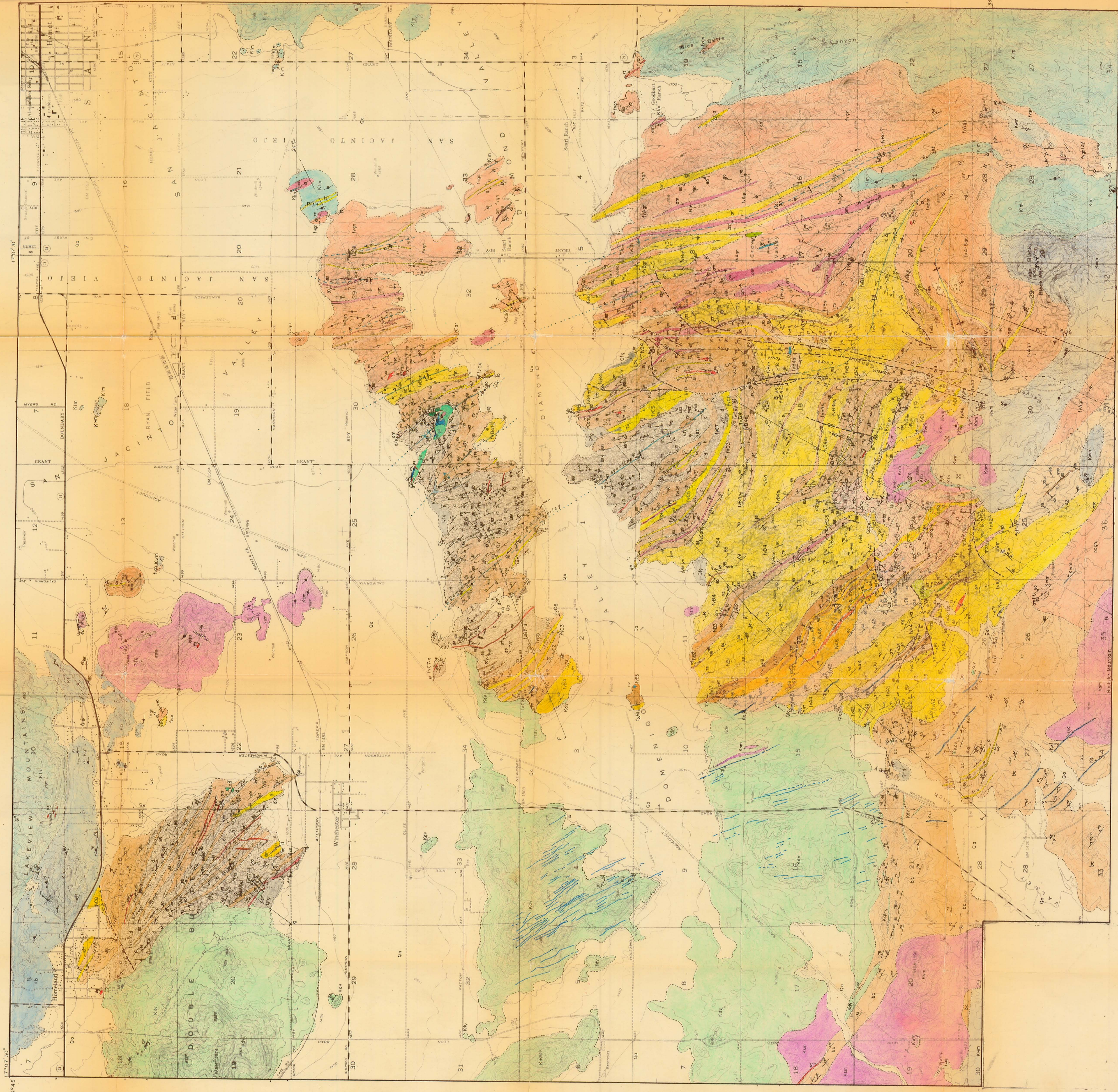
GEOLOGIC MAP OF THE WINCHESTER-HEMET AREA, RIVERSIDE CO., CALIFORNIA.
