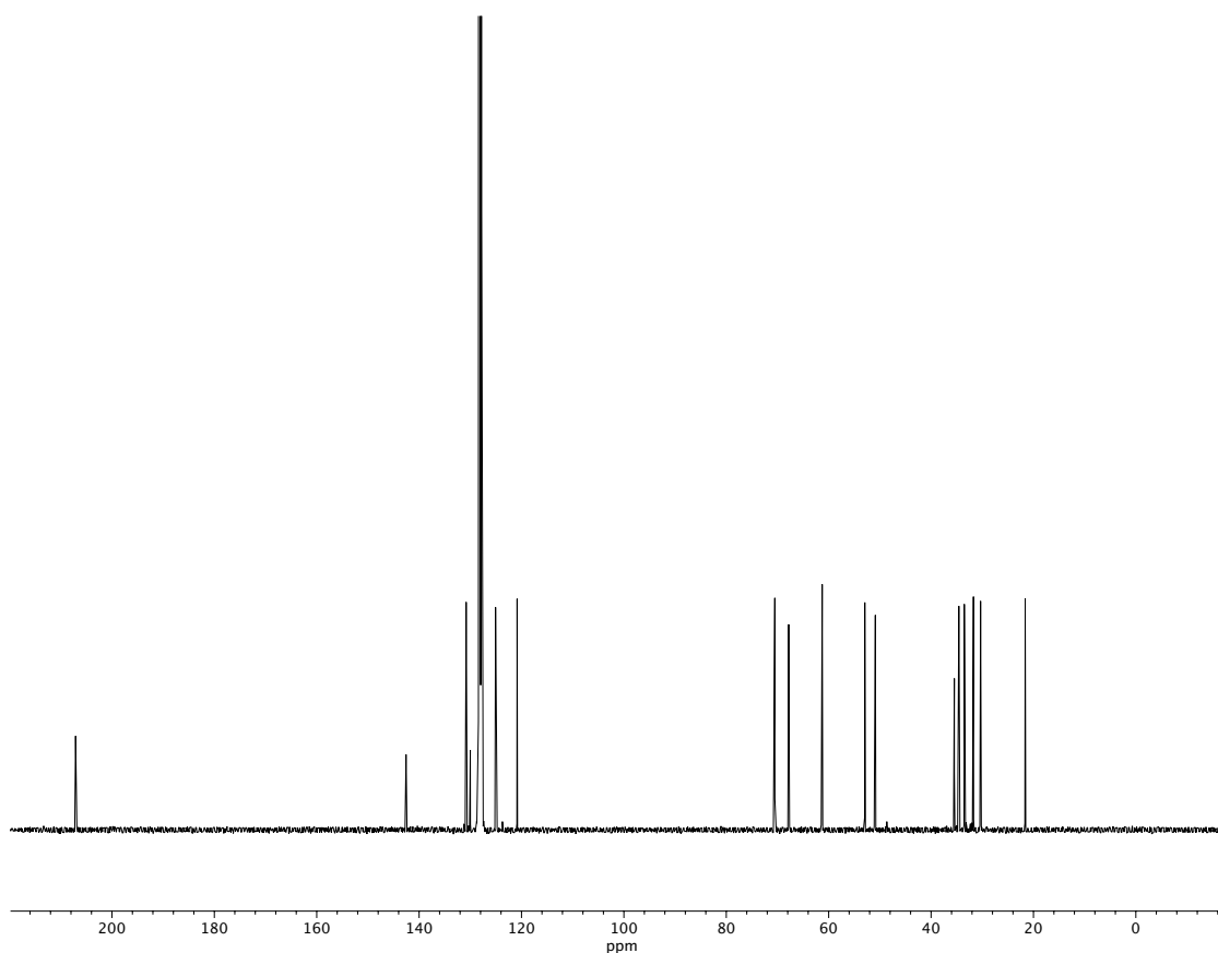
Figure A3.92 13 C NMR (100 MHz, C 6 D 6 ) of compound 116 .
