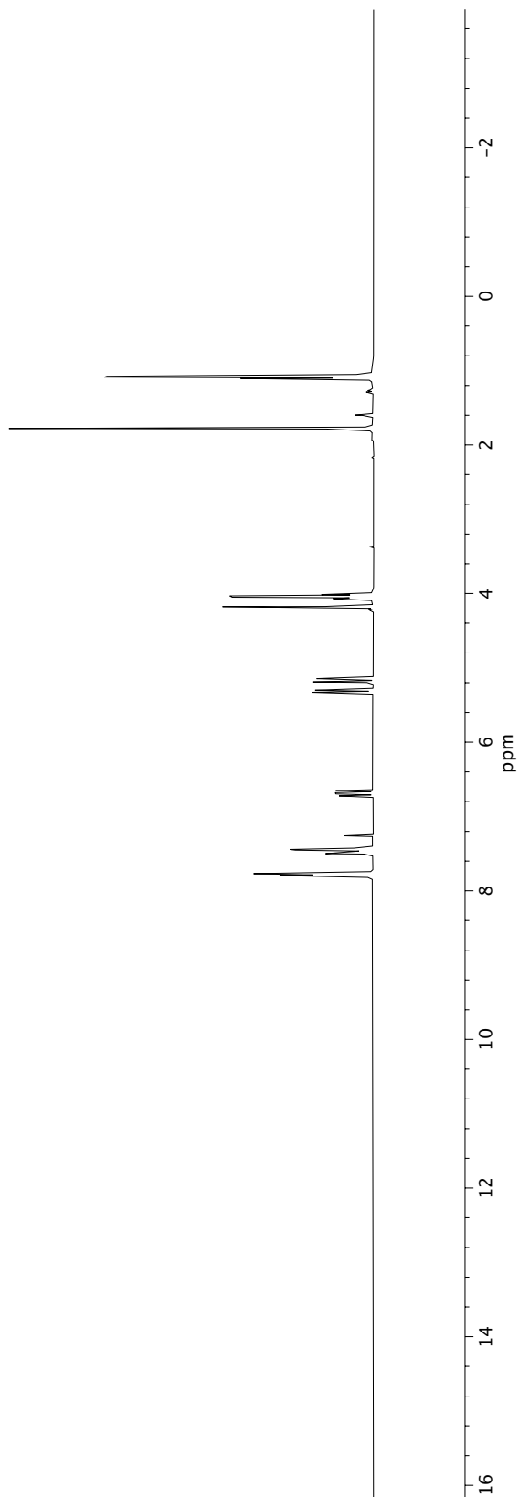
Figure A1.13 ^1\text{H} NMR (400 MHz, \text{CDCl}_3 ) of compound 32b .
