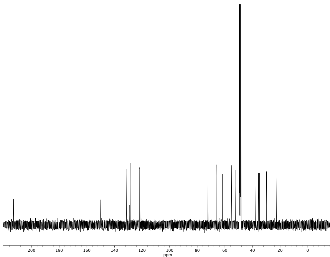
Figure A3.100 13 C NMR (100 MHz, CD 3 OD) of compound 53 .
