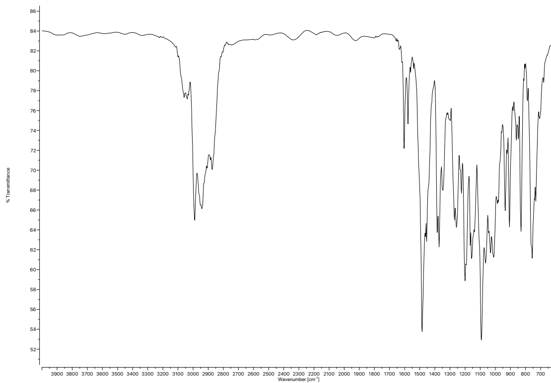
Figure A5.23 Infrared spectrum (Thin Film, NaCl) of compound 155 .
