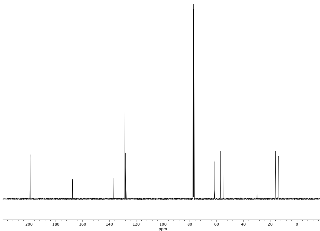
Figure A1.74 13 C NMR (100 MHz, CDCl 3 ) of compound 41 .
