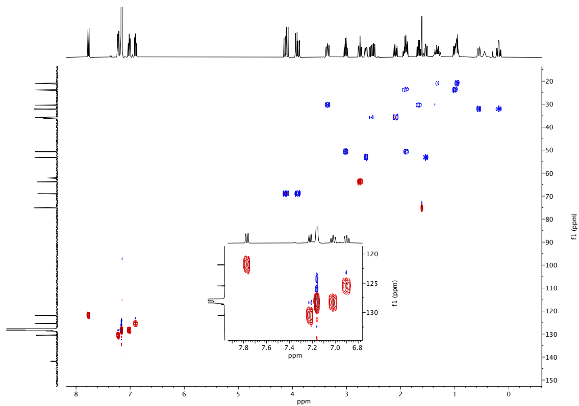
Figure A3.97 HSQC spectrum ( \text{C}_6\text{D}_6 ) of compound 117 .
