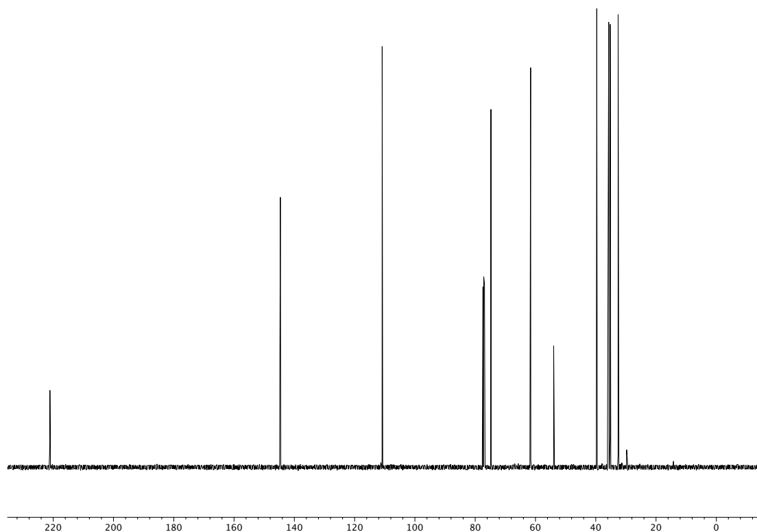
Figure A3.18 13 C NMR (125 MHz, CDCl 3 ) of compound 70 .
