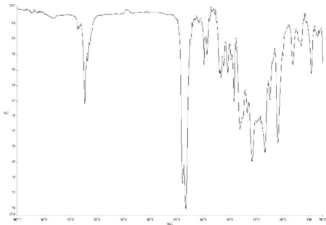
Figure A1.20 Infrared spectrum (Thin Film, NaCl) of compound 32d .
