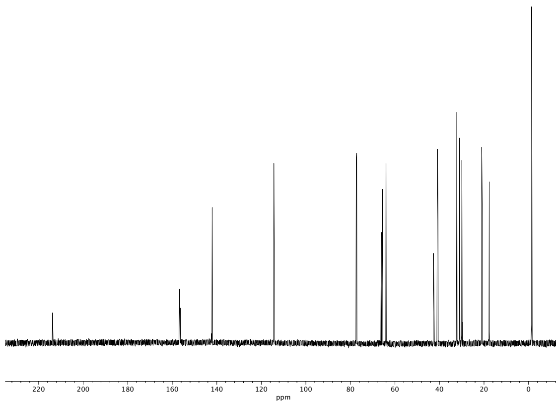
Figure A1.51 13 C NMR (150 MHz, CDCl 3 ) of compound 67c .
