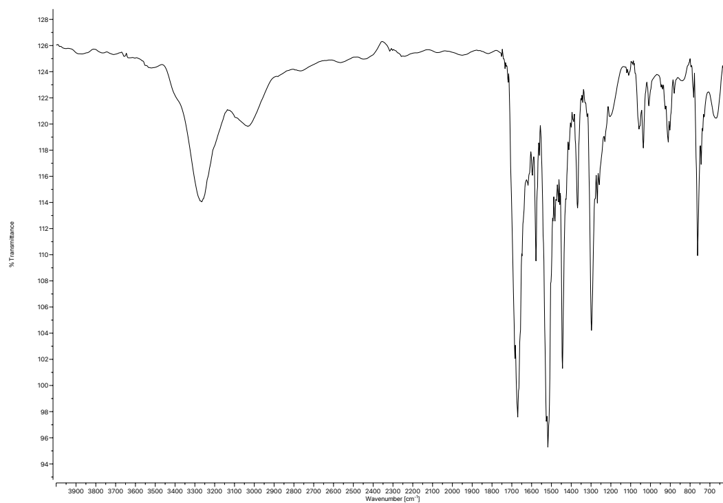
Figure A3.71 Infrared spectrum (Thin Film, NaCl) of compound 104 .
