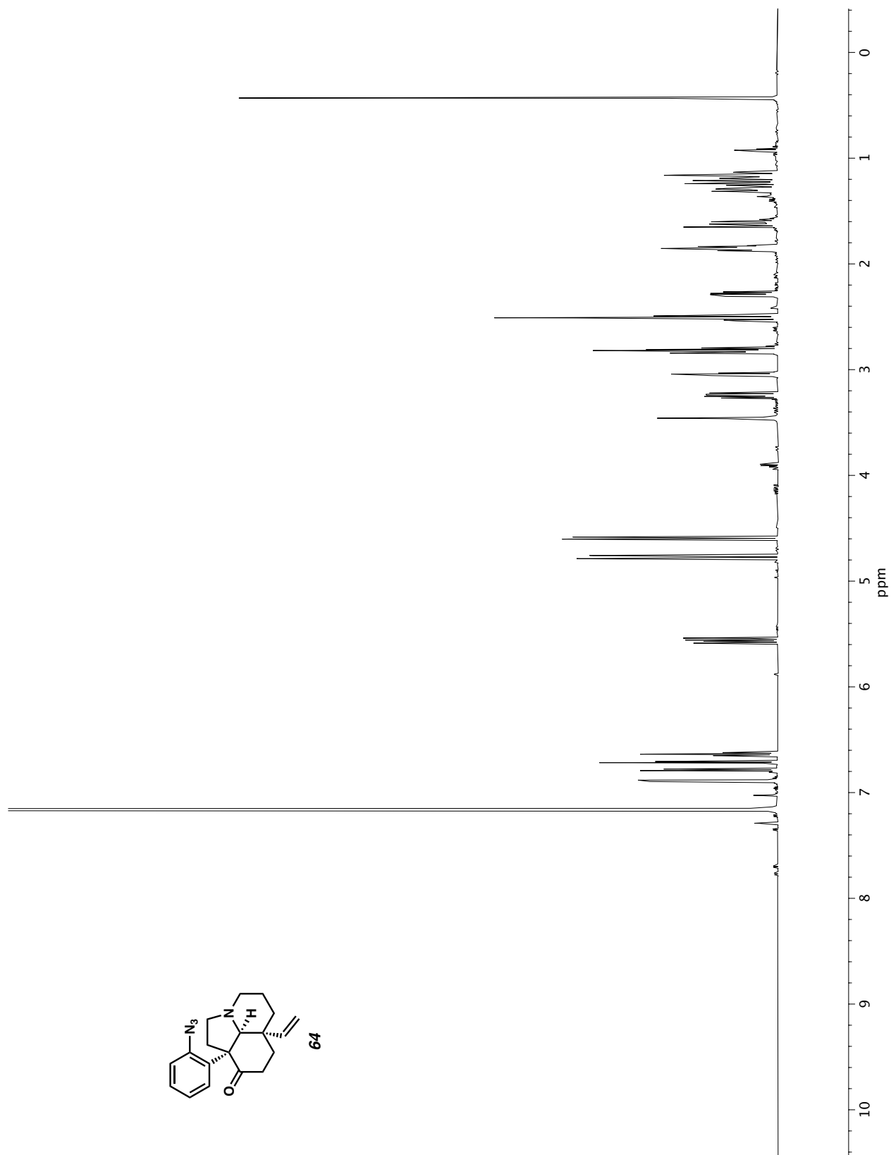
Figure A1.86 ^1H NMR (600 MHz, CDCl_3 ) of compound 64 .
