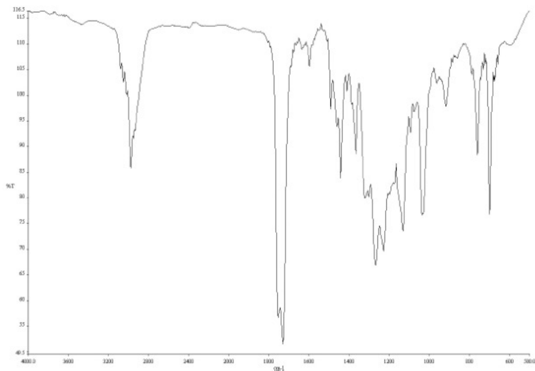
Figure A1.2 Infrared spectrum (Thin Film, NaCl) of compound 32a .
