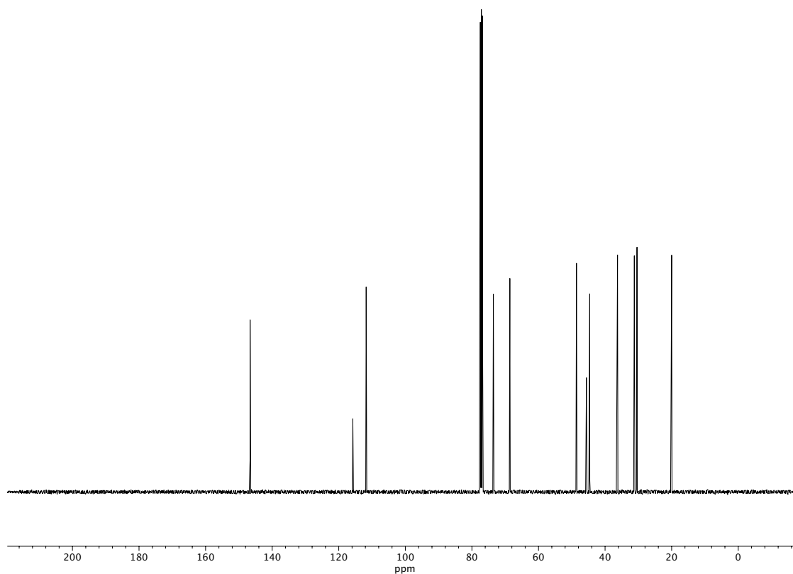
Figure A3.42 13 C NMR (100 MHz, CDCl 3 ) of compound 88 .
