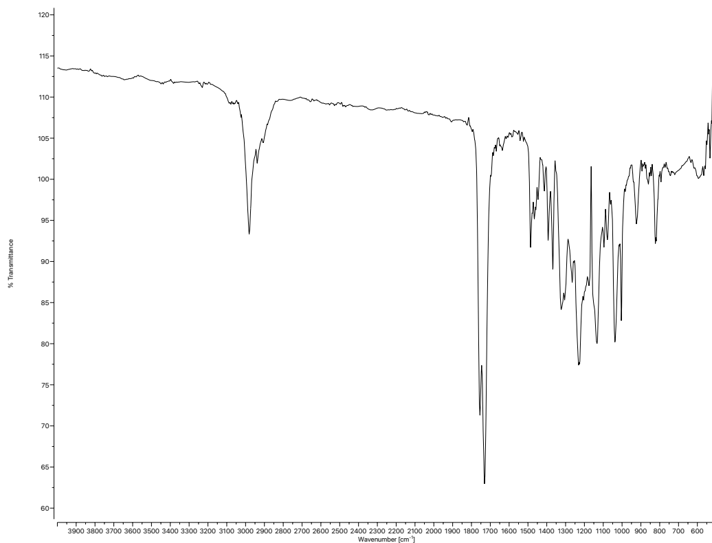
Figure A1.29 Infrared spectrum (Thin Film, NaCl) of compound 32g .
