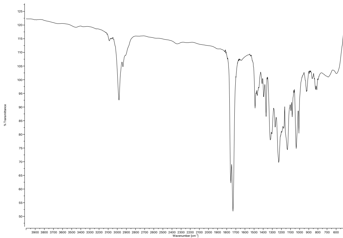
Figure A1.32 Infrared spectrum (Thin Film, NaCl) of compound 32h .
