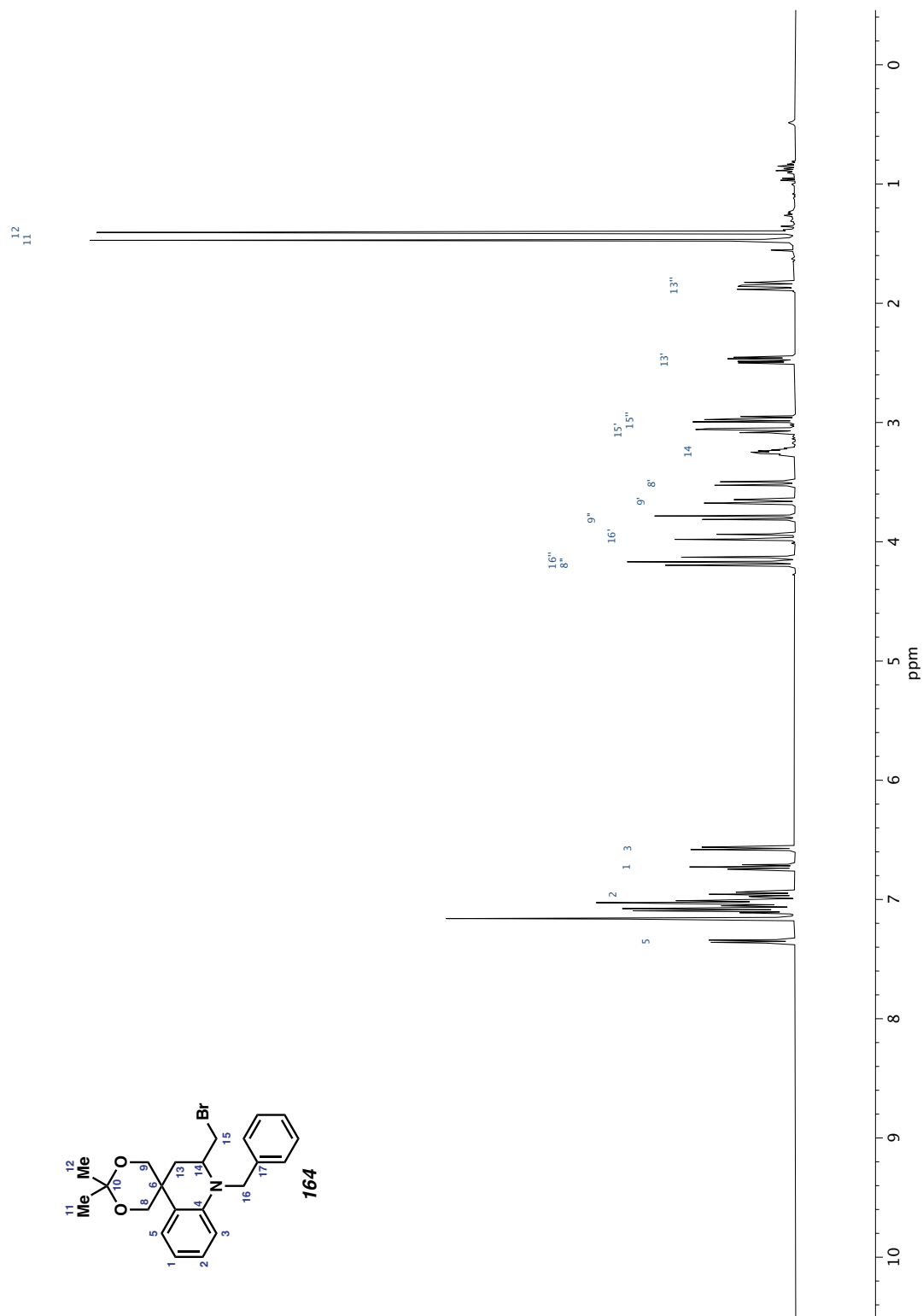
Figure A5.70 ^1\text{H} NMR (400 MHz, \text{C}_6\text{D}_6 ) of compound 164 .
