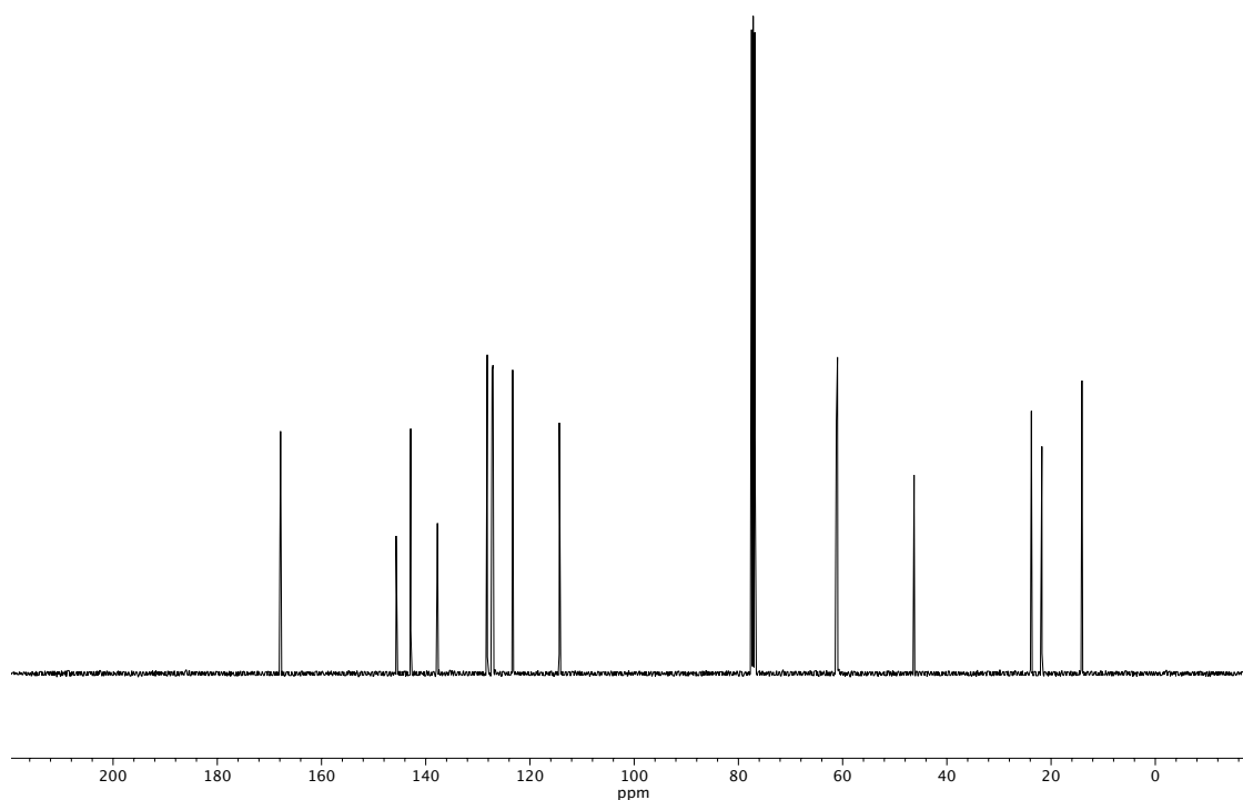
Figure A1.18 13 C NMR (100 MHz, CDCl 3 ) of compound 32c .
