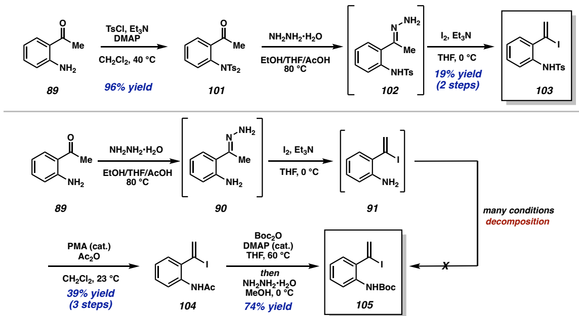
Scheme 2.4.9. Synthesis of dianion nucleophile precursors 103 and 105 .
