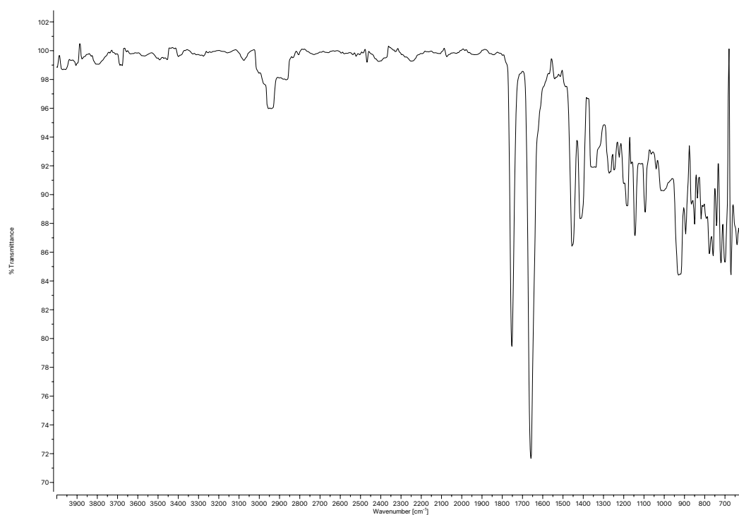
Figure A3.53 Infrared spectrum (Thin Film, NaCl) of compound 67d .
