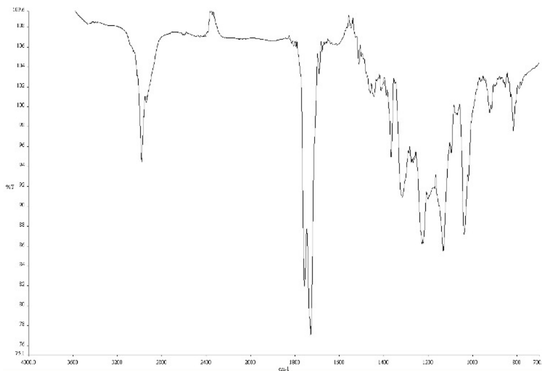
Figure A1.26 Infrared spectrum (Thin Film, NaCl) of compound 32f .
