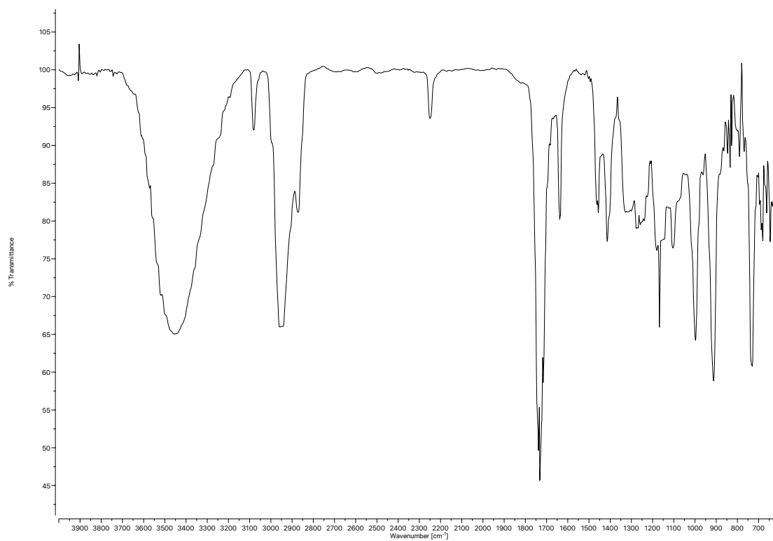
Figure A3.17 Infrared spectrum (Thin Film, NaCl) of compound 70 .
