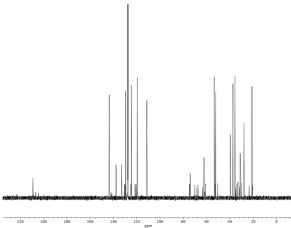
Figure A3.88 13 C NMR (125 MHz, C 6 D 6 ) of compound 64 .
