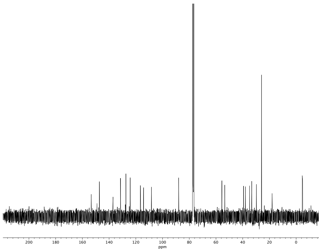
Figure A3.60 13 C NMR (100 MHz, CDCl 3 ) of compound 93 .
