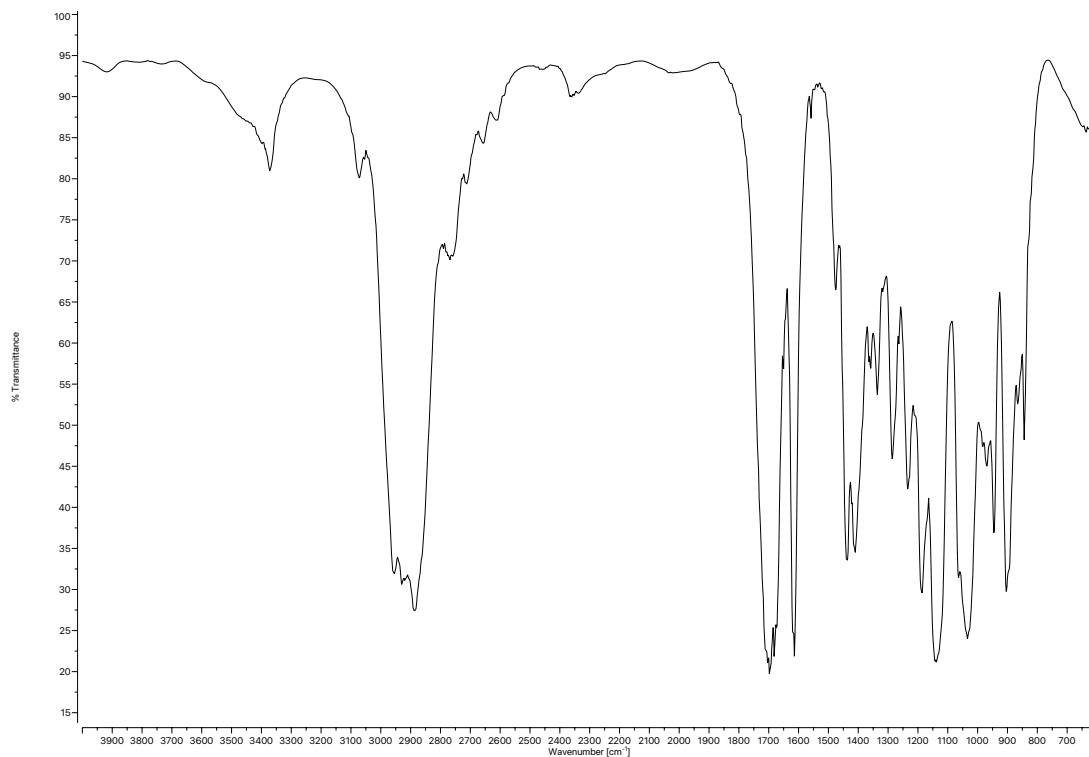
Figure A3.2 Infrared spectrum (Thin Film, NaCl) of compound 72 .
