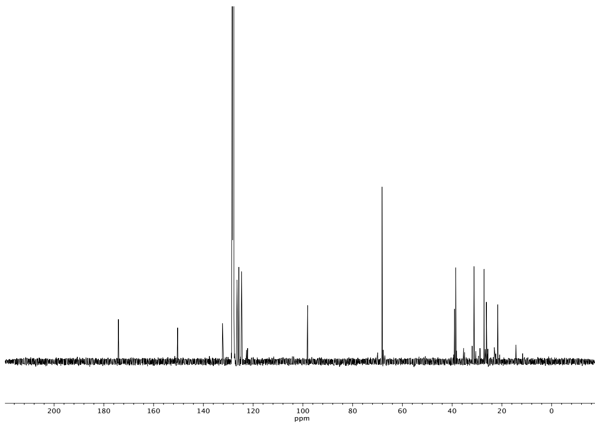
Figure A5.45 13 C NMR (100 MHz, C 6 D 6 ) of compound 166 .
