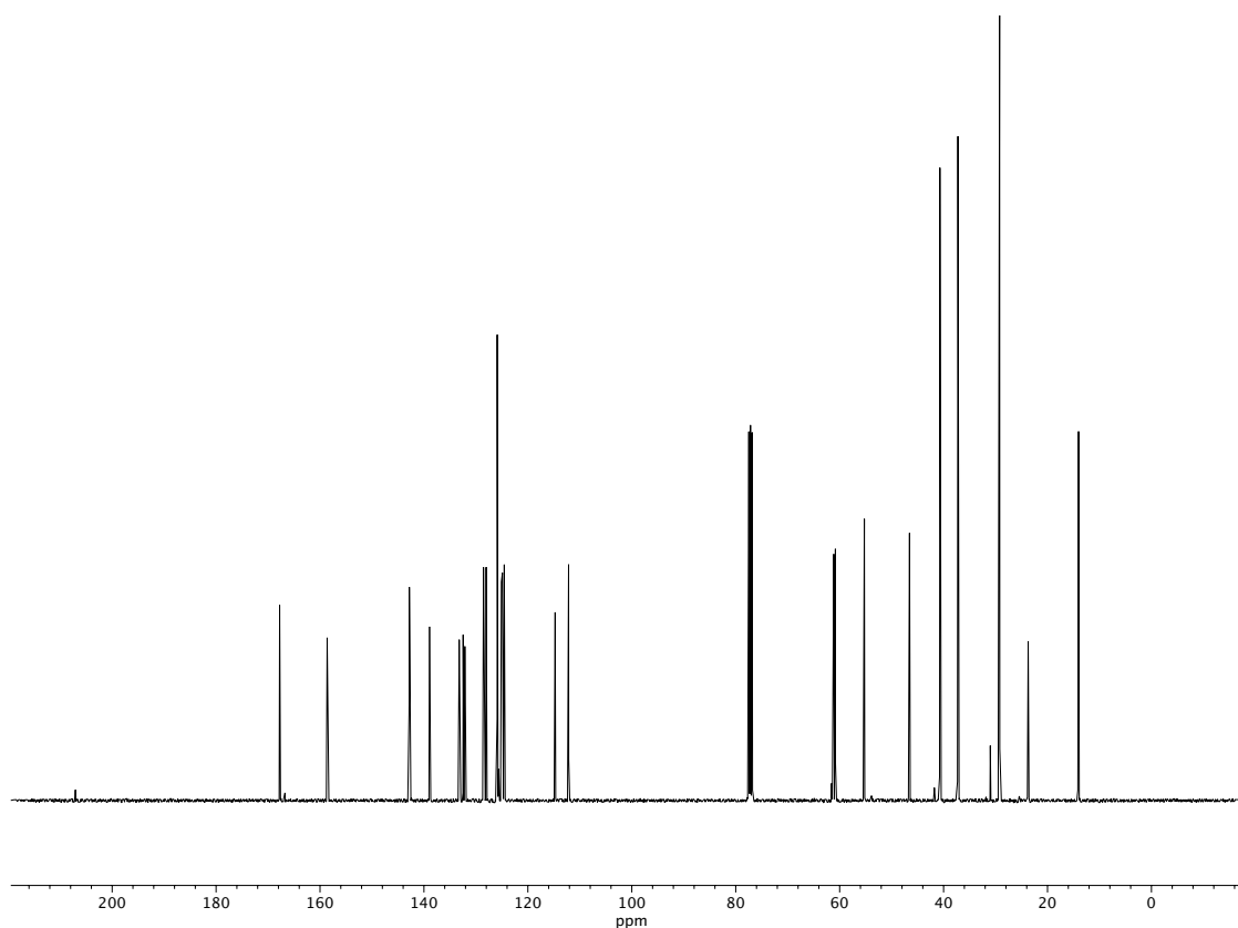
Figure A1.53 13 C NMR (100 MHz, CDCl 3 ) of compound 32n .
