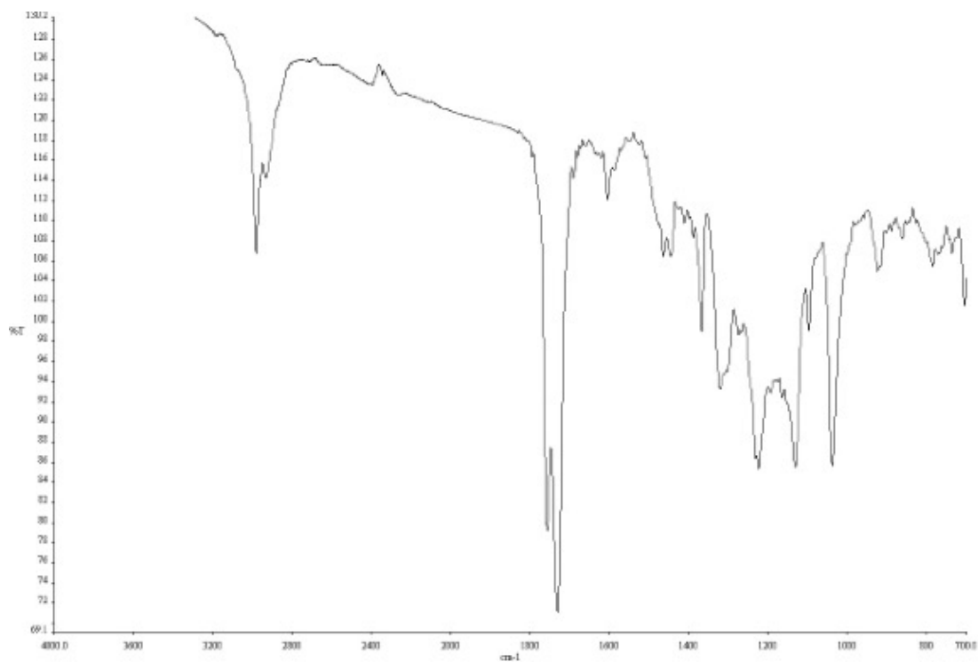
Figure A1.17 Infrared spectrum (Thin Film, NaCl) of compound 32c .
