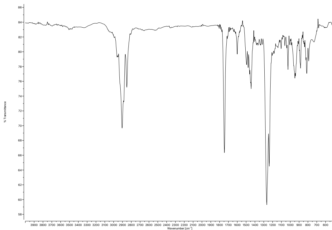
Figure A1.109 Infrared spectrum (Thin Film, NaCl) of compound 31n .
