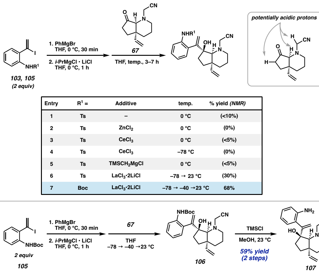
Scheme 2.4.10. Optimization of the dianion 1,2-addition.
