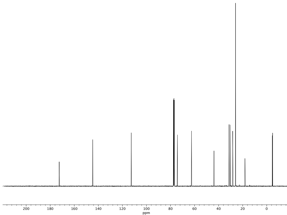
Figure A3.39 13 C NMR (100 MHz, CDCl 3 ) of compound 87 .
