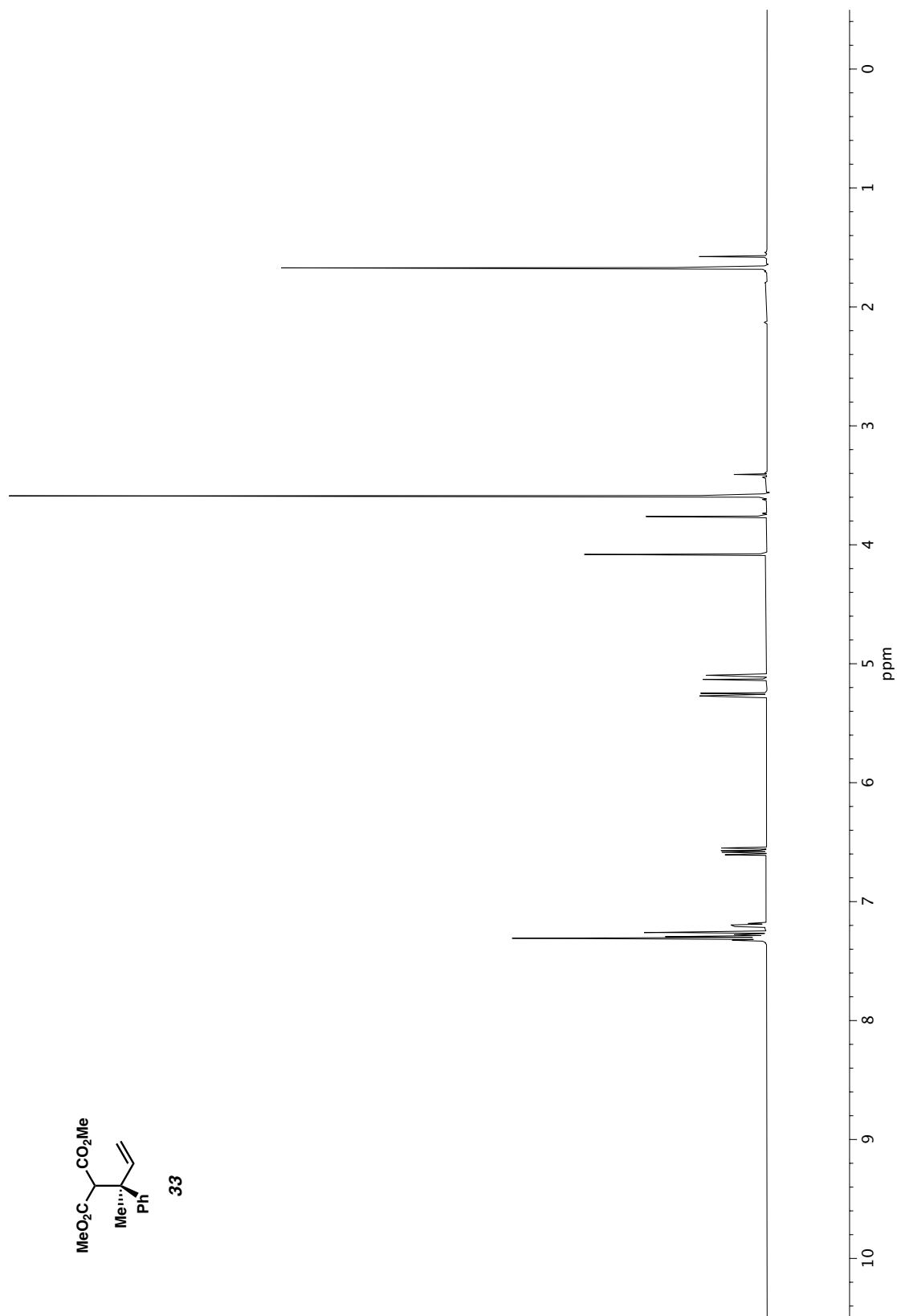
Figure A1.4 1 H NMR (500 MHz, CDCl 3 ) of compound 33 .
