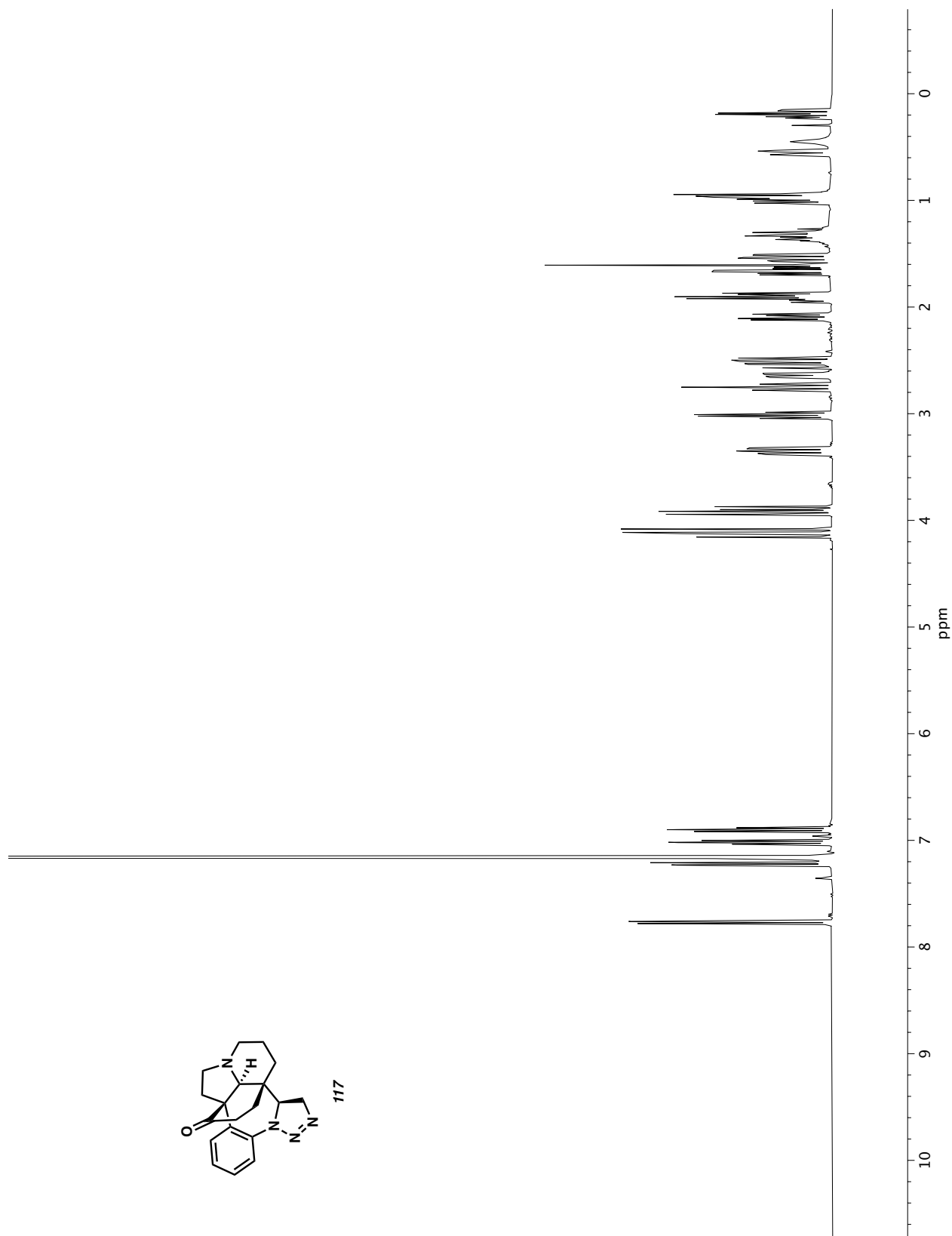
Figure A3.94 ^1\text{H} NMR (400 MHz, \text{C}_6\text{D}_6 ) of compound 117 .
