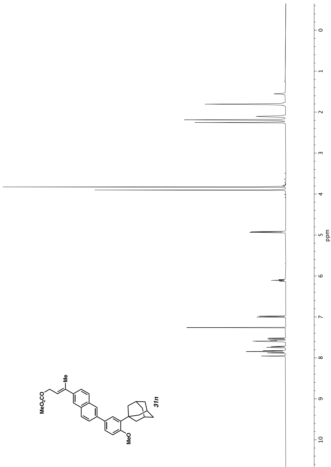
Figure A1.108 ^1\text{H} NMR (400 MHz, \text{CDCl}_3 ) of compound 31n .
