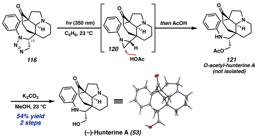
Scheme 2.4.15. Completion of the synthesis of hunterine A.
