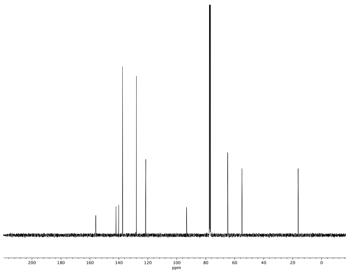
Figure A1.89 13 C NMR (100 MHz, CDCl 3 ) of compound 31g .
