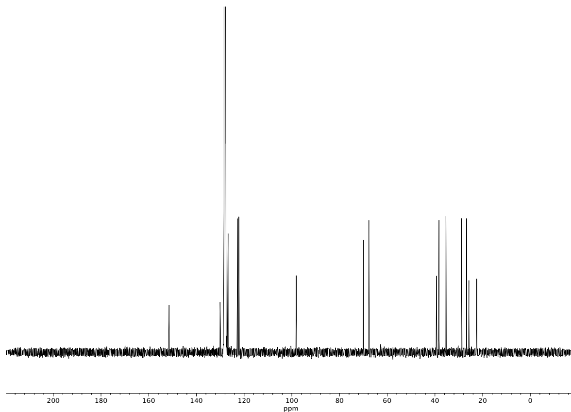
Figure A5.36 13 C NMR (100 MHz, C 6 D 6 ) of compound 158 .
