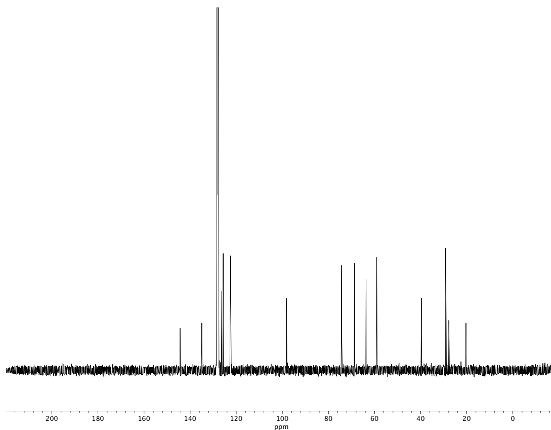
Figure A5.30 13 C NMR (100 MHz, C 6 D 6 ) of compound 156 .
