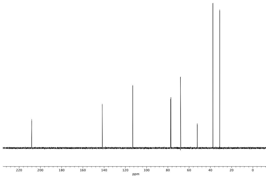
Figure A3.15 13 C NMR (125 MHz, CDCl 3 ) of compound 68 .
