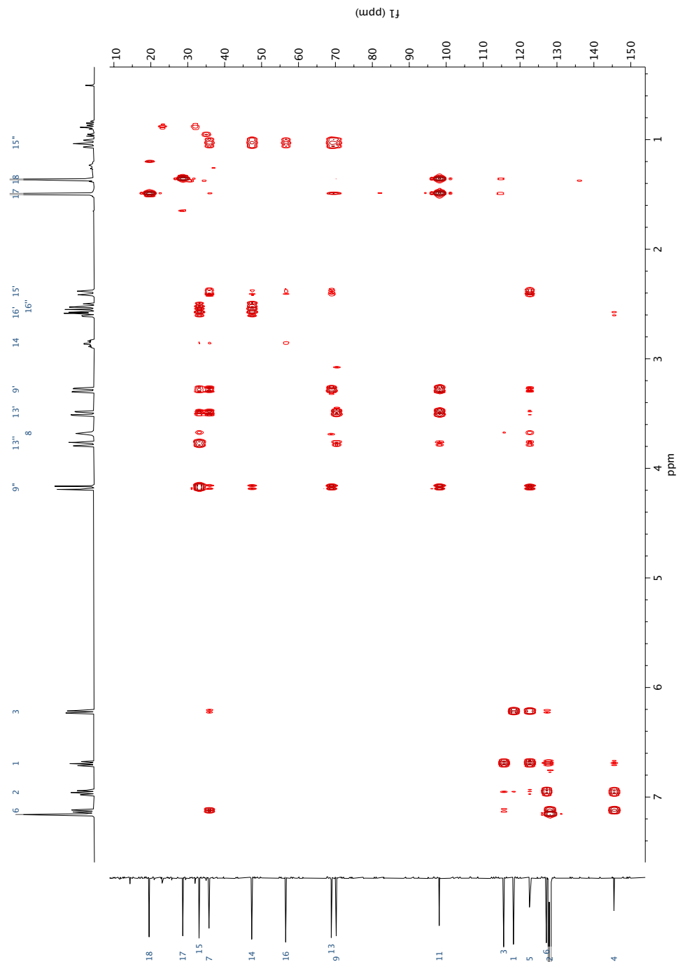
Figure A.69 HMBC spectrum ( C_6D_6 ) of compound 163 .
