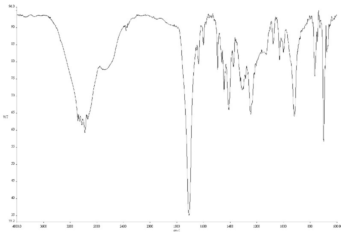
Figure A1.70 Infrared spectrum (Thin Film, NaCl) of compound 40 .
