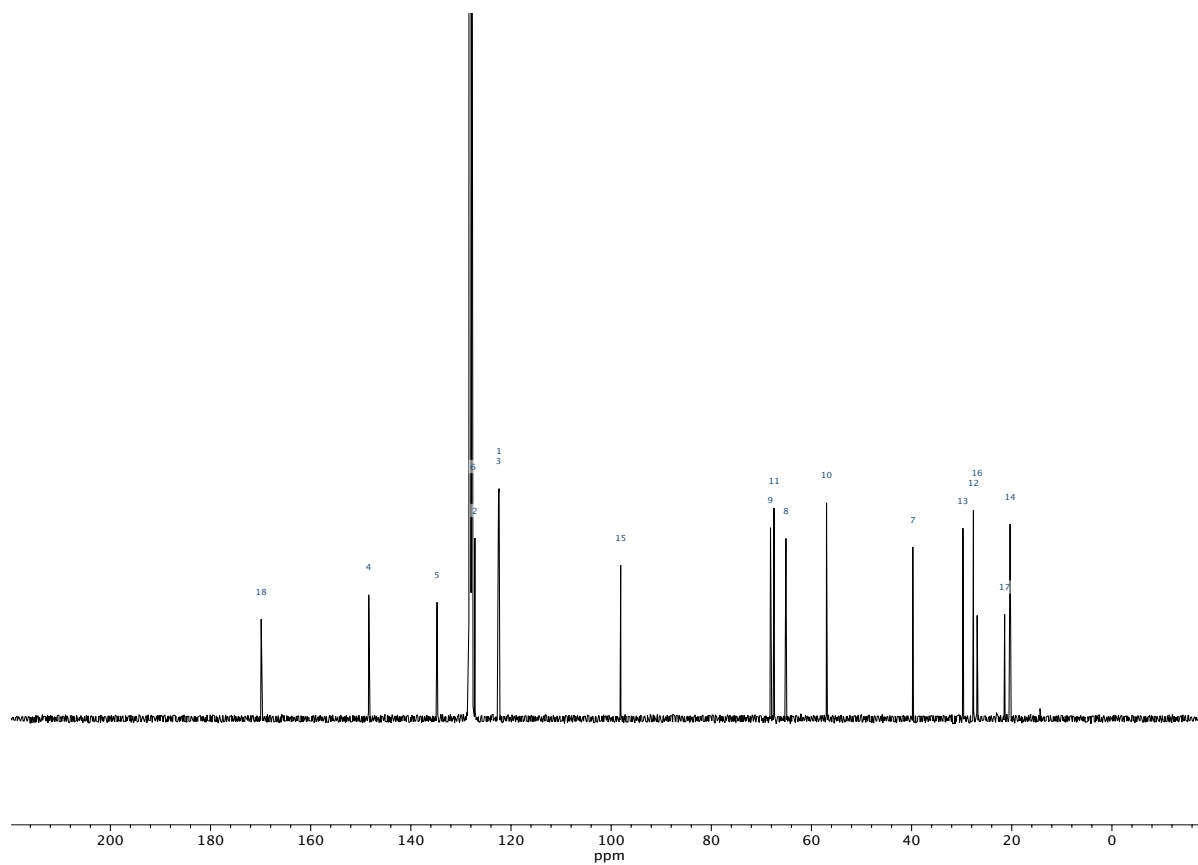
Figure A.39 13 C NMR (100 MHz, C 6 D 6 ) of compound 159 .
