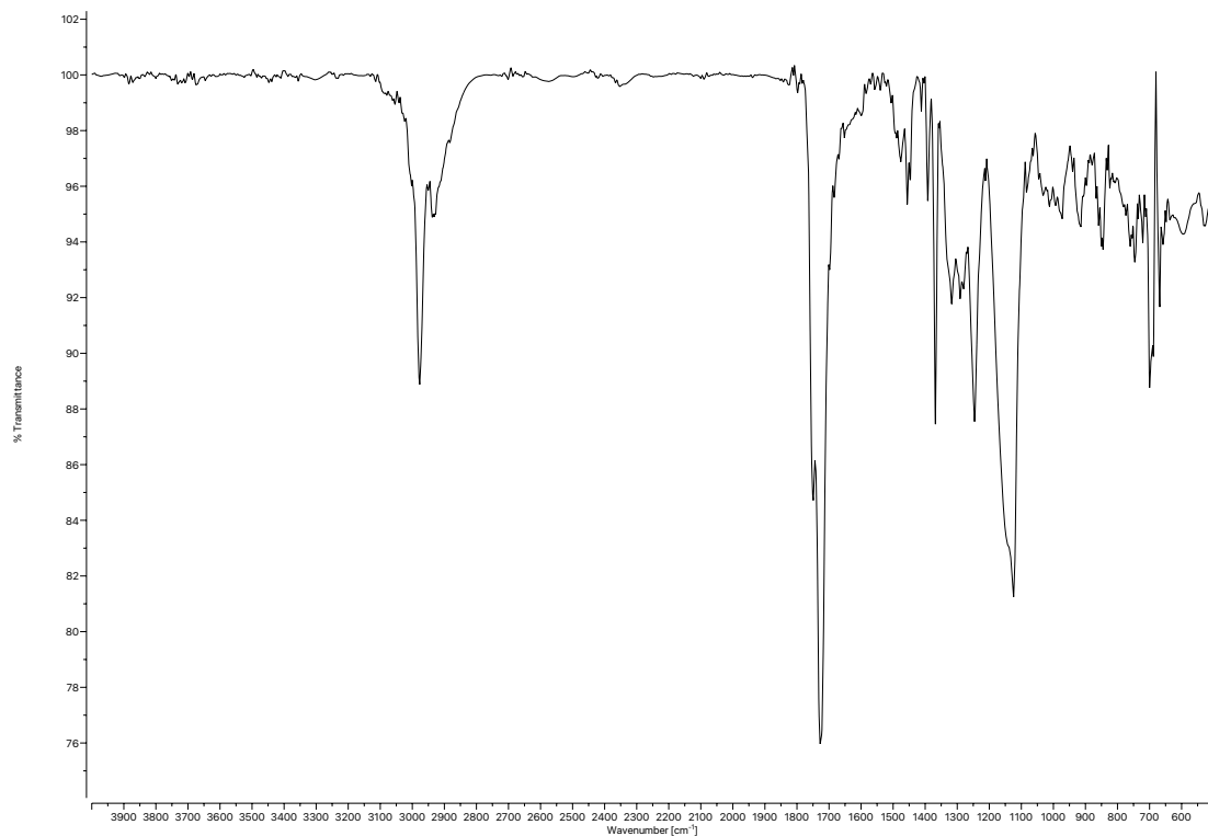
Figure A1.8 Infrared spectrum (Thin Film, NaCl) of compound 34 .
