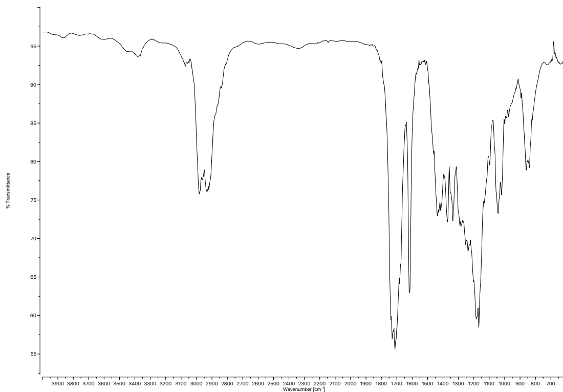
Figure A3.8 Infrared spectrum (Thin Film, NaCl) of compound 76 .
