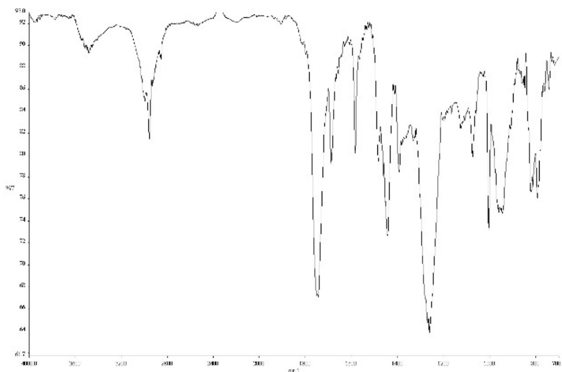
Figure A1.88 Infrared spectrum (Thin Film, NaCl) of compound 31g .
