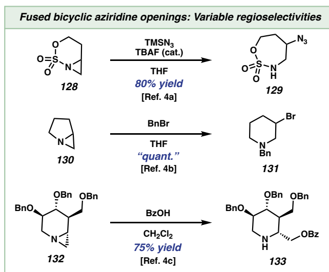
Scheme 3.1.1 Ring opening reactions of fused bicyclic aziridines
