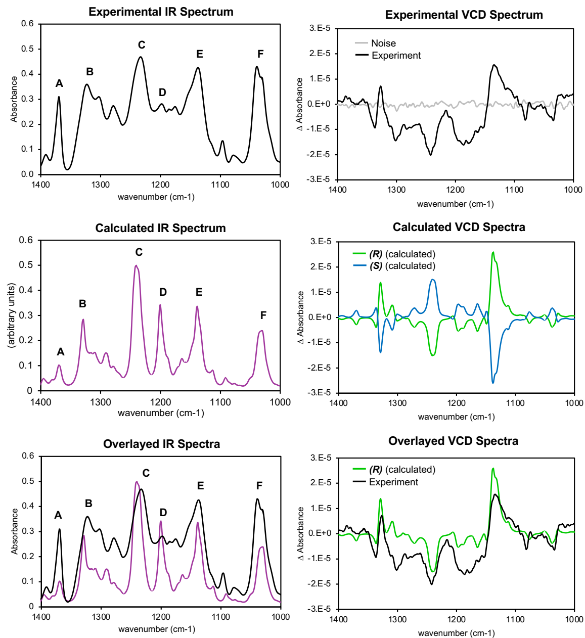
Figure 1.11.3.1. Experimental and computationally determined IR, VCD spectra of 32a and overlayed experimentally and computationally determined IR, VCD spectra of 32a .
