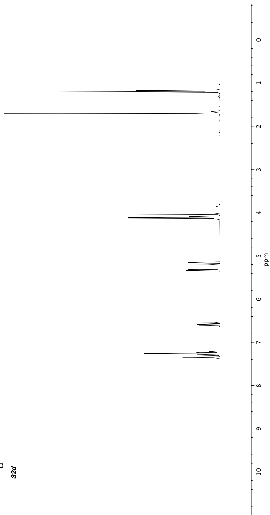
Figure A1.19 1 H NMR (400 MHz, CDCl 3 ) of compound 32d .
