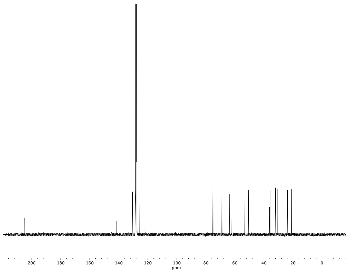
Figure A3.96 13 C NMR (100 MHz, C 6 D 6 ) of compound 117 .
