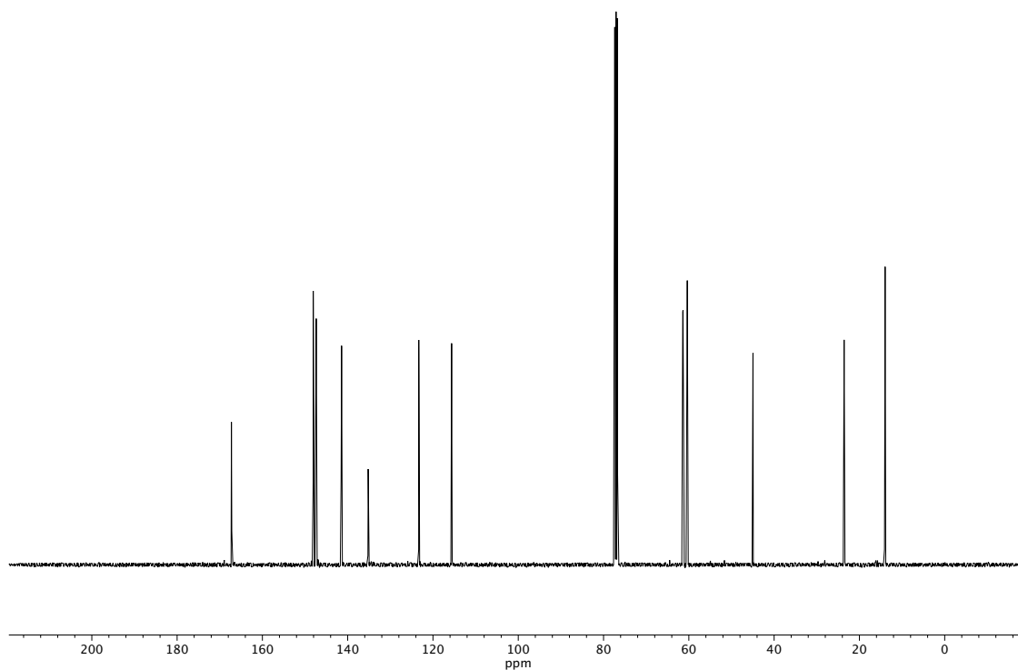
Figure A1.59 13 C NMR (100 MHz, CDCl 3 ) of compound 32q .
