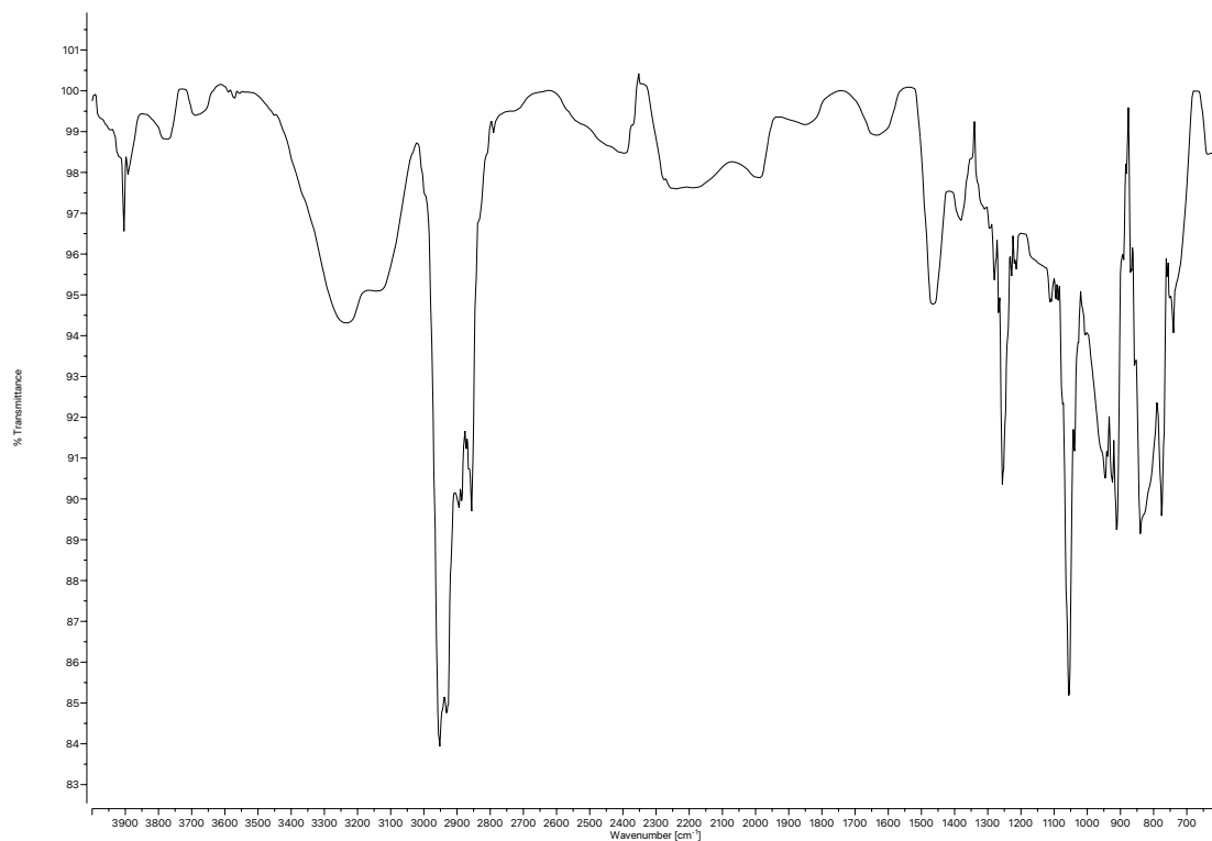
Figure A3.32 Infrared spectrum (Thin Film, NaCl) of compound (Z)-86.
