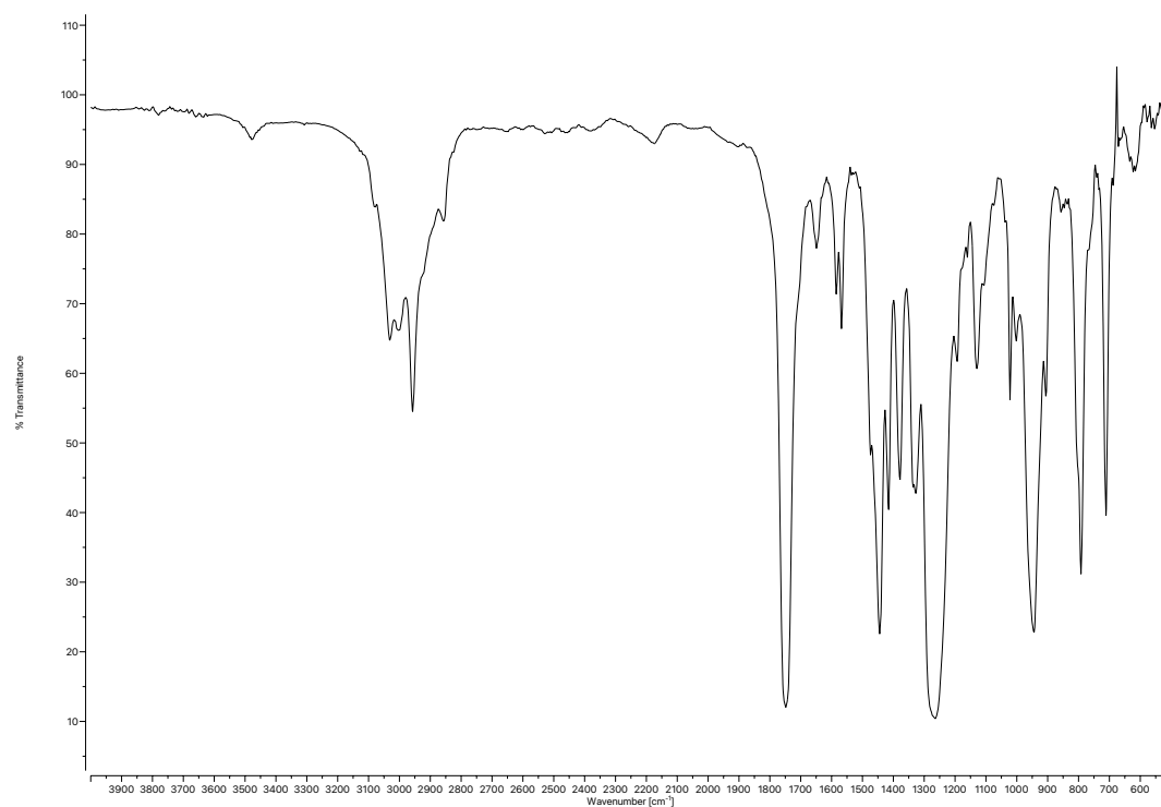
Figure A1.115 Infrared spectrum (Thin Film, NaCl) of compound 31q .
