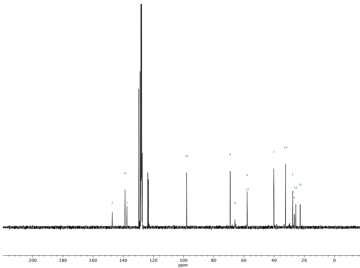
Figure A.54 13 C NMR (100 MHz, C 6 D 6 ) of compound 161 .
