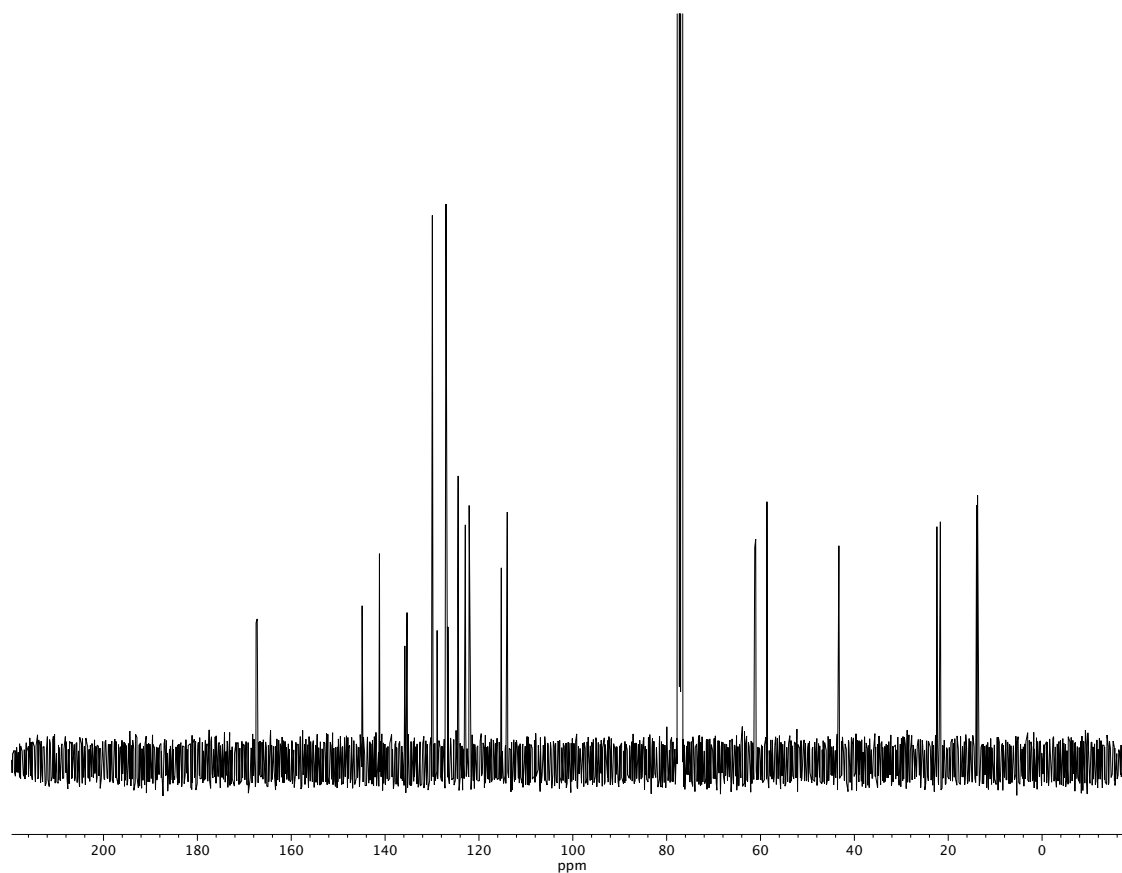
Figure A1.56 13 C NMR (100 MHz, CDCl 3 ) of compound 32p .
