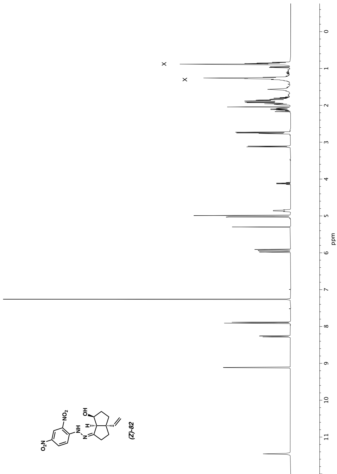
Figure A3.25 ^1\text{H} NMR (400 MHz, \text{CDCl}_3 ) of compound (Z)-82.
