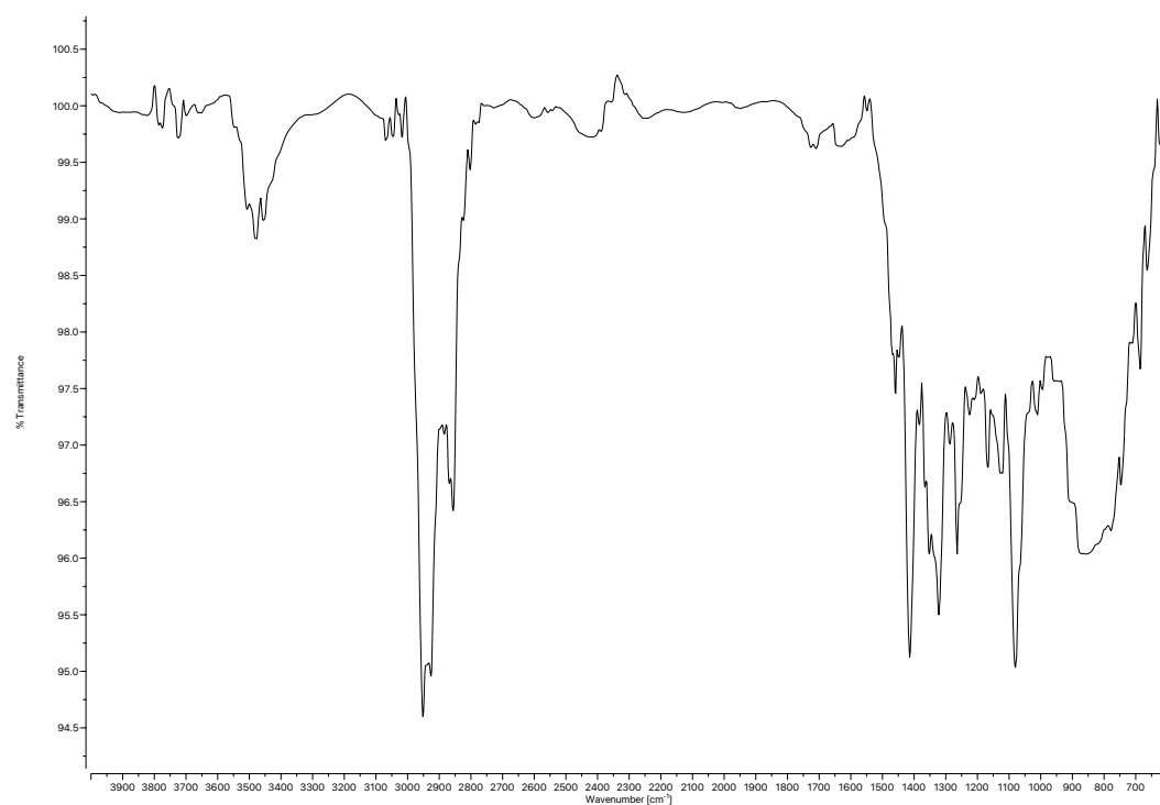
Figure A3.59 Infrared spectrum (Thin Film, NaCl) of compound 93 .
