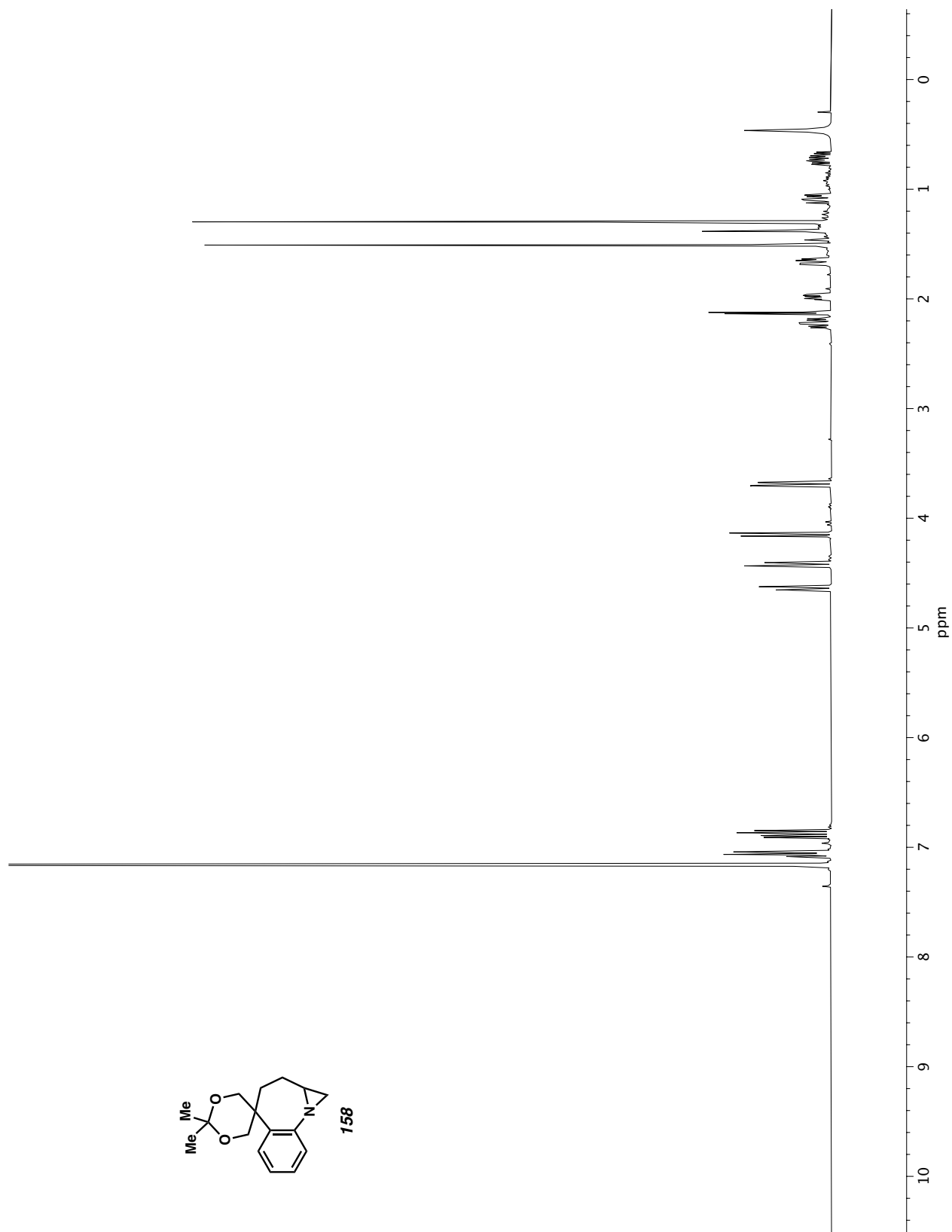
Figure A5.34 ^1\text{H} NMR (400 MHz, \text{C}_6\text{D}_6 ) of compound 158 .
