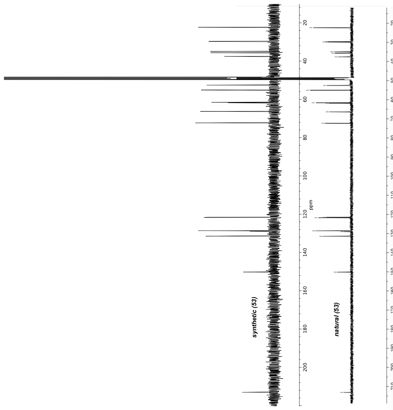
Figure A3.102 Overlaid ^{13}\text{C} (100 MHz, \text{CD}_3\text{OD} ) of synthetic and natural 53.
