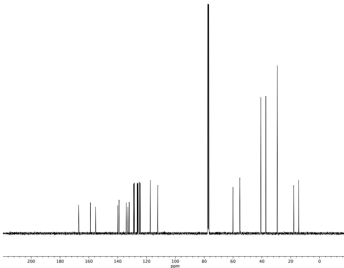
Figure A1.107 13 C NMR (100 MHz, CDCl 3 ) of compound 47n .
