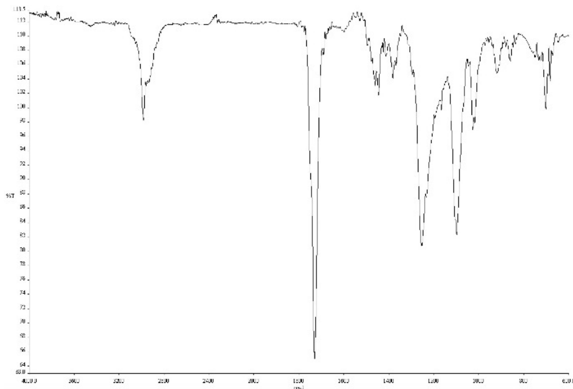
Figure A1.76 Infrared spectrum (Thin Film, NaCl) of compound 42 .
