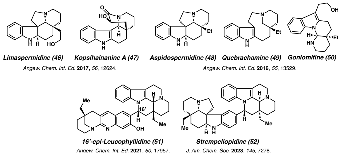
Figure 2.1.2 MIAs and monoterpene bisindole alkaloids synthesized by the Stoltz laboratory.
