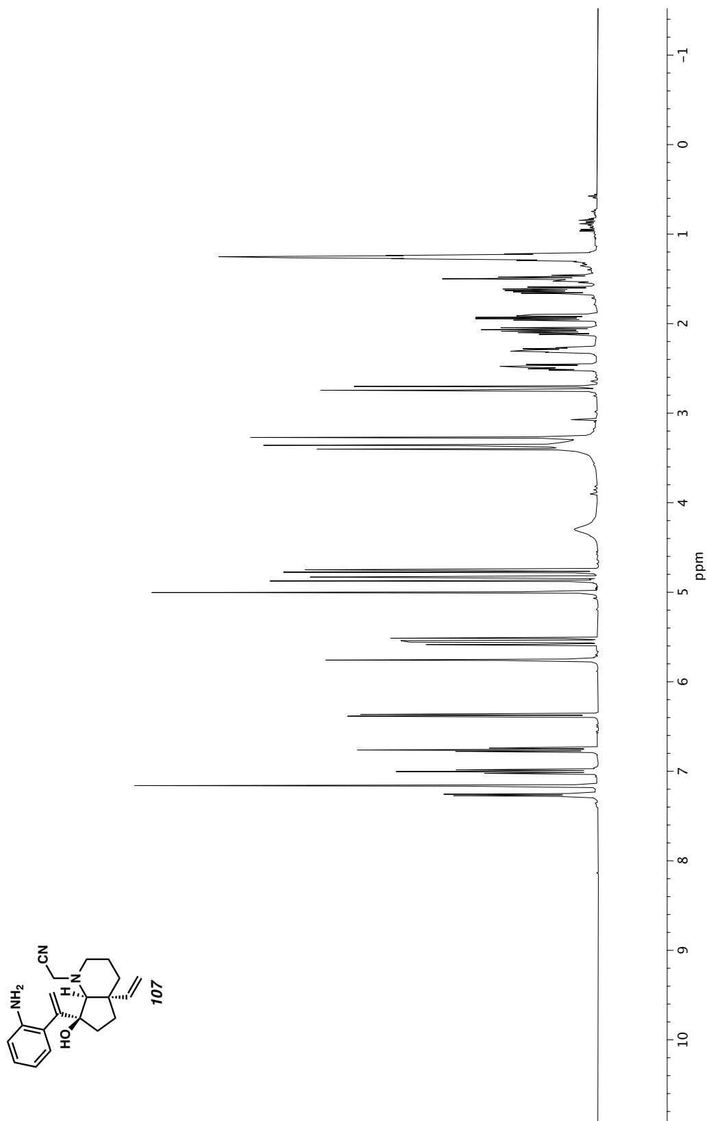
Figure A3.79 ^1\text{H} NMR (400 MHz, \text{C}_6\text{D}_6 ) of compound 107 .
