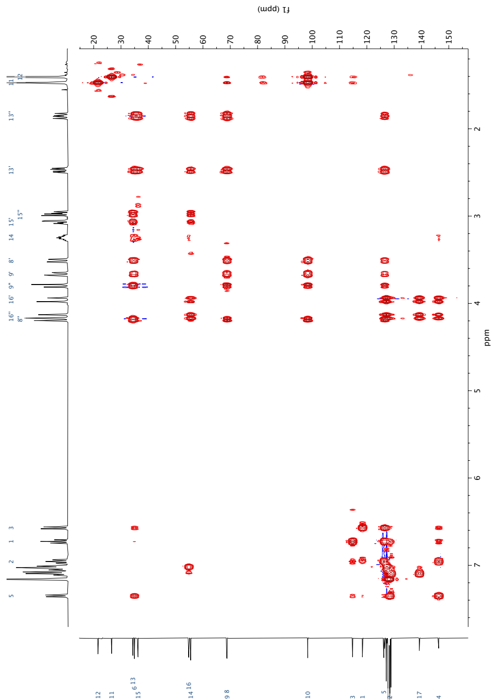
Figure A.75 HMBC spectrum ( C_6D_6 ) of compound 164 .
