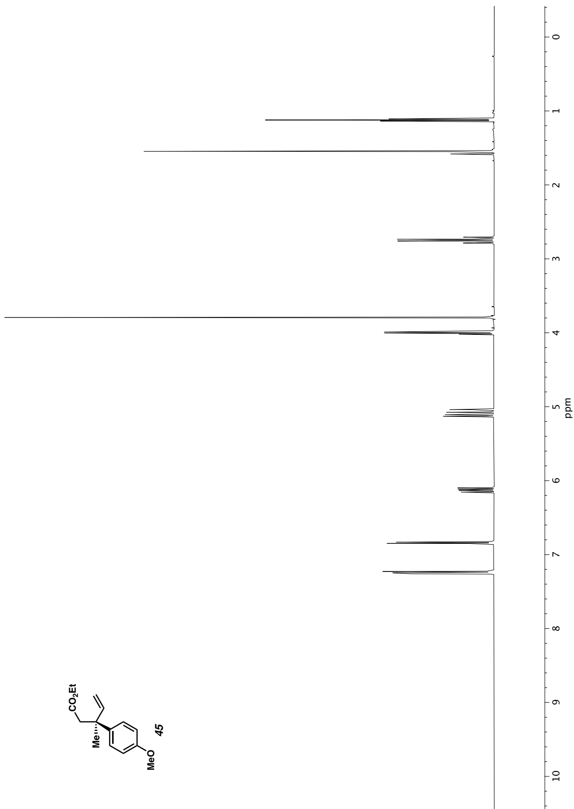
Figure A1.84 1 H NMR (500 MHz, CDCl 3 ) of compound 45 .
