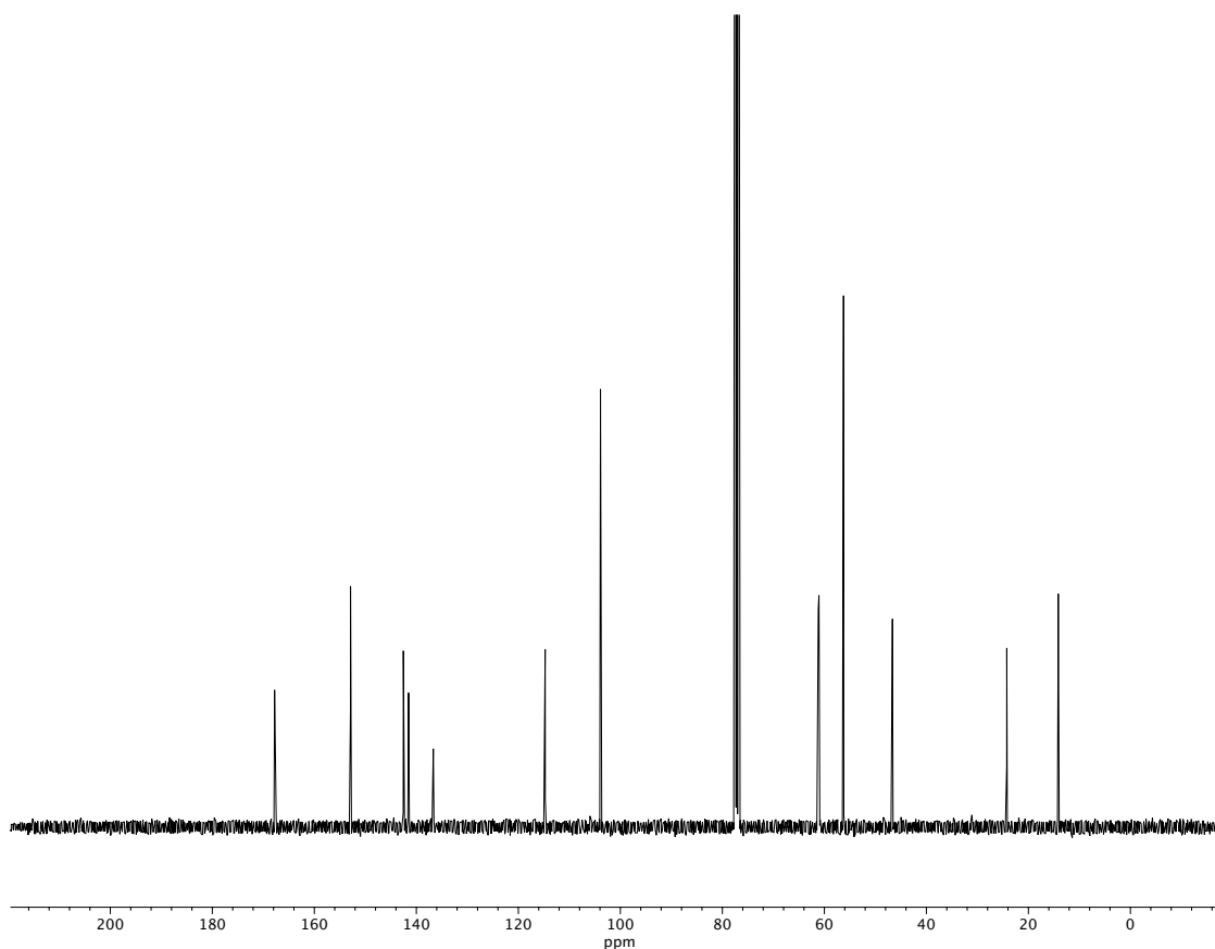
Figure A1.50 13 C NMR (100 MHz, CDCl 3 ) of compound 32m .
