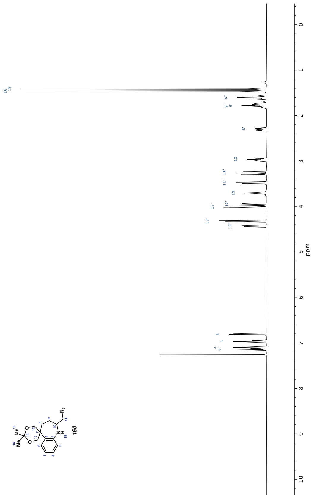
Figure A5.46 1 H NMR (400 MHz, CDCl 3 ) of compound 160 .
