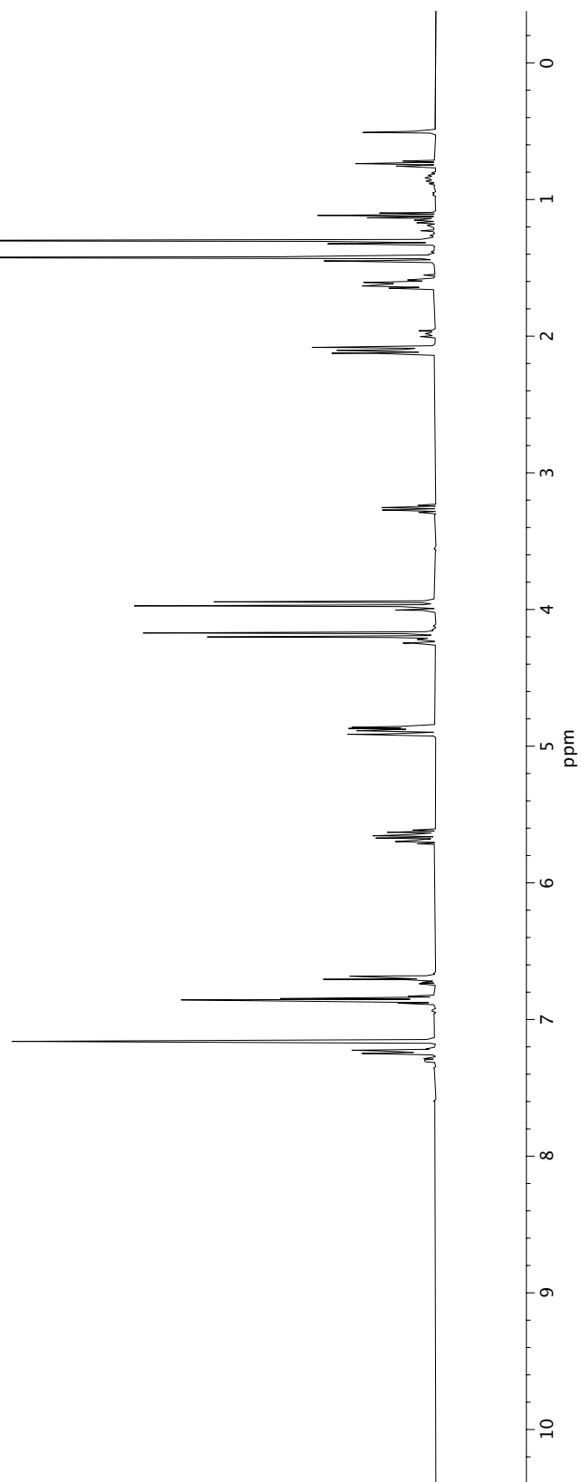
Figure A5.25 ^1\text{H} NMR (400 MHz, \text{C}_6\text{D}_6 ) of compound 154 .
