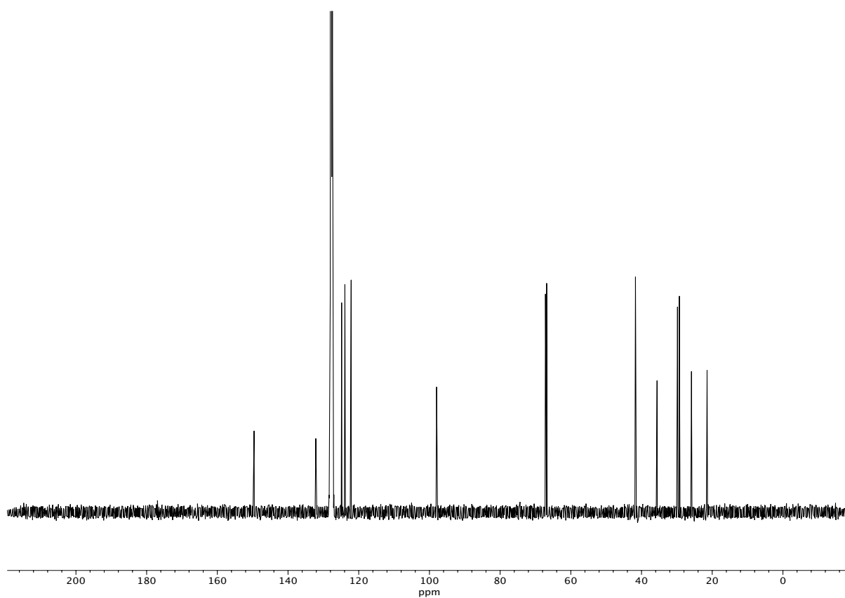
Figure A5.33 13 C NMR (100 MHz, C 6 D 6 ) of compound 157 .
