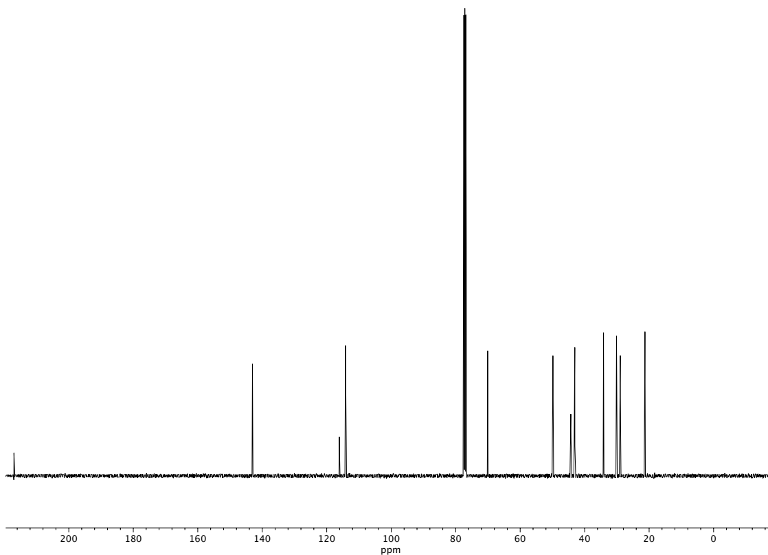
Figure A3.45 13 C NMR (100 MHz, CDCl 3 ) of compound 67 .
