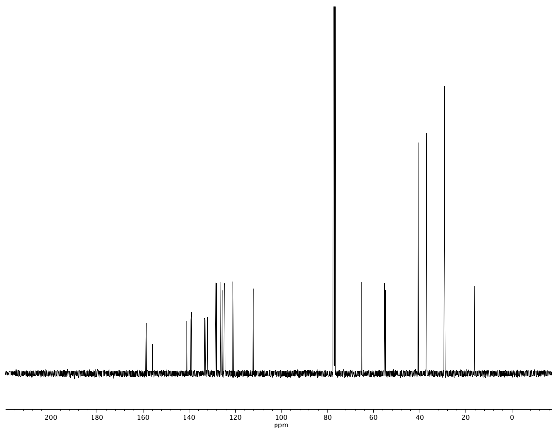
Figure A1.110 13 C NMR (100 MHz, CDCl 3 ) of compound 31n .
