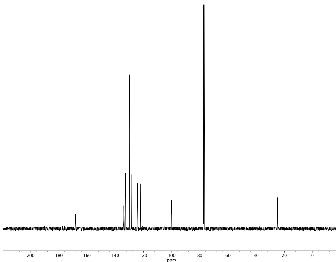
Figure A3.72 13 C NMR (100 MHz, CDCl 3 ) of compound 104 .
