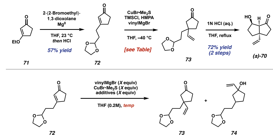
Scheme 2.4.1. Construction of racemic keto alcohol 70 and optimization of the 1,4-addition.
