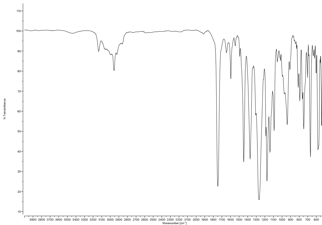
Figure A1.112 Infrared spectrum (Thin Film, NaCl) of compound 31p .
