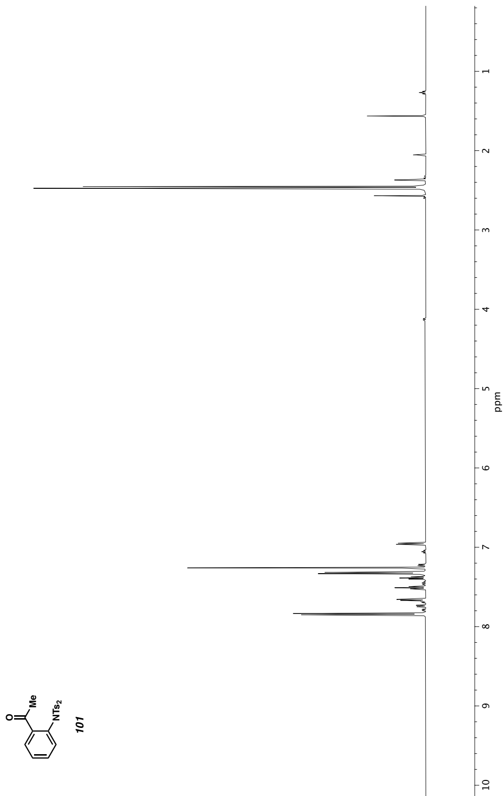
Figure A3.64 1 H NMR (500 MHz, CDCl 3 ) of compound 101 .
