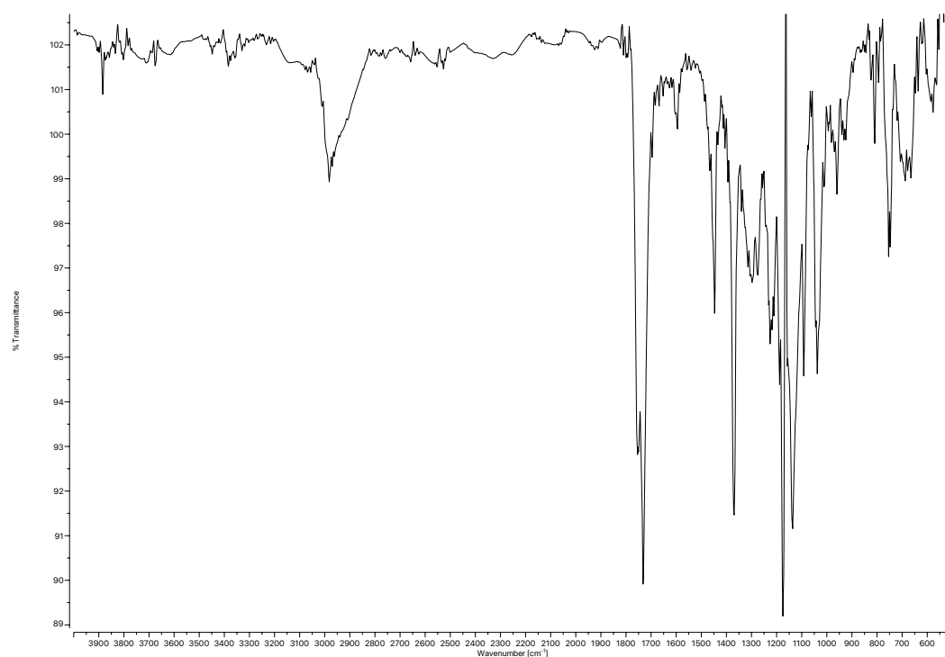
Figure A1.55 Infrared spectrum (Thin Film, NaCl) of compound 32p .
