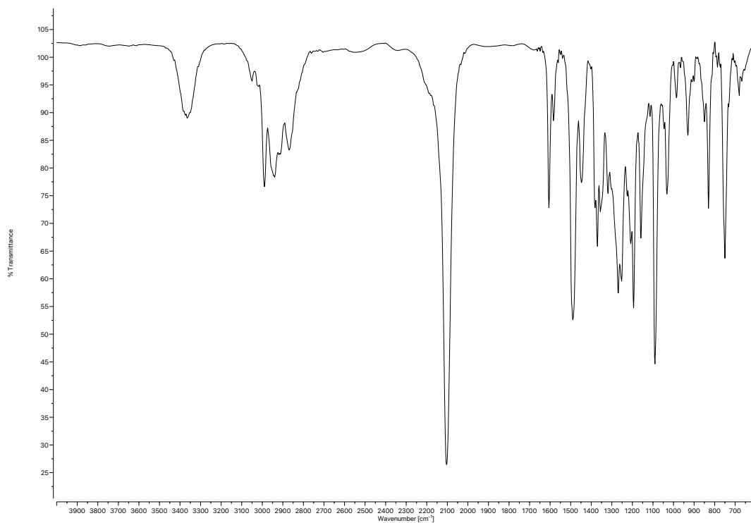
Figure A.65 Infrared spectrum (Thin Film, NaCl) of compound 163 .
