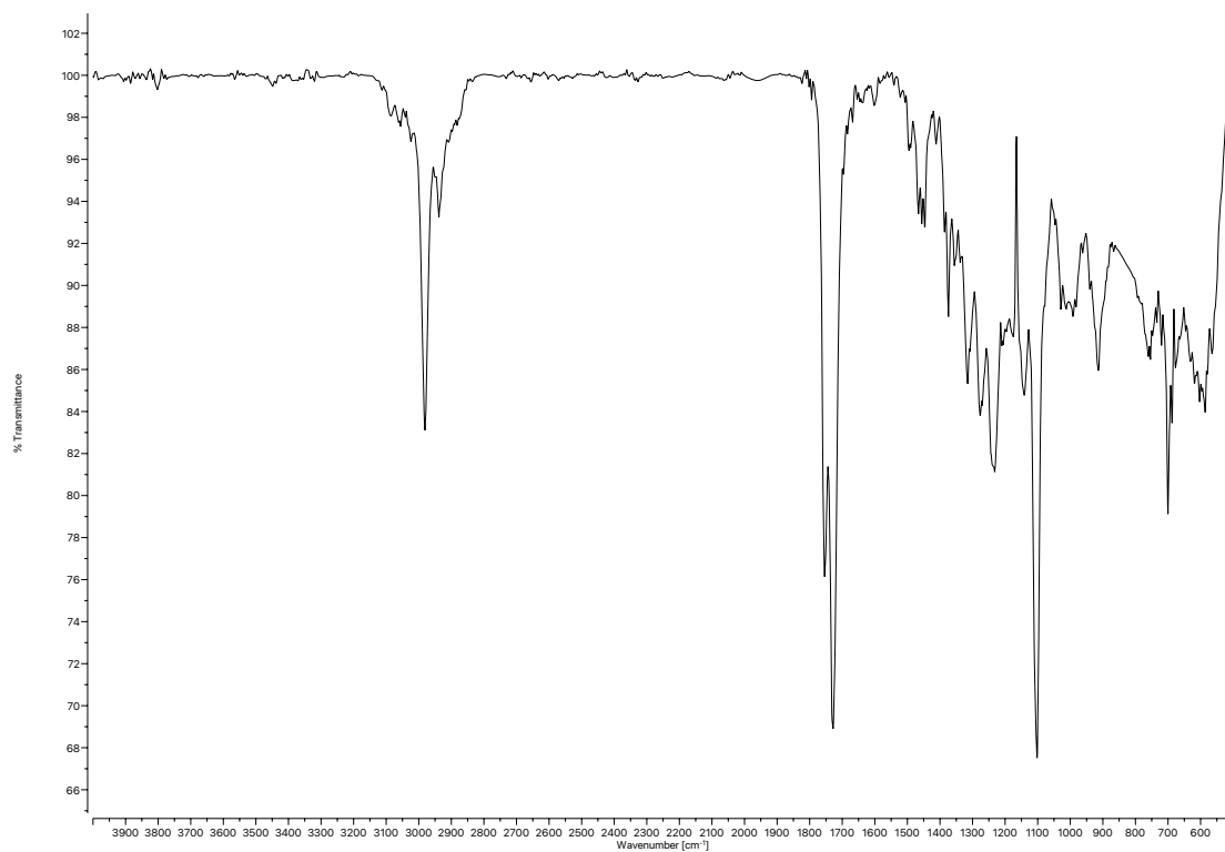
Figure A1.11 Infrared spectrum (Thin Film, NaCl) of compound 35 .
