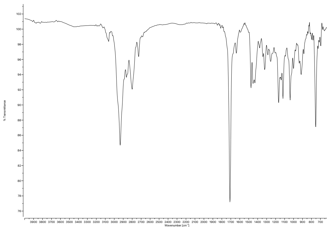
Figure A3.62 Infrared spectrum (Thin Film, NaCl) of compound 97 .
