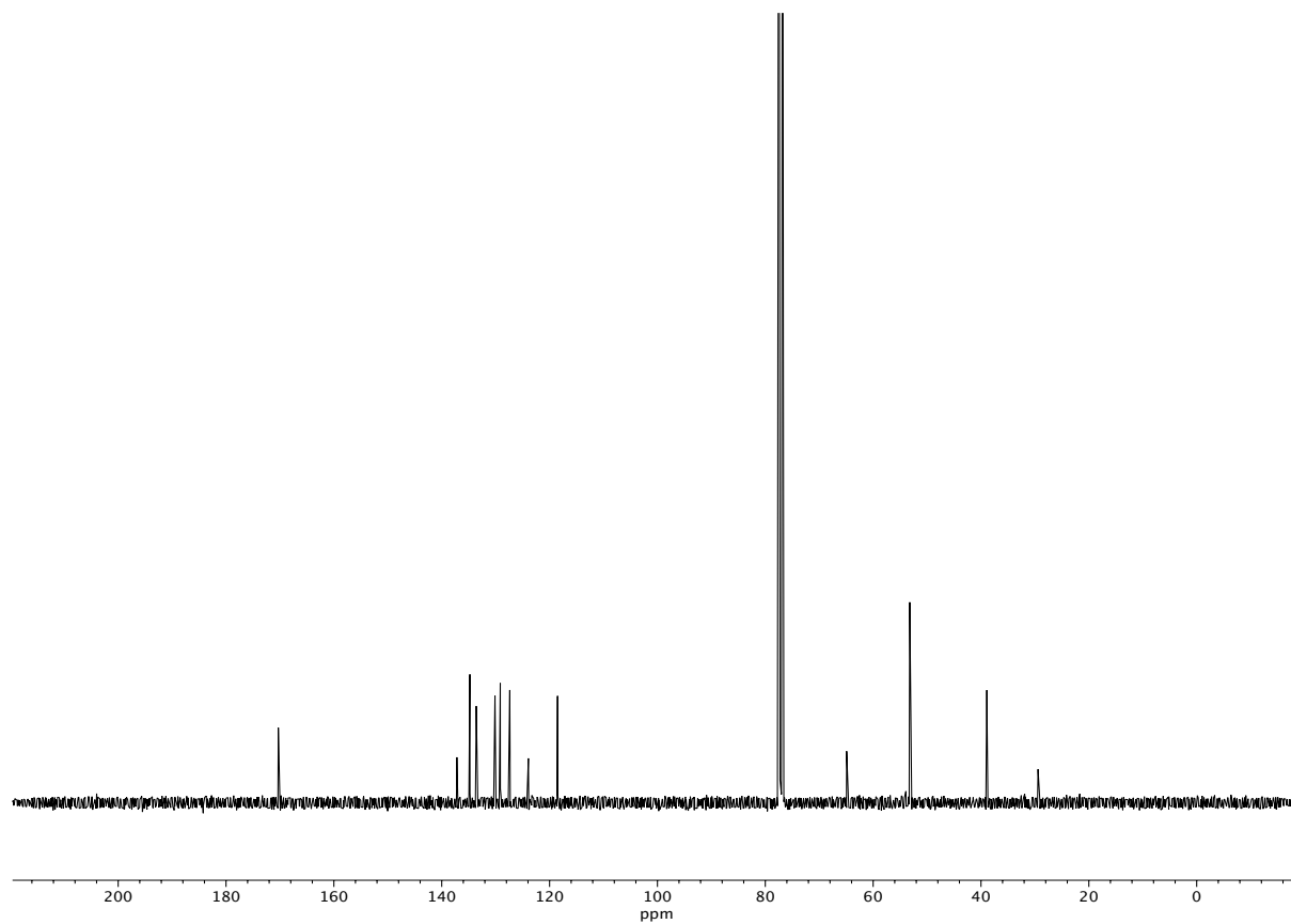
Figure A5.4 13 C NMR (100 MHz, CDCl 3 ) of compound 145 .
