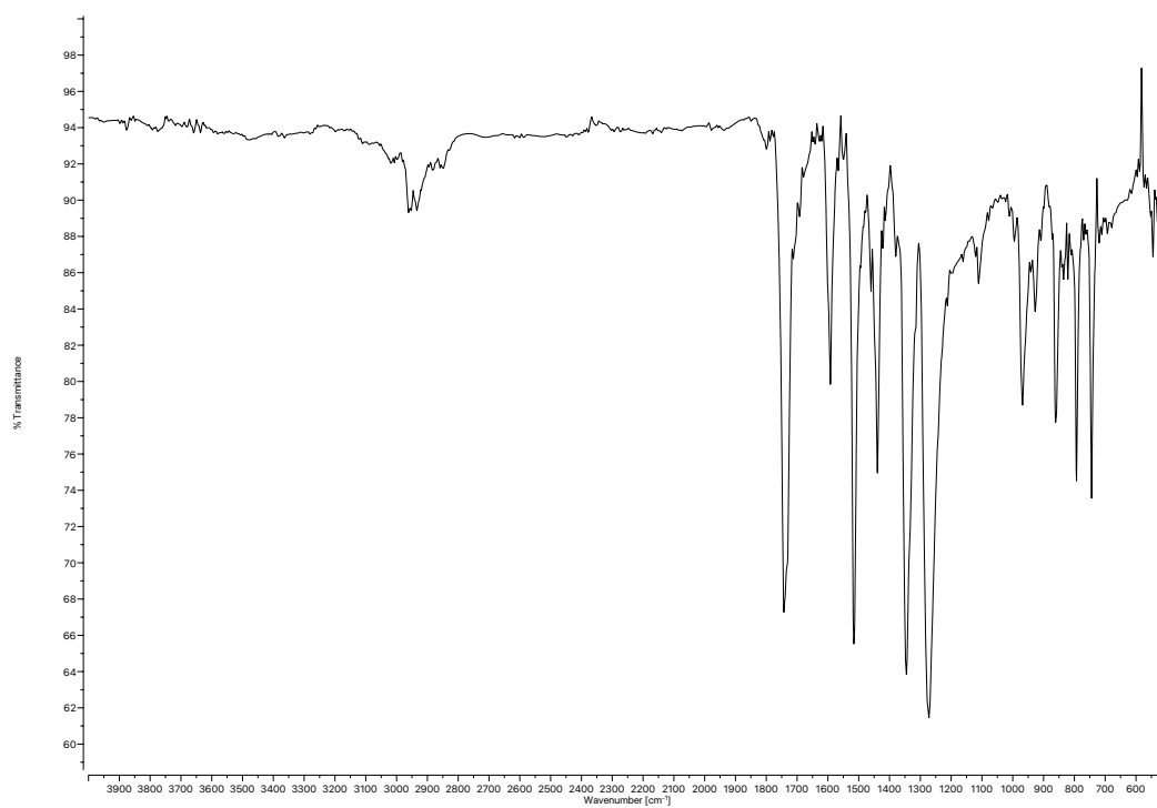
Figure A1.94 Infrared spectrum (Thin Film, NaCl) of compound 31k .
