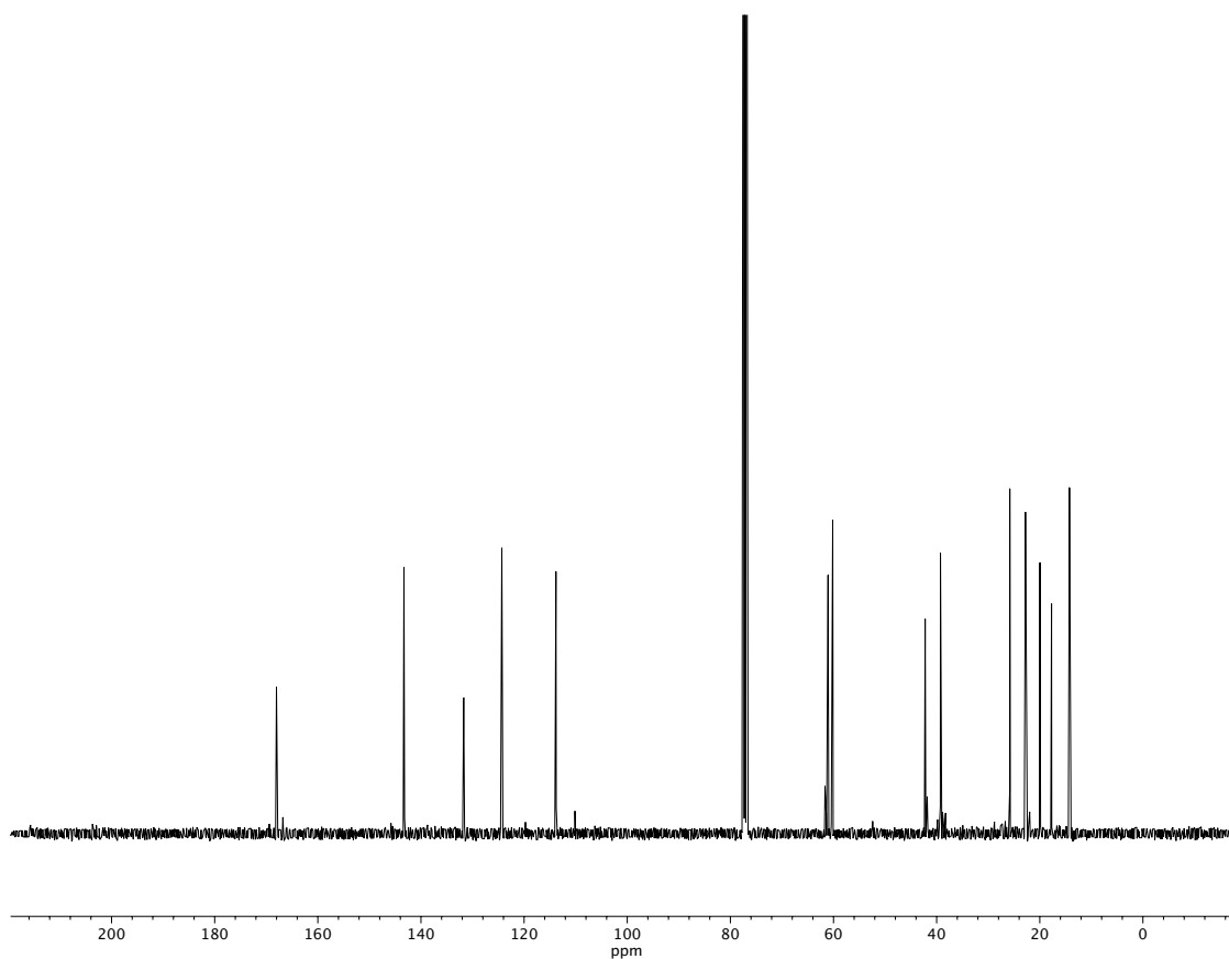
Figure A1.68 13 C NMR (100 MHz, CDCl 3 ) of compound 32u .
