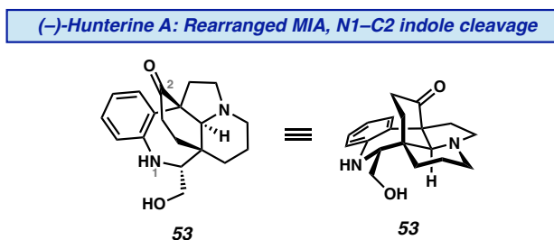
Figure 2.1.3. Structure of Hunterine A.
