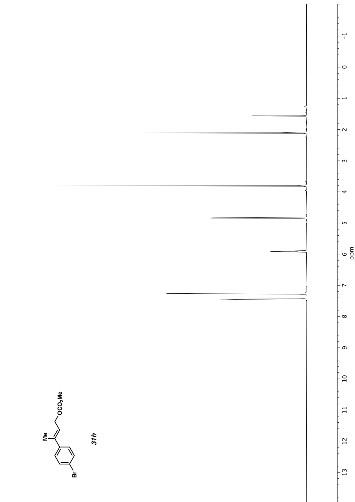
Figure A1.90 ^1\text{H} NMR (400 MHz, \text{CDCl}_3 ) of compound 31h .
