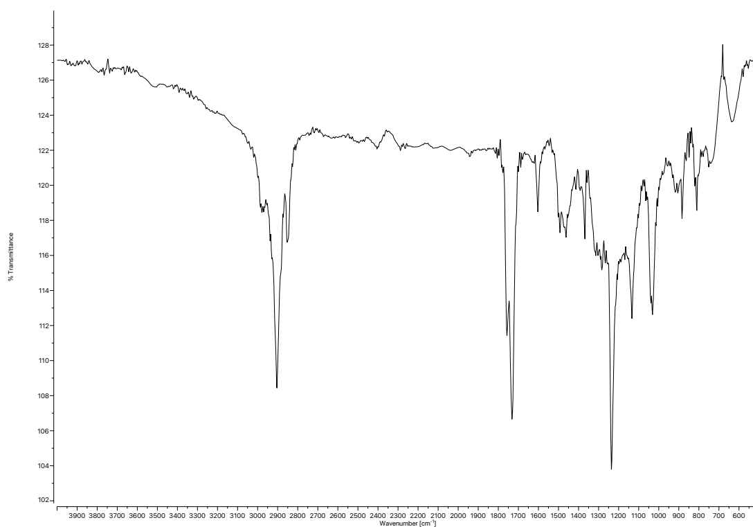
Figure A1.52 Infrared spectrum (Thin Film, NaCl) of compound 32n .
