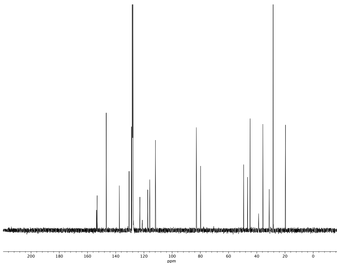
Figure A3.78 13 C NMR (100 MHz, CDCl 3 ) of compound 106 .
