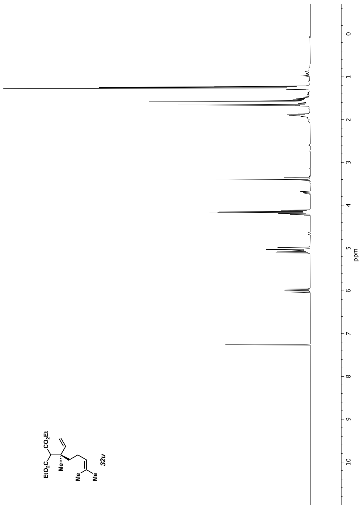
Figure A1.66 ^1\text{H} NMR (400 MHz, \text{CDCl}_3 ) of compound 32u .
