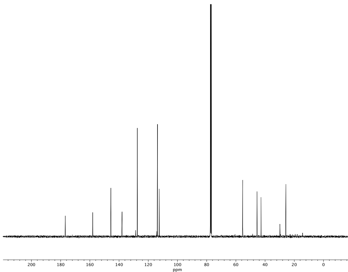
Figure A1.83 13 C NMR (100 MHz, CDCl 3 ) of compound 44 .
