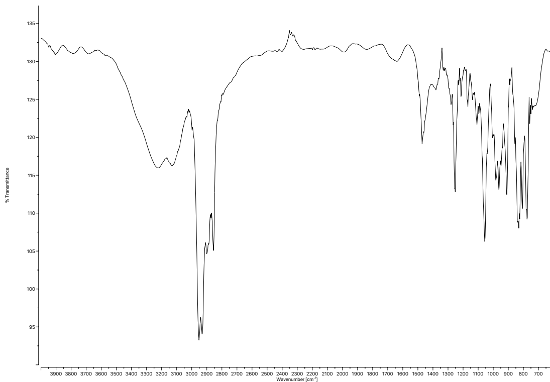
Figure A3.35 Infrared spectrum (Thin Film, NaCl) of compound (E)-86.
