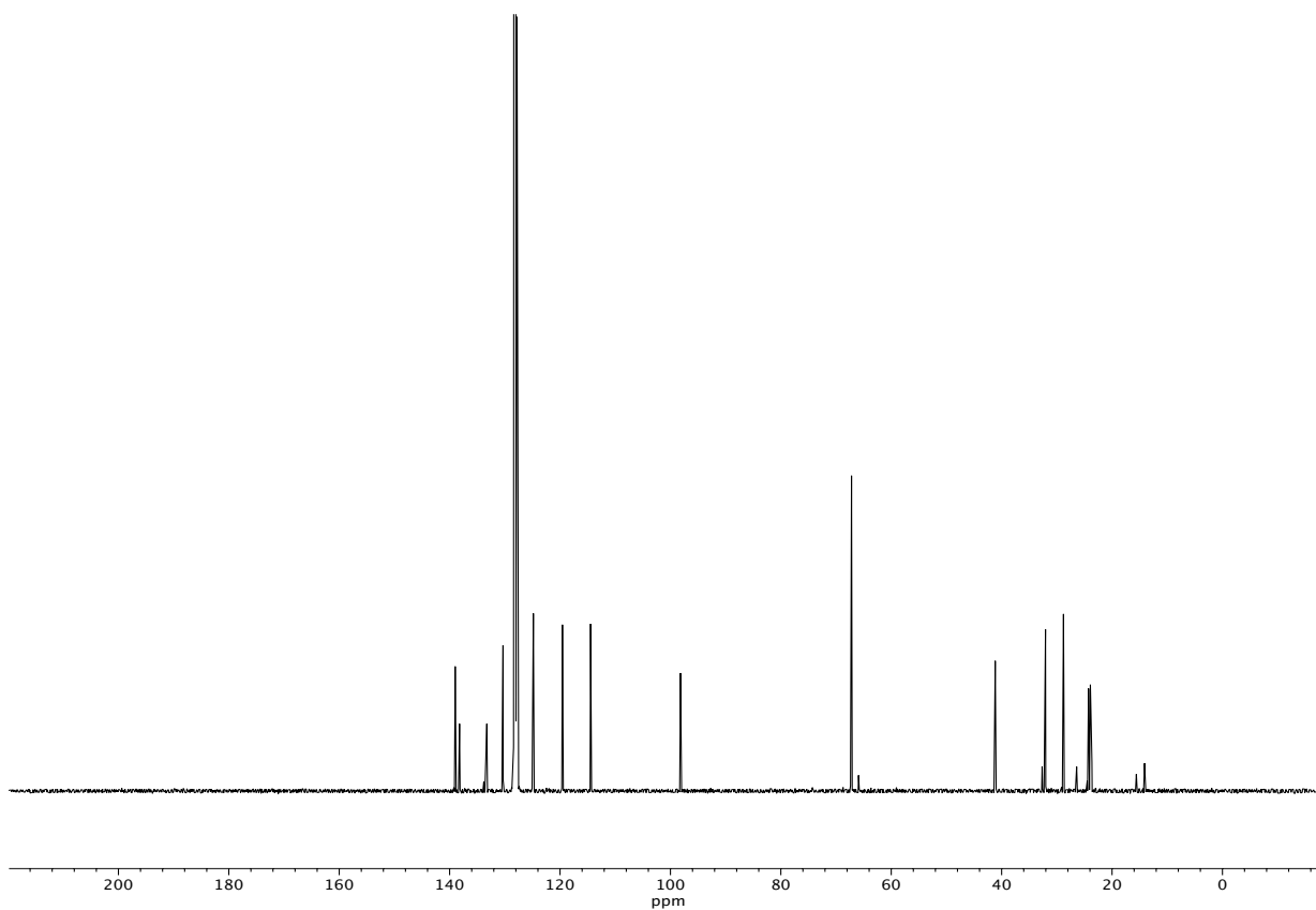
Figure A5.27 13 C NMR (100 MHz, C 6 D 6 ) of compound 154 .
