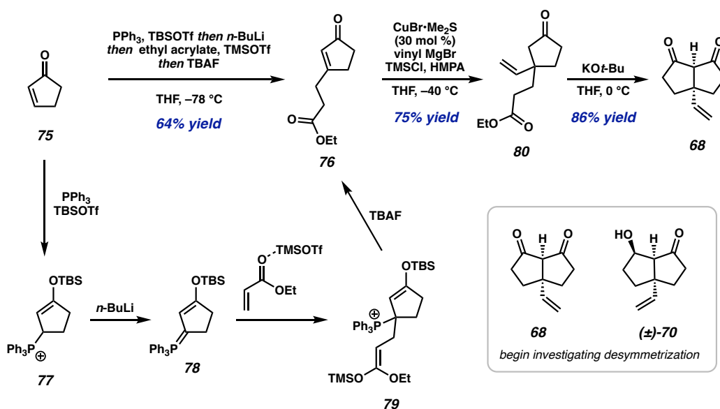
Scheme 2.4.2. Construction of bicyclic diketone 68 .
