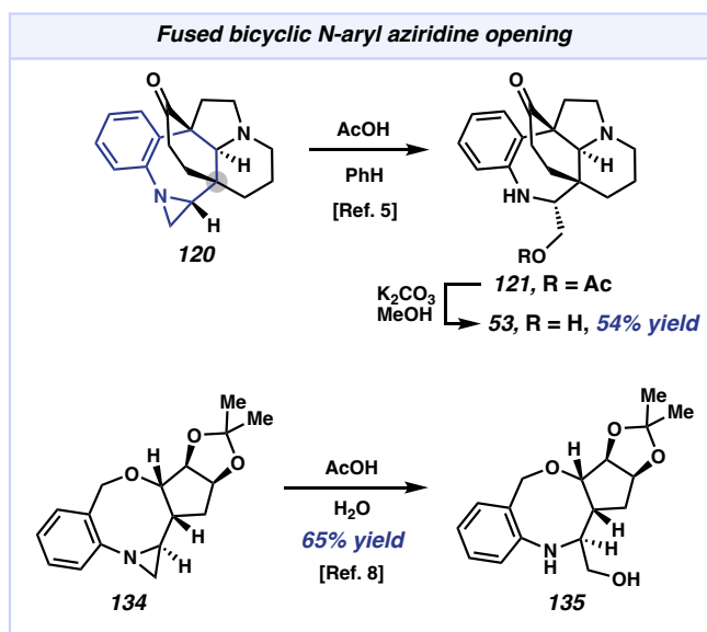
Scheme 3.1.2 Ring opening reactions of fused bicyclic N -aryl aziridines
