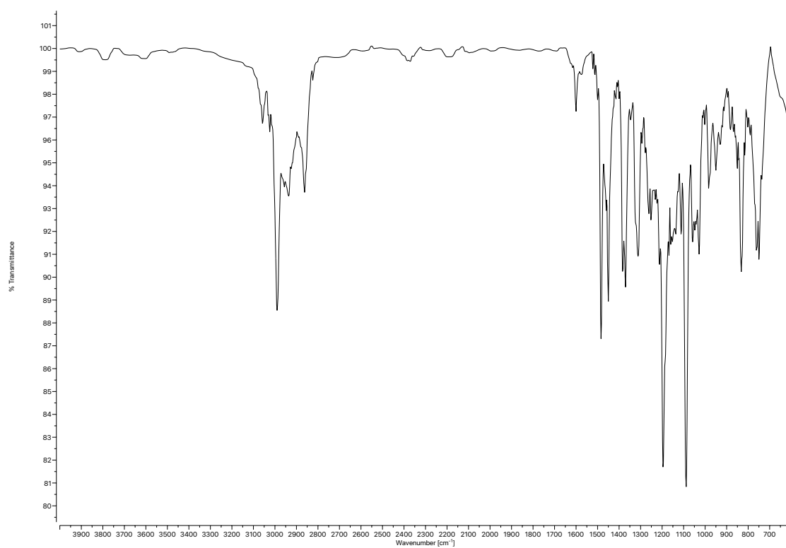
Figure A5.32 Infrared spectrum (Thin Film, NaCl) of compound 157 .
