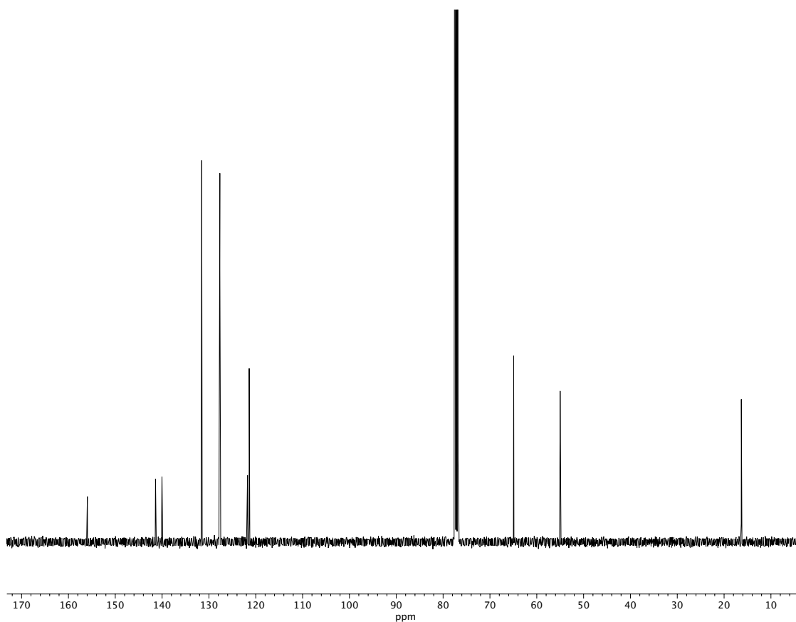
Figure A1.92 13 C NMR (100 MHz, CDCl 3 ) of compound 31h .
