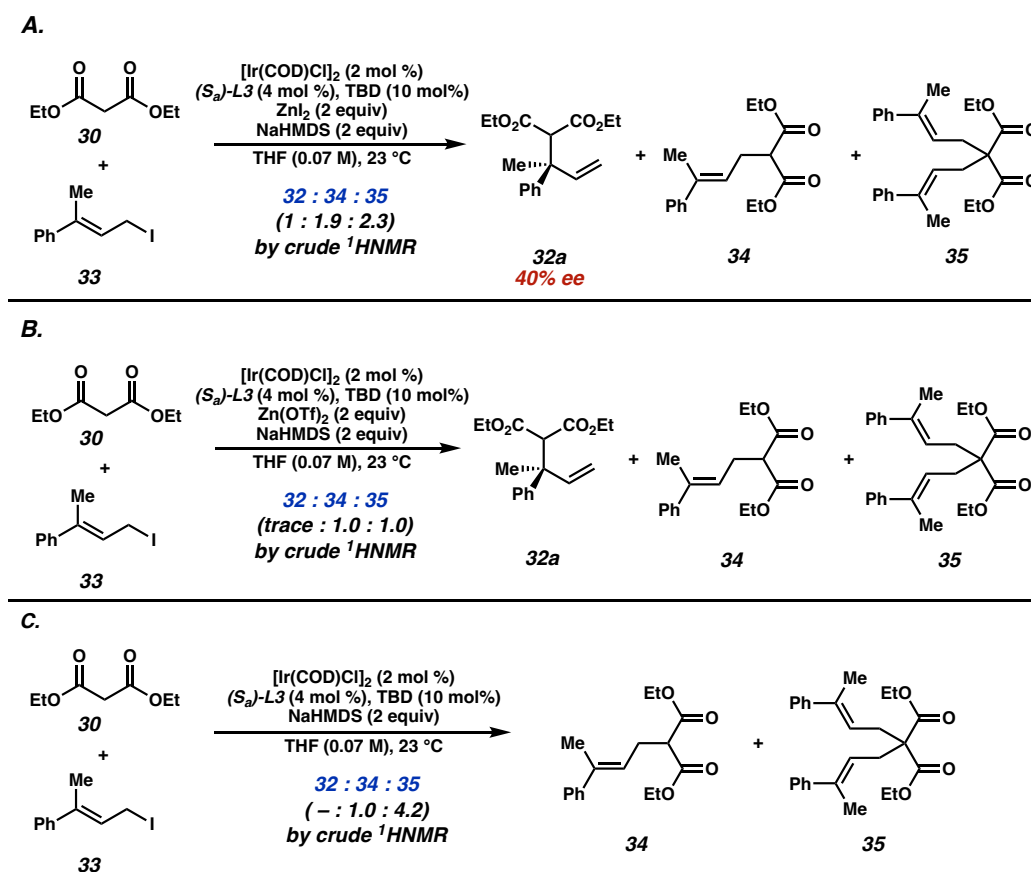
Scheme 1.6.1. Control experiments and mechanistic probes.
