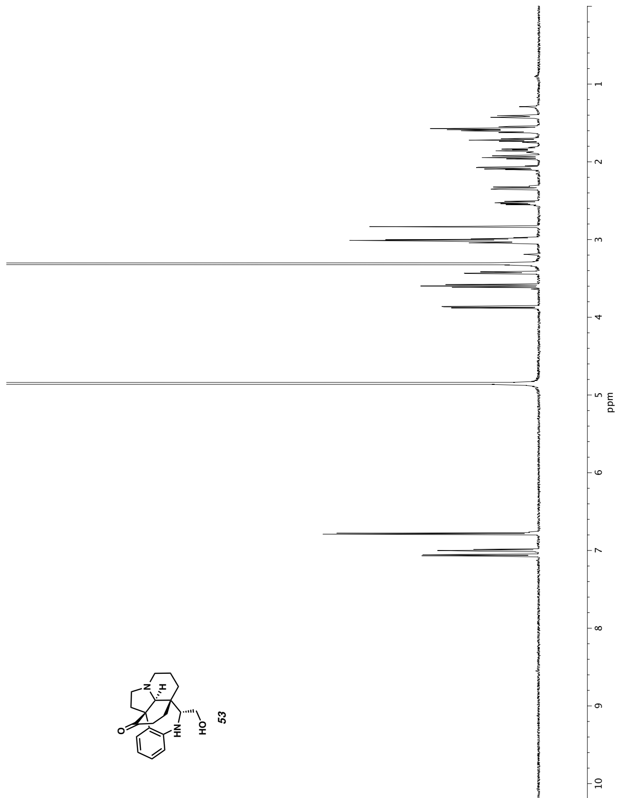
Figure A3.98 1 H NMR (600 MHz, CD 3 OD) of compound 53.
