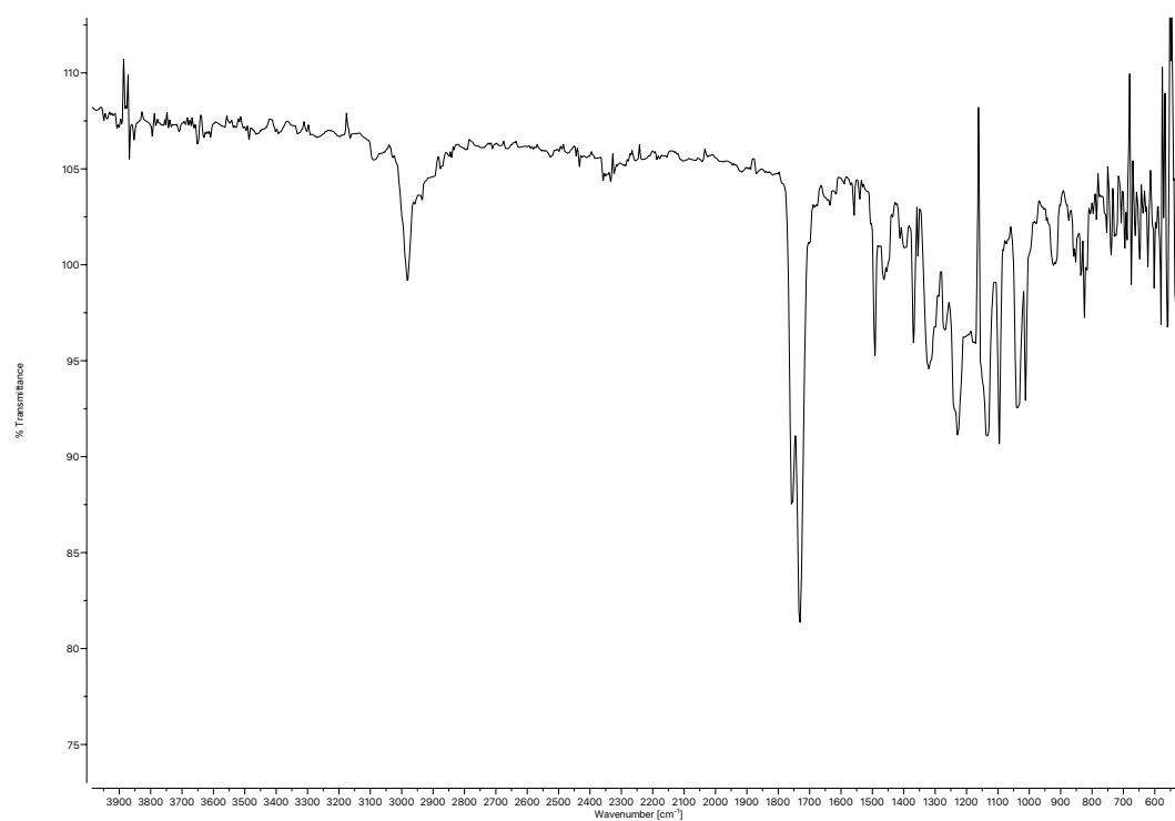
Figure A1.35 Infrared spectrum (Thin Film, NaCl) of compound 32i .
