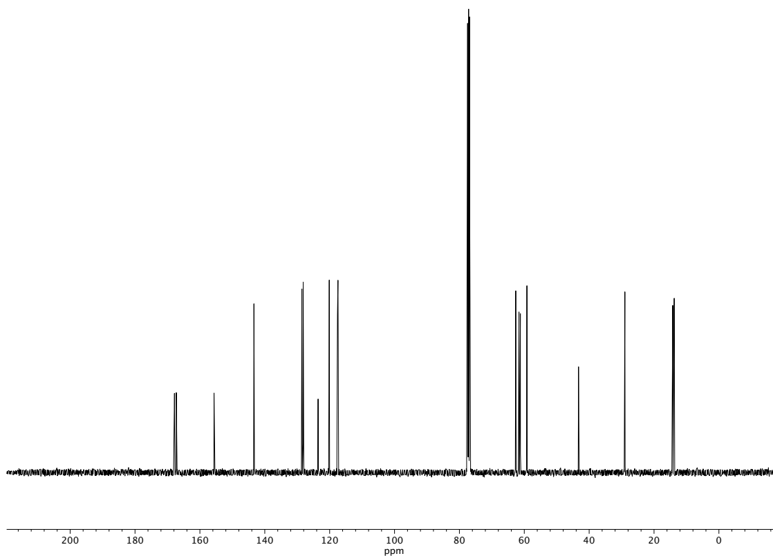
Figure A1.62 13 C NMR (100 MHz, CDCl 3 ) of compound 32s .
