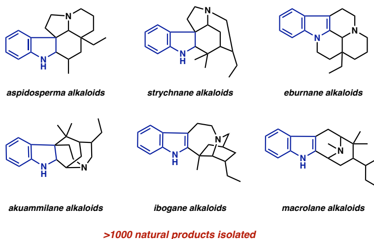
Figure 2.1.1. Carbon skeletons of various MIA subfamilies.
