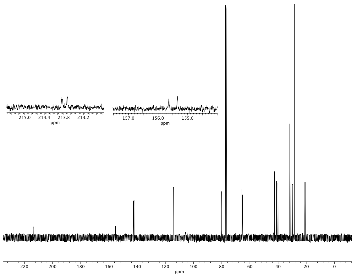
Figure A1.48 13 C NMR (150 MHz, CDCl 3 ) of compound 67b .
