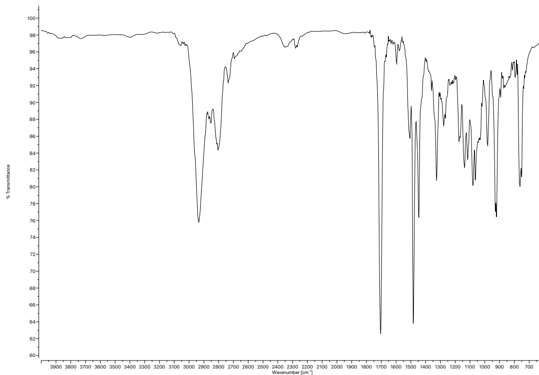
Figure A3.91 Infrared spectrum (Thin Film, NaCl) of compound 116 .
