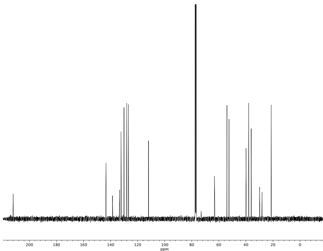
Figure A3.63 13 C NMR (100 MHz, CDCl 3 ) of compound 97 .
