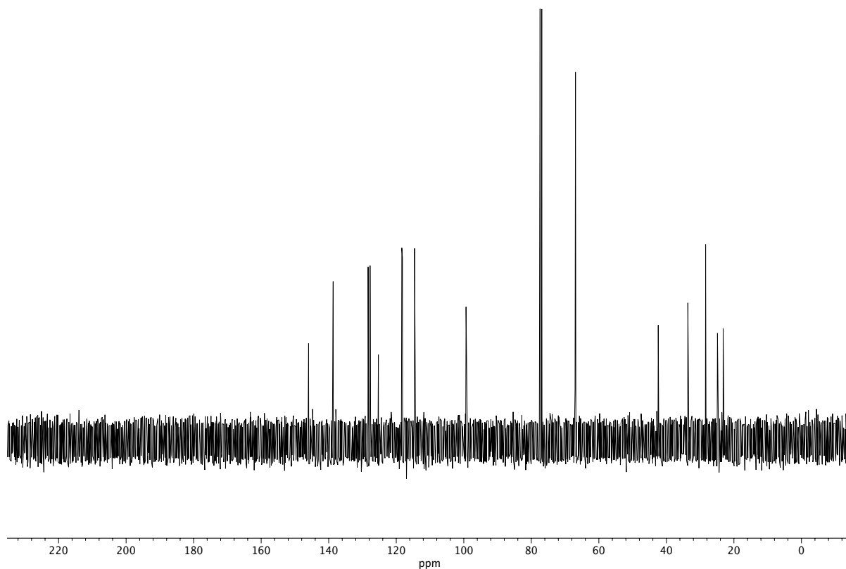
Figure A5.21 13 C NMR (125 MHz, CDCl 3 ) of compound 152 .
