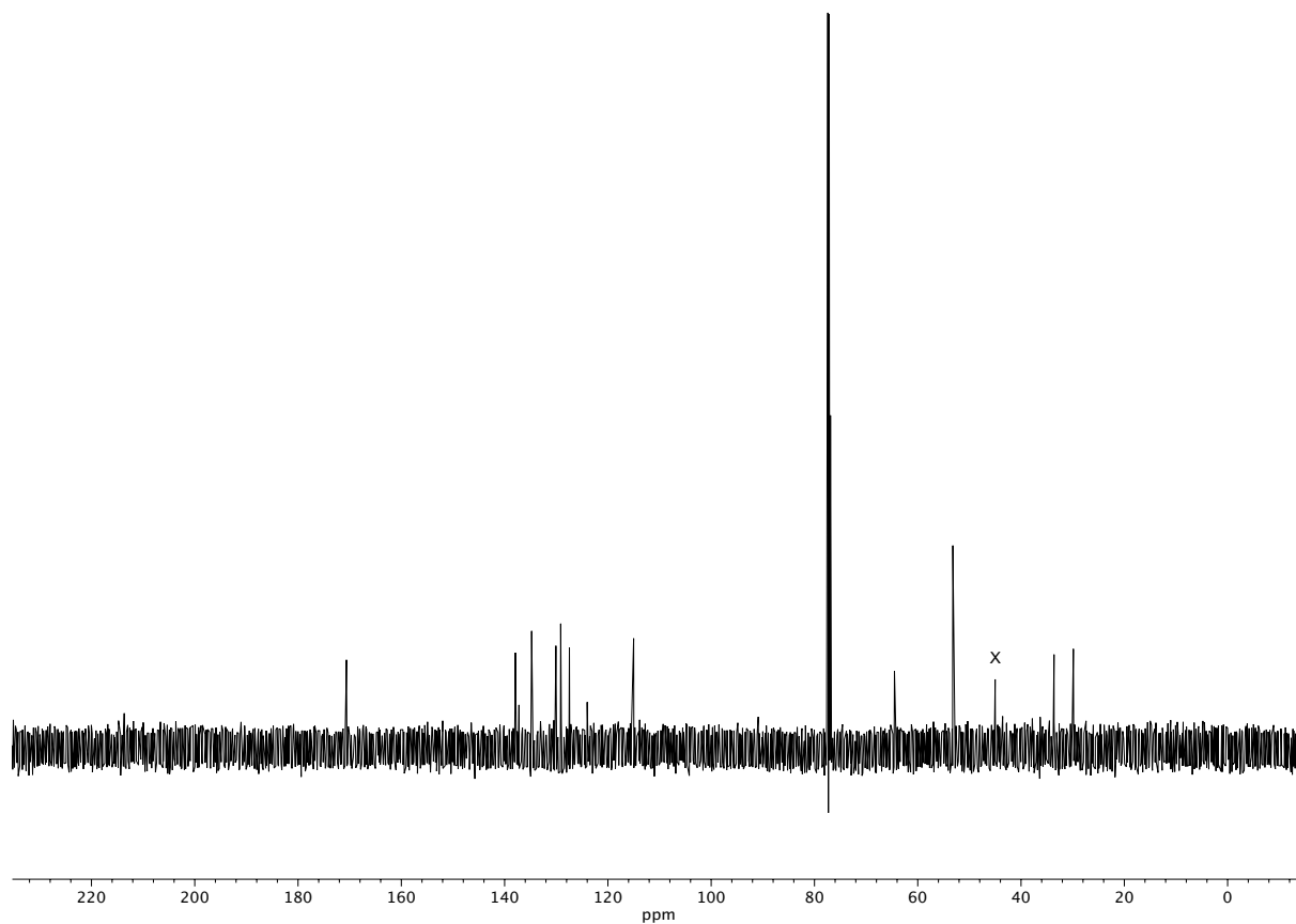
Figure A5.7 13 C NMR (125 MHz, CDCl 3 ) of compound 146 .
