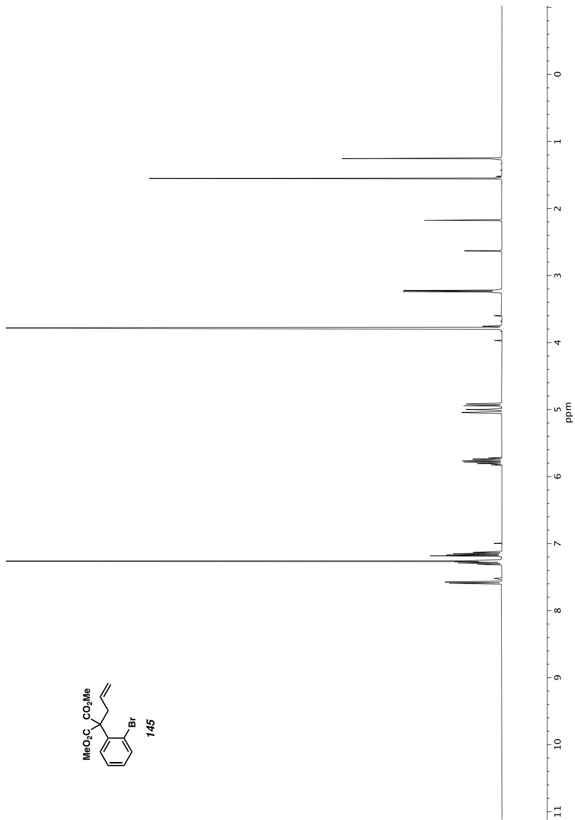
Figure A5.2 1 H NMR (400 MHz, CDCl 3 ) of compound 145 .
