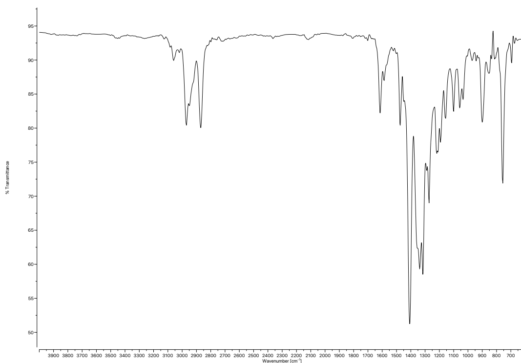
Figure A3.56 Infrared spectrum (Thin Film, NaCl) of compound 92 .
