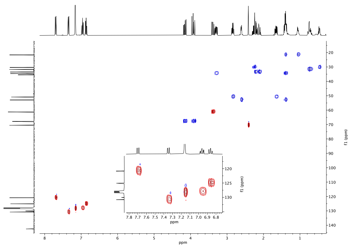
Figure A3.93 HSQC spectrum ( C_6D_6 ) of compound 116 .
