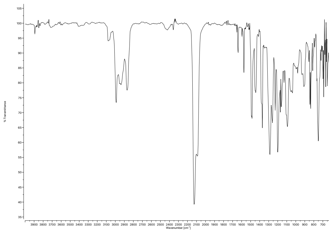
Figure A5.26 Infrared spectrum (Thin Film, NaCl) of compound 154 .
