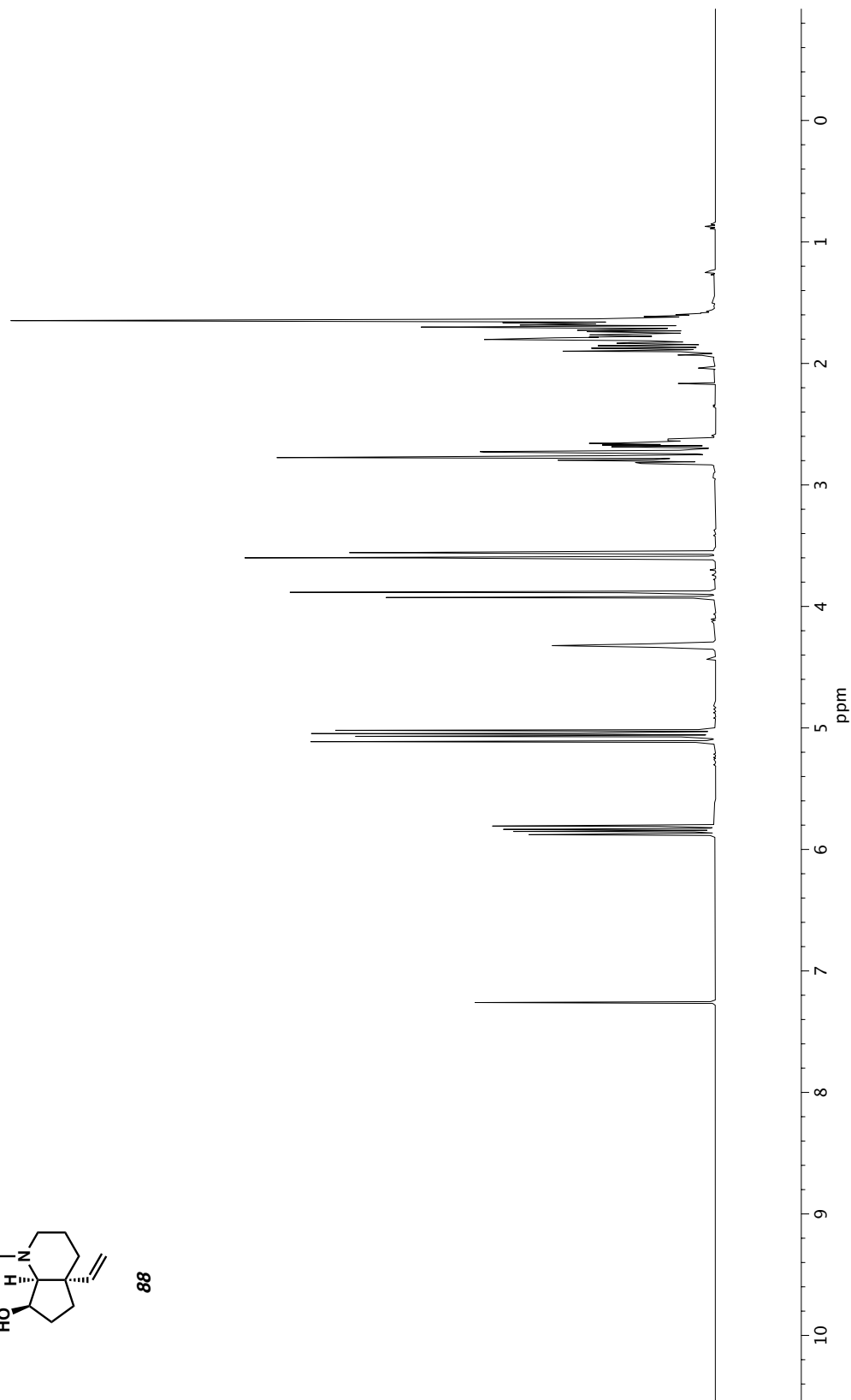
Figure A3.40 1 H NMR (400 MHz, CDCl 3 ) of compound 88 .
