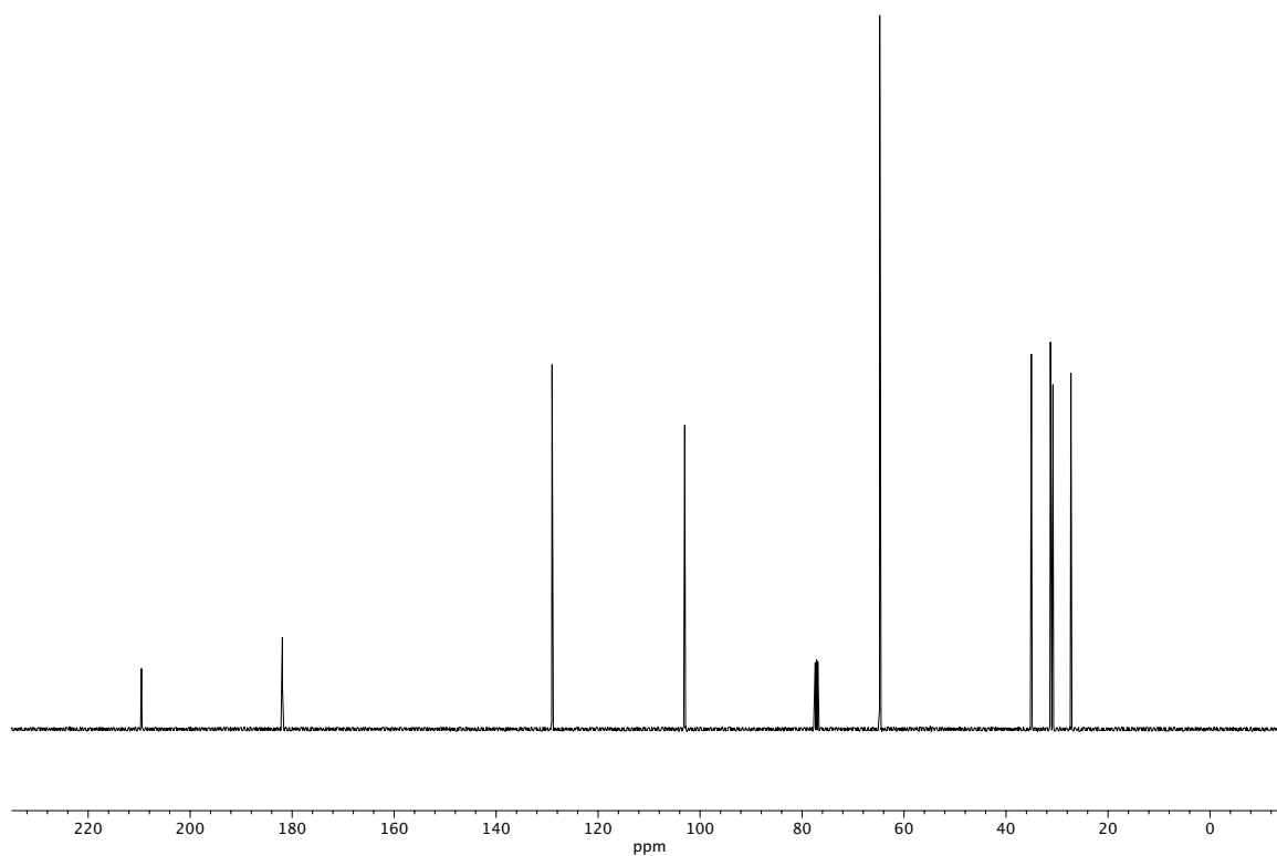
Figure A3.3 13 C NMR (125 MHz, CDCl 3 ) of compound 72 .
