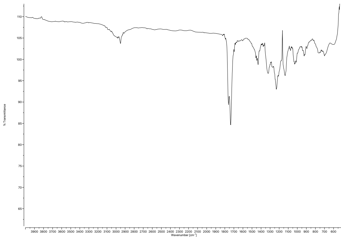
Figure A1.5 Infrared spectrum (Thin Film, NaCl) of compound 33 .
