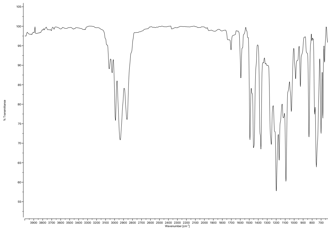
Figure A.53 Infrared spectrum (Thin Film, NaCl) of compound 161 .
