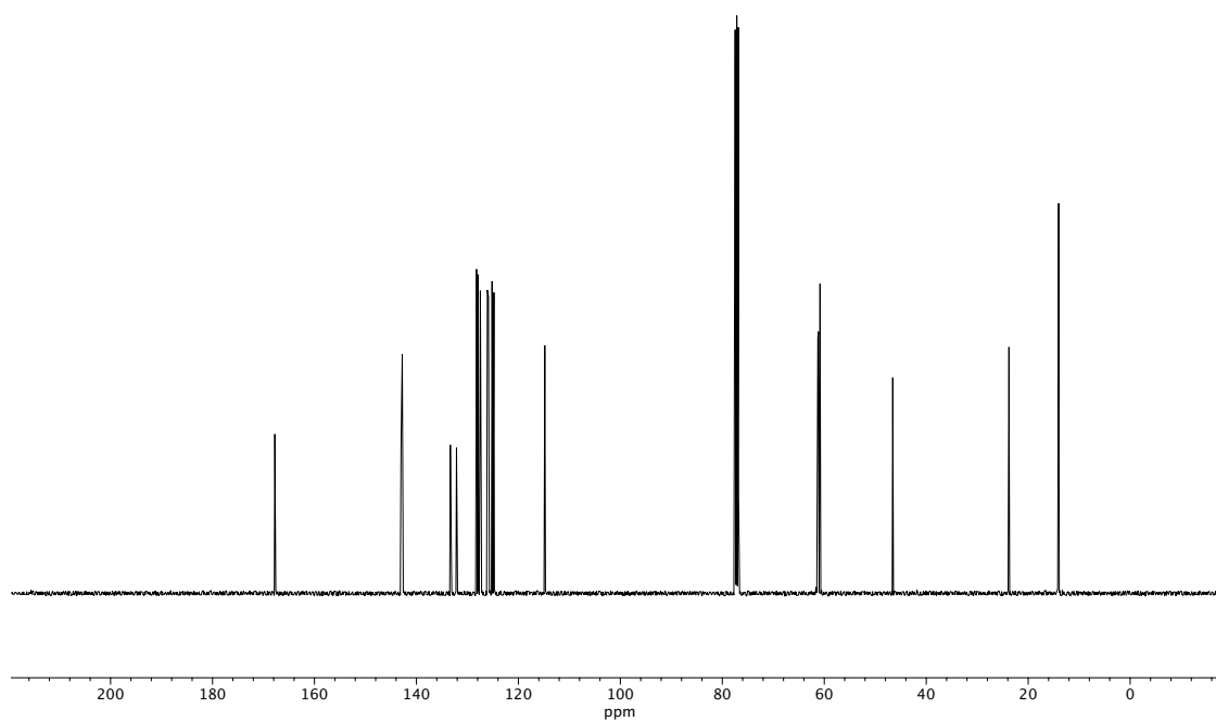
Figure A1.15 13 C NMR (100 MHz, CDCl 3 ) of compound 32b .
