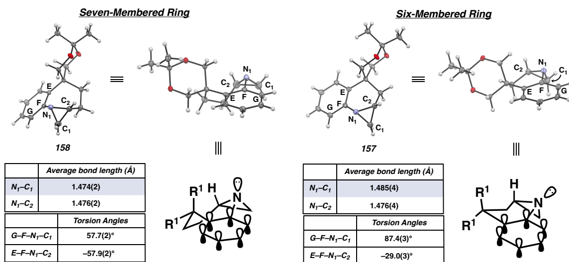
Figure 3.3.1 Conformational analysis of aziridines and identification of a relationship between lone pair conjugation and N1–C1 bond length
