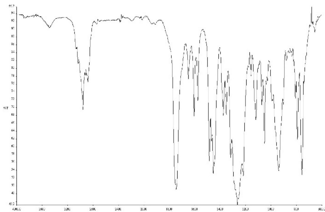
Figure A1.118 Infrared spectrum (Thin Film, NaCl) of compound 31s .
