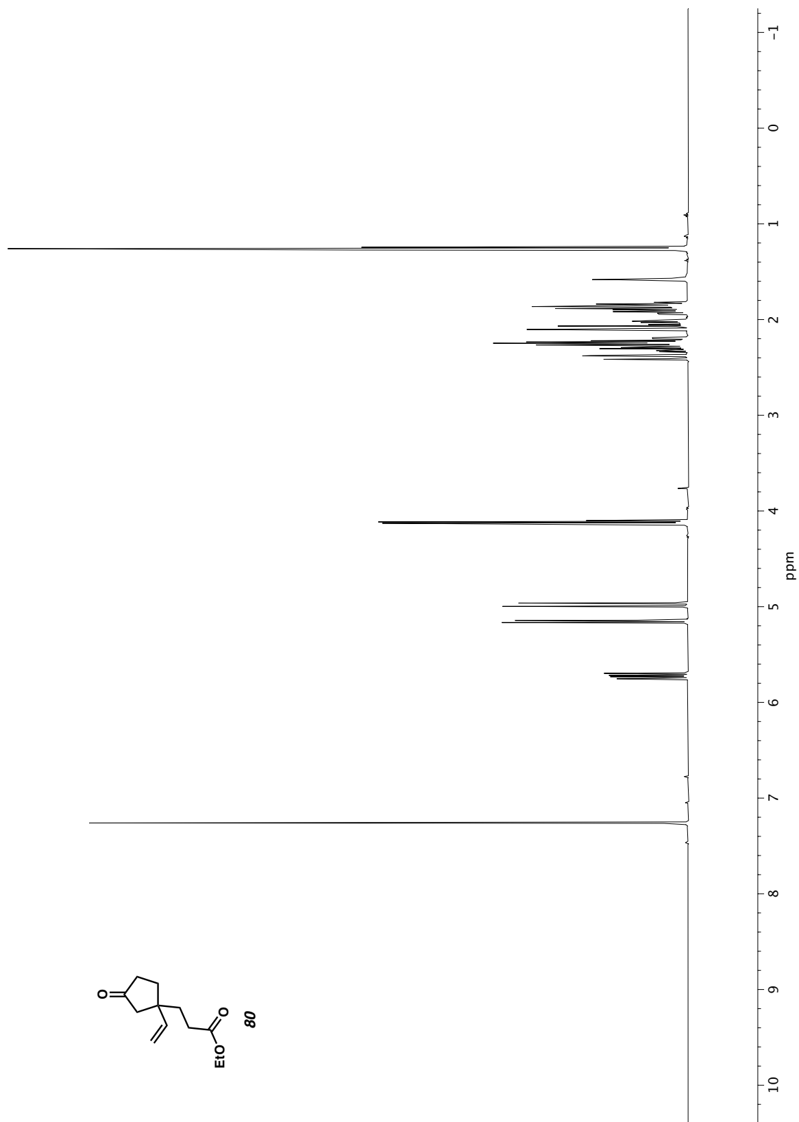
Figure A3.10 1 H NMR (500 MHz, CDCl 3 ) of compound 80 .
