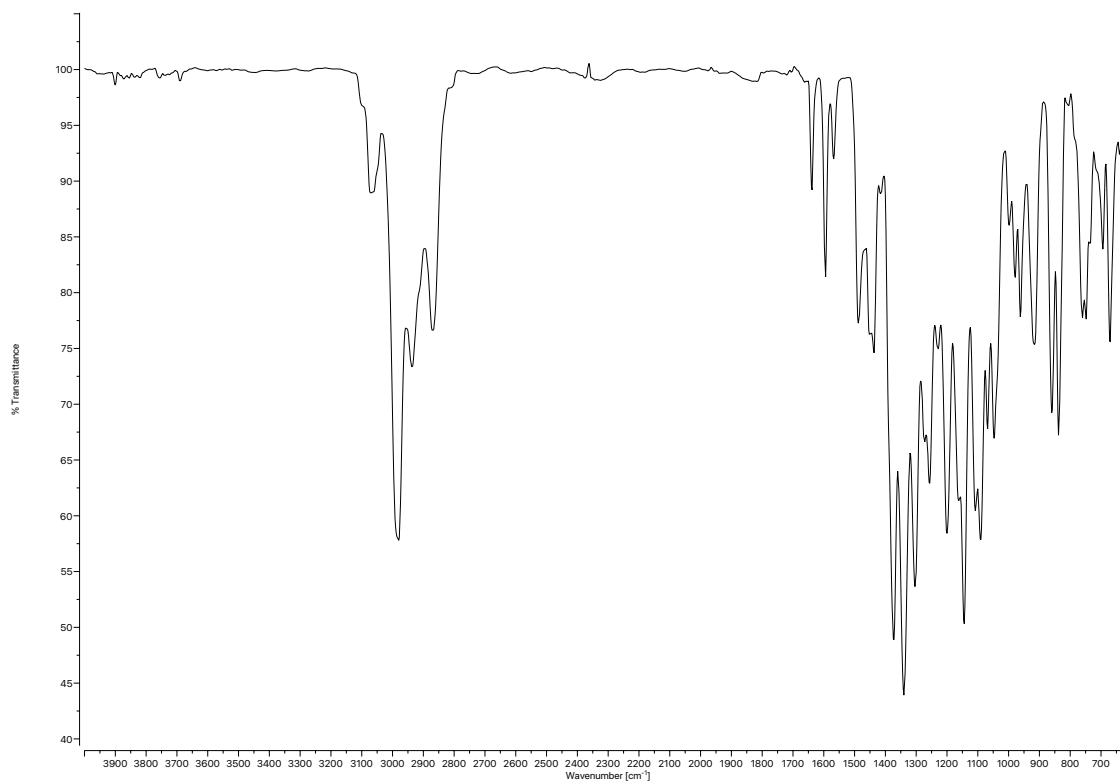
Figure A5.9 Infrared spectrum (Thin Film, NaCl) of compound 149 .
