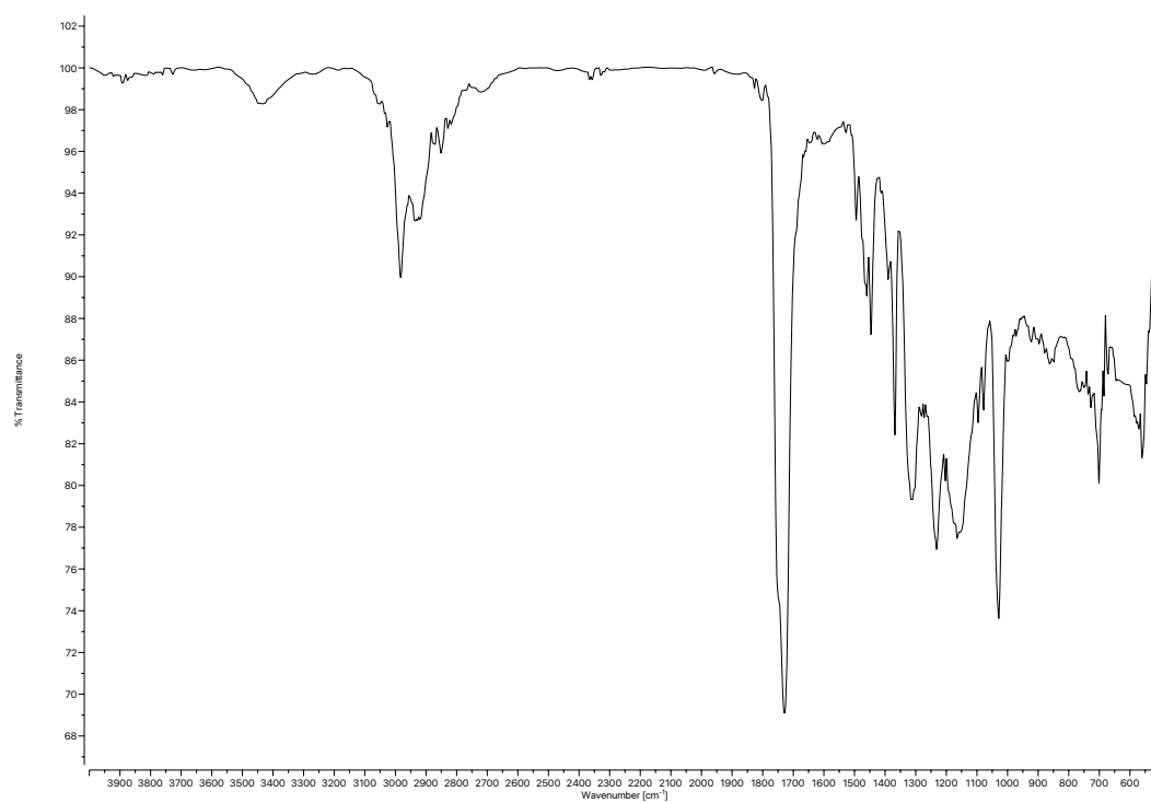
Figure A1.73 Infrared spectrum (Thin Film, NaCl) of compound 41 .
