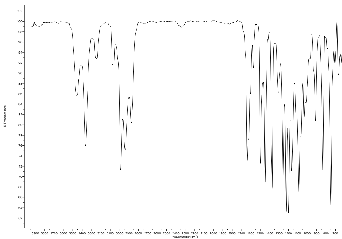
Figure A5.20 Infrared spectrum (Thin Film, NaCl) of compound 152 .
