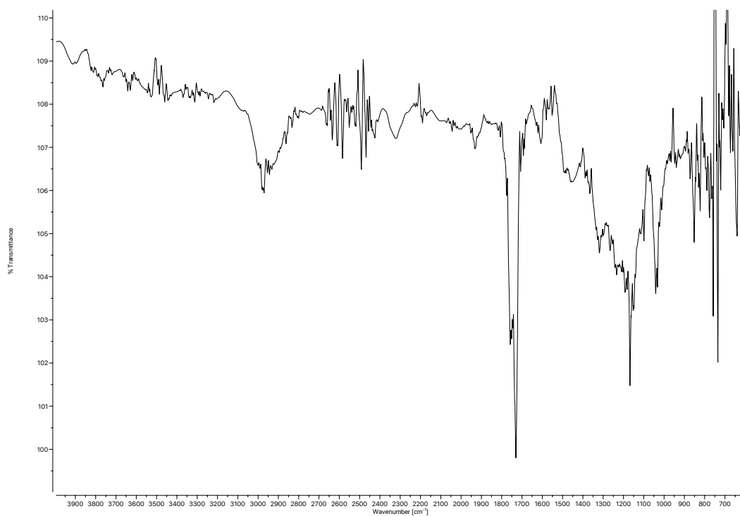
Figure A1.64 Infrared spectrum (Thin Film, NaCl) of compound 32t .
