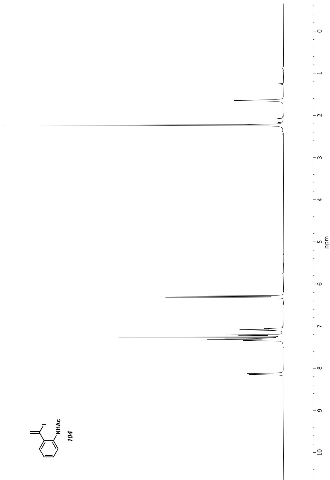
Figure A3.70 1 H NMR (500 MHz, CDCl 3 ) of compound 104 .
