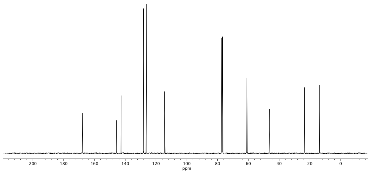
Figure A1.3 13 C NMR (100 MHz, CDCl 3 ) of compound 32a .
