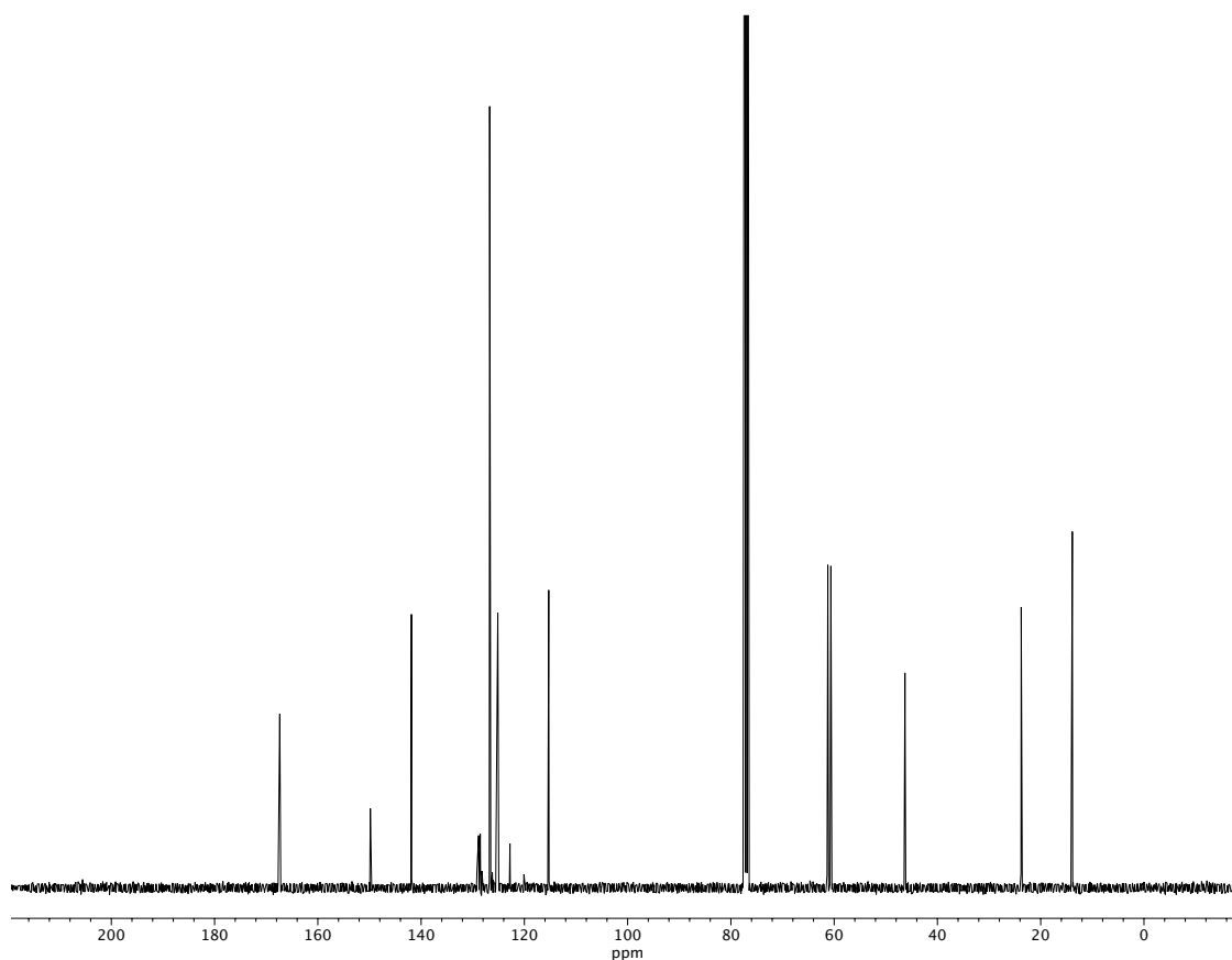
Figure A1.40 13 C NMR (100 MHz, CDCl 3 ) of compound 32j .
