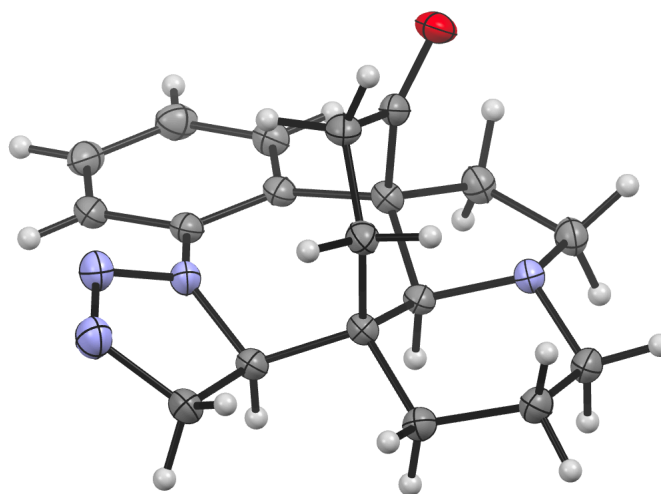
Figure A4.6.1. X-Ray Coordinate of 117 (V23195)
