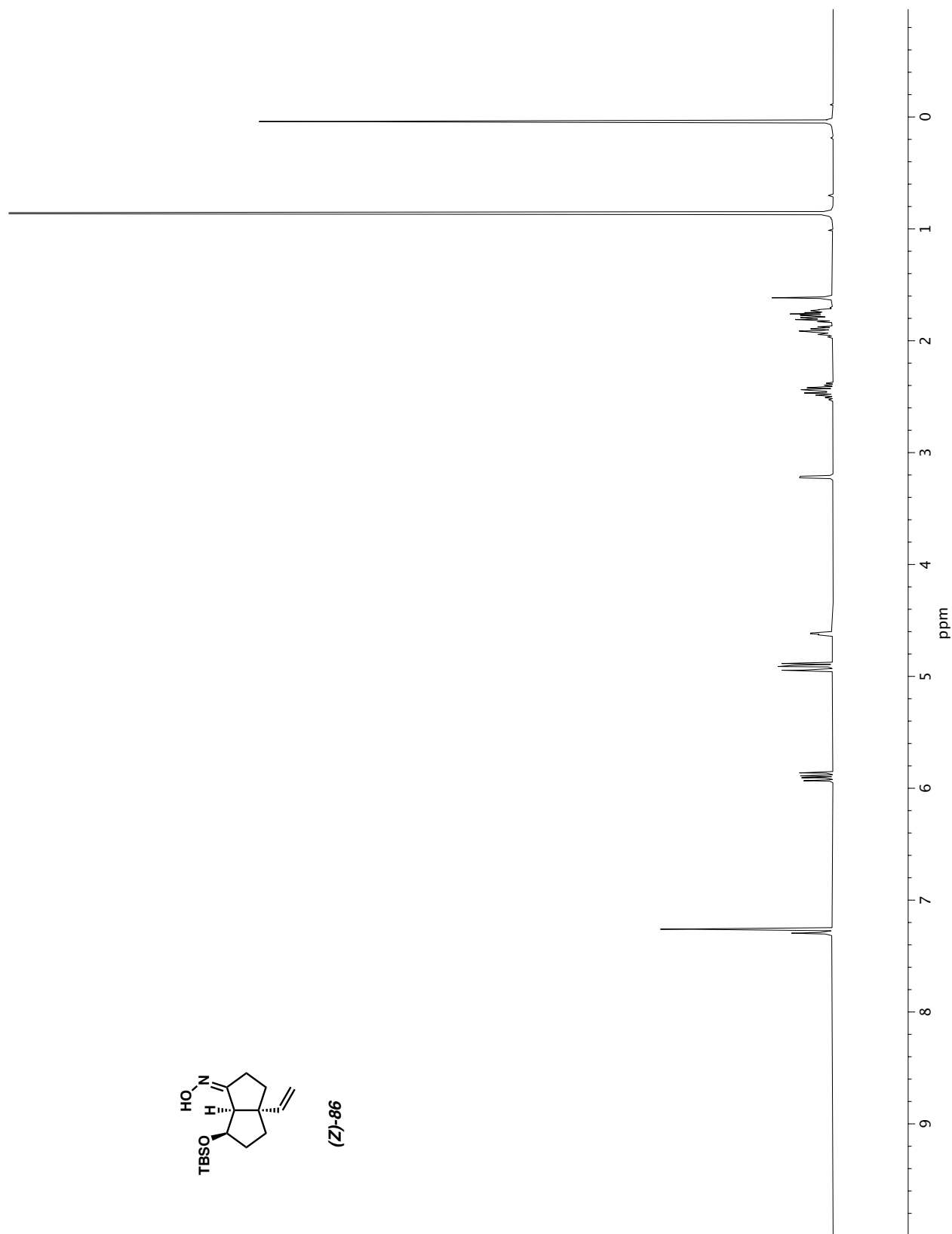
Figure A3.31 ^1\text{H} NMR (400 MHz, \text{CDCl}_3 ) of compound (Z)-86.
