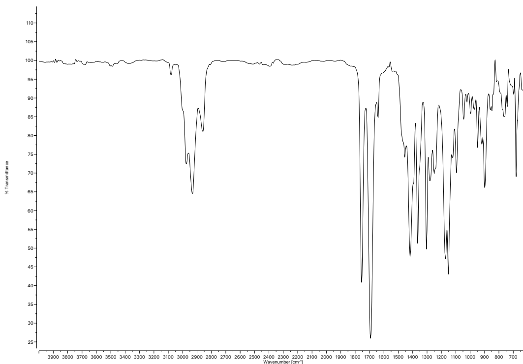
Figure A3.47 Infrared spectrum (Thin Film, NaCl) of compound 67b .
