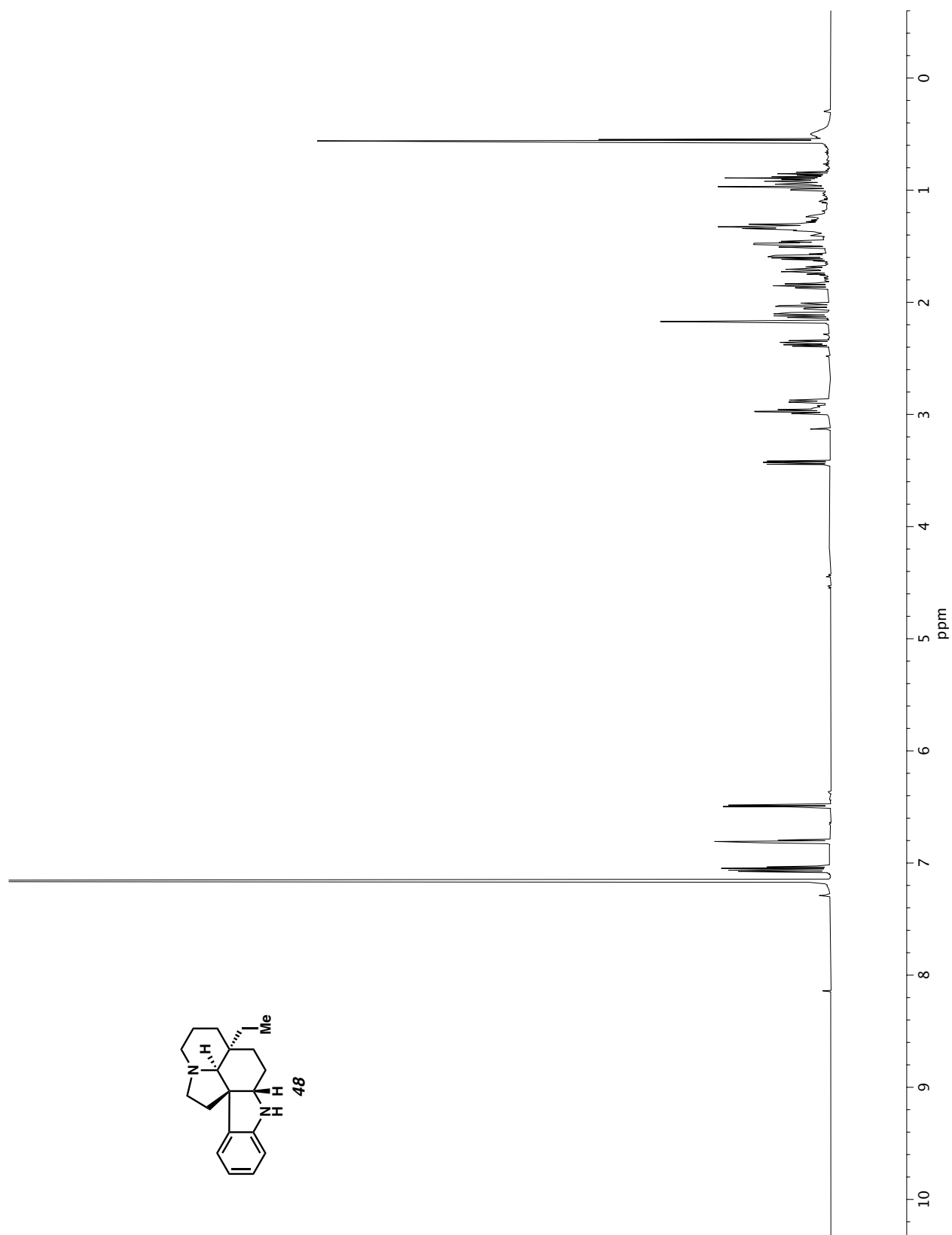
Figure A3.82 ^1\text{H} NMR (600 MHz, \text{C}_6\text{D}_6 ) of compound 48 .
