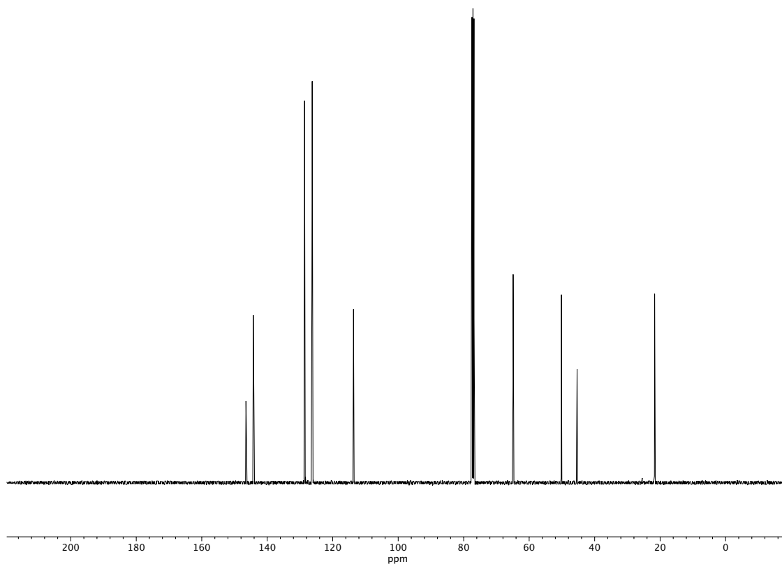
Figure A1.80 13 C NMR (100 MHz, CDCl 3 ) of compound 43 .
