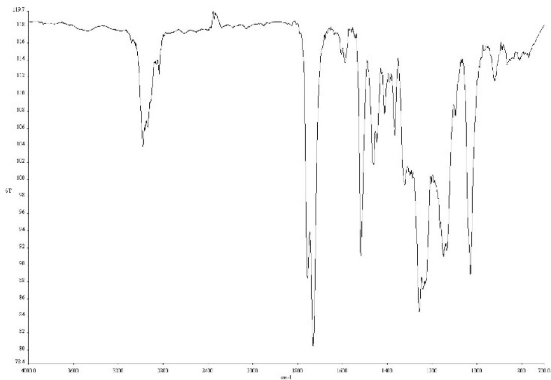
Figure A1.46 Infrared spectrum (Thin Film, NaCl) of compound 32I .
