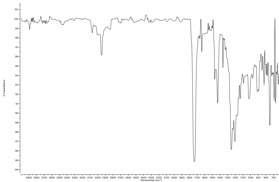
Figure A5.6 Infrared spectrum (Thin Film, NaCl) of compound 146 .
