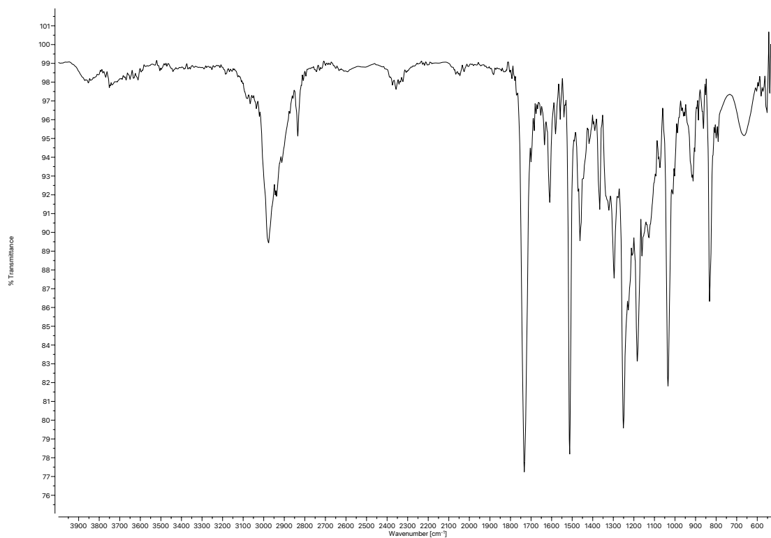
Figure A1.85 Infrared spectrum (Thin Film, NaCl) of compound 45 .
