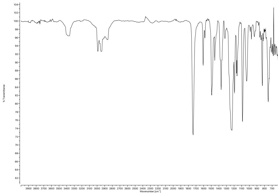
Figure A.59 Infrared spectrum (Thin Film, NaCl) of compound 162 .
