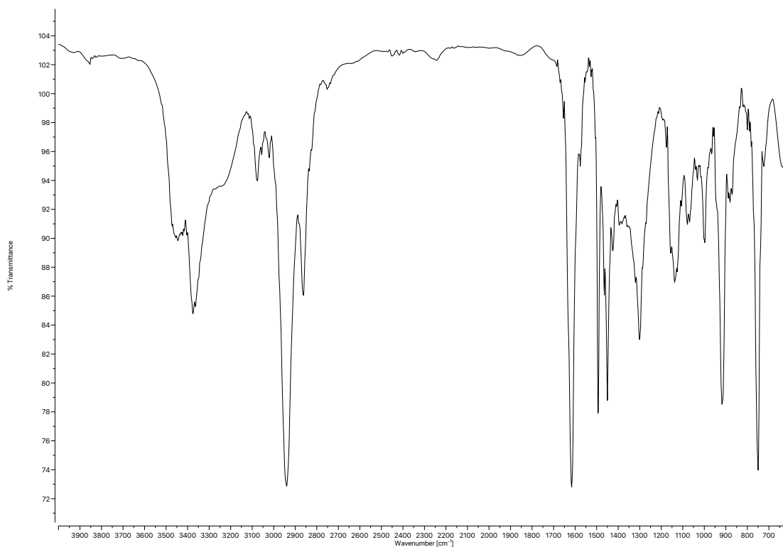
Figure A3.80 Infrared spectrum (Thin Film, NaCl) of compound 107 .
