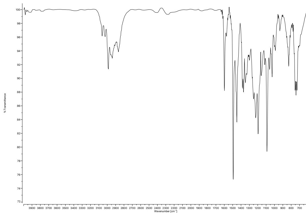
Figure A.71 Infrared spectrum (Thin Film, NaCl) of compound 164 .
