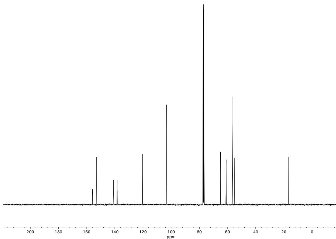
Figure A1.101 13 C NMR (100 MHz, CDCl 3 ) of compound 31m .
