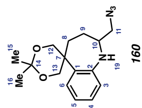
Figure A5.49 COSY spectrum ( \text{CDCl}_3 ) of compound 160 .
