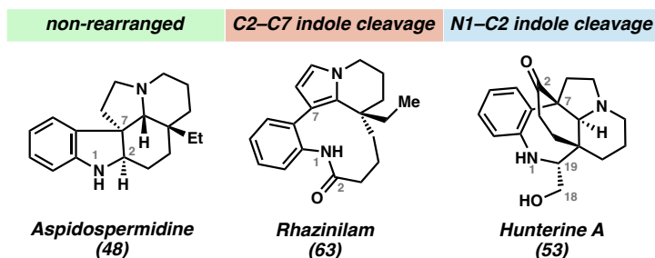
Figure 2.2.1. Aspidospermidine (non-rearranged) and rearranged aspidosperma MIAs.
