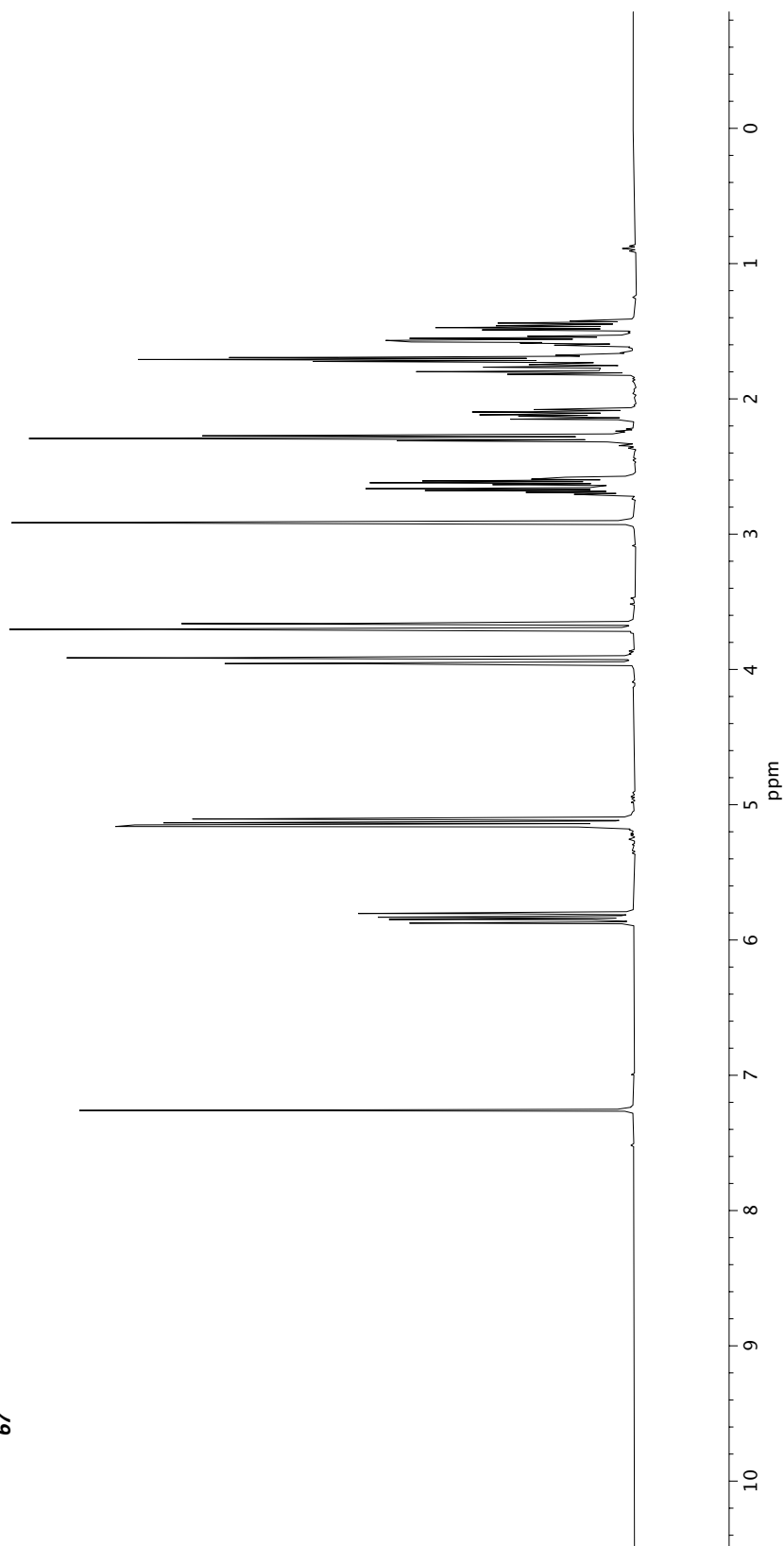
Figure A3.43 ^1\text{H} NMR (400 MHz, \text{CDCl}_3 ) of compound 67 .
