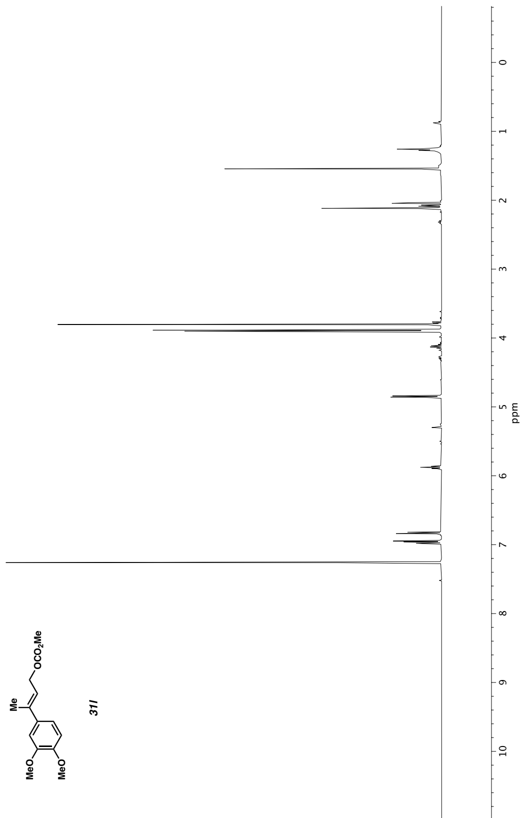
Figure A1.96 ^1\text{H} NMR (400 MHz, \text{CDCl}_3 ) of compound 31I .
