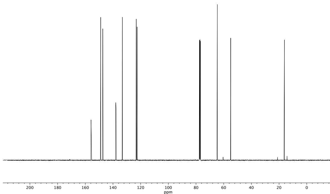
Figure A1.116 13 C NMR (100 MHz, CDCl 3 ) of compound 31q .
