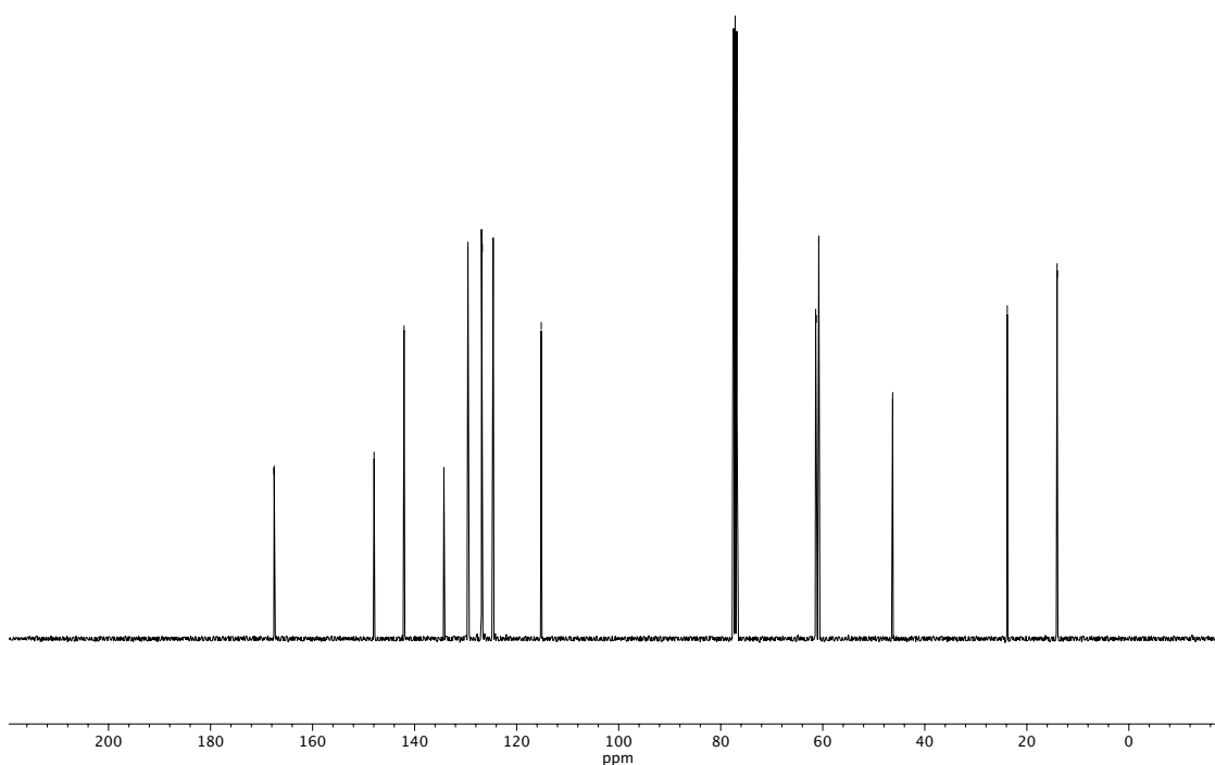
Figure A1.33 13 C NMR (100 MHz, CDCl 3 ) of compound 32h .
