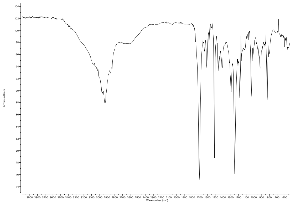
Figure A1.82 Infrared spectrum (Thin Film, NaCl) of compound 44 .
