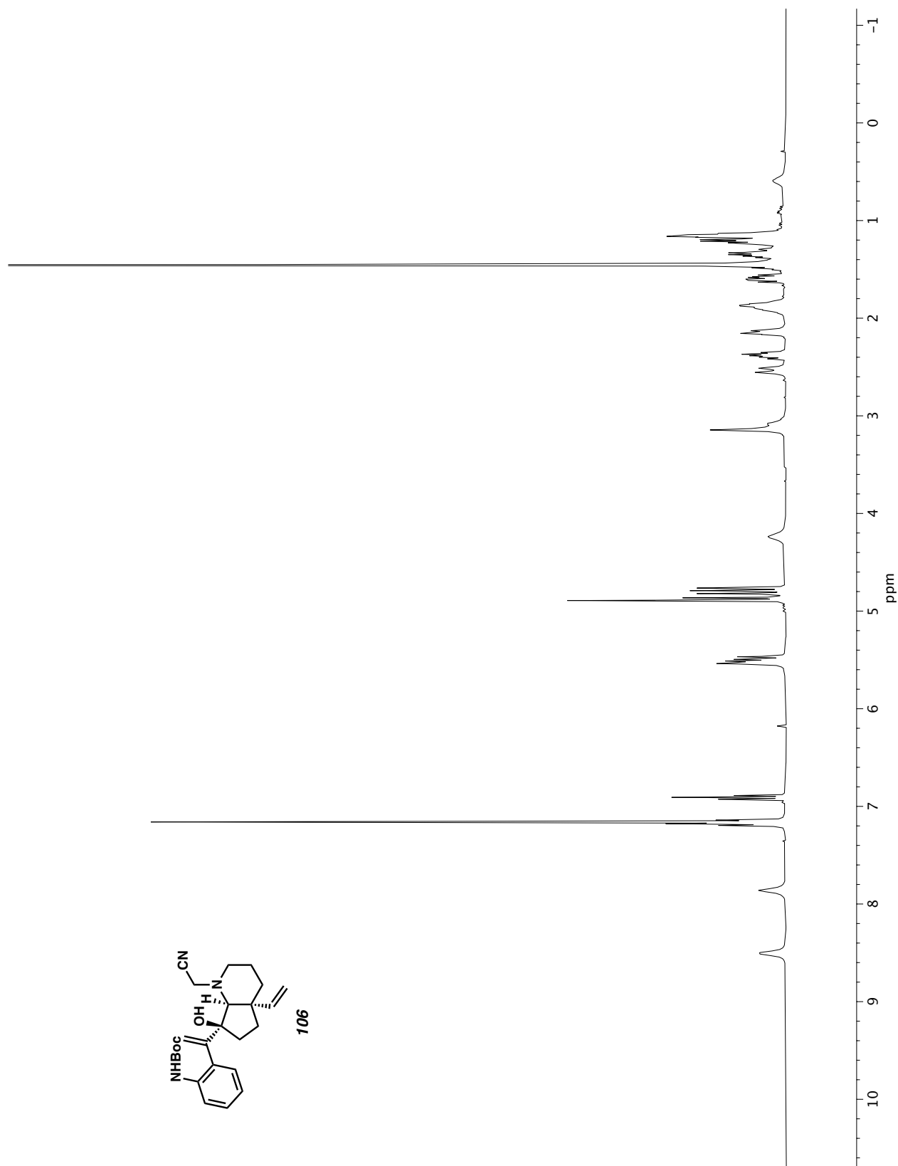
Figure A3.76 ^1\text{H} NMR (400 MHz, \text{CDCl}_3 ) of compound 106 .
