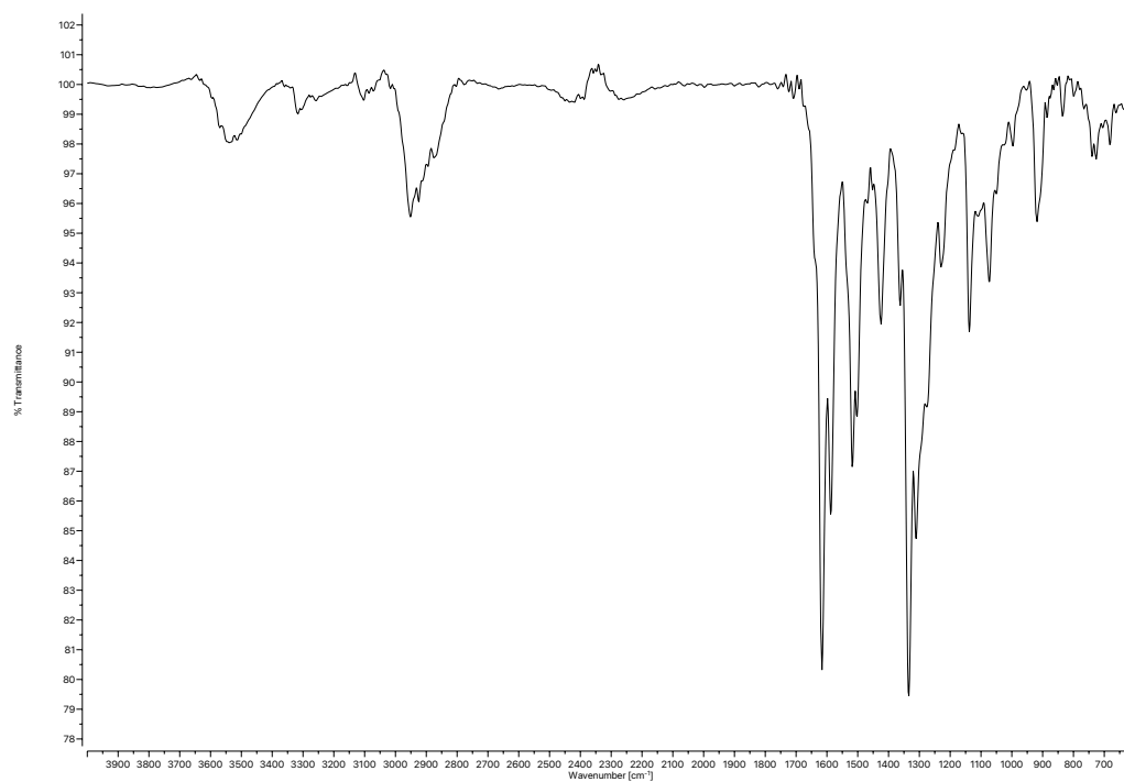
Figure A3.26 Infrared spectrum (Thin Film, NaCl) of compound 82 .
