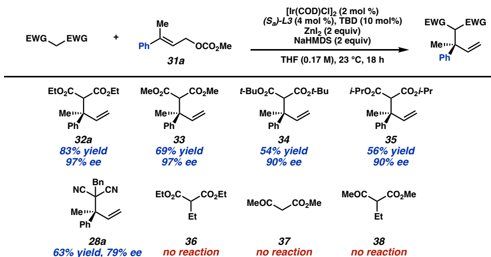
Scheme 1.8.1. Nucleophile scope.
