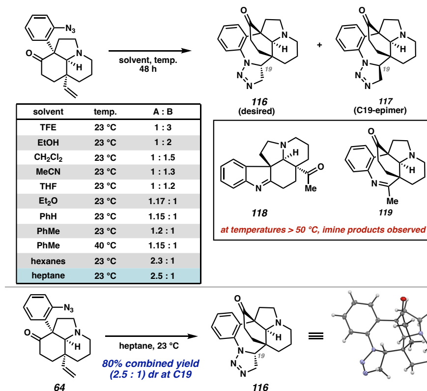
Scheme 2.4.13. Optimization of the [3+2] cycloaddition.
