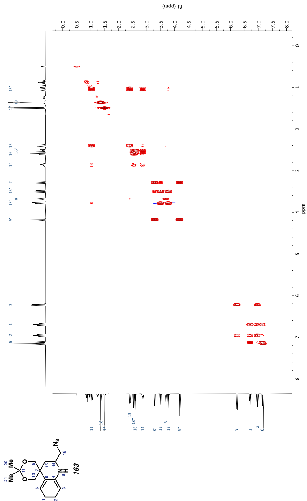
Figure A.67 COSY spectrum ( C_6D_6 ) of compound 163 .
