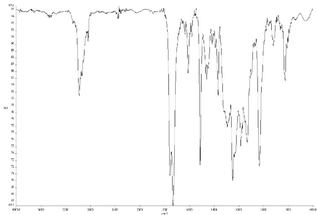
Figure A1.23 Infrared spectrum (Thin Film, NaCl) of compound 32e .
