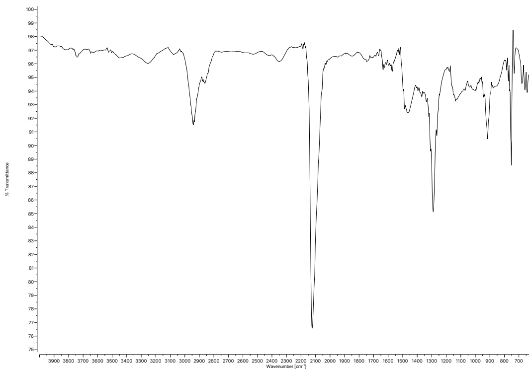
Figure A1.84 Infrared spectrum (Thin Film, NaCl) of compound 112 .
