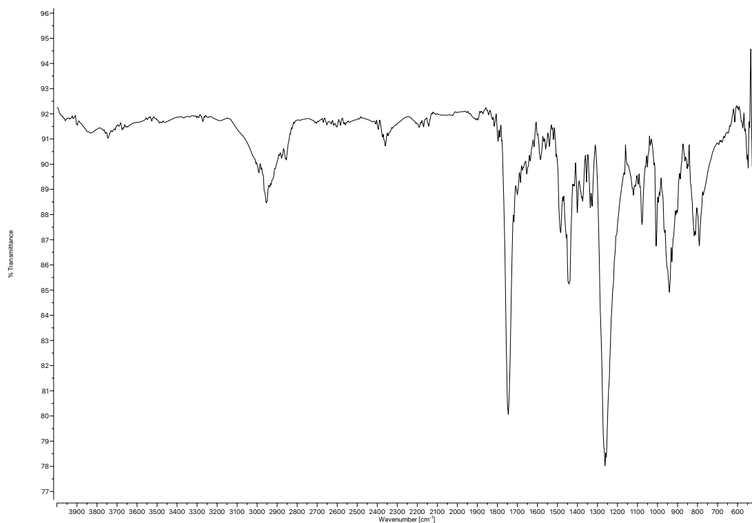
Figure A1.91 Infrared spectrum (Thin Film, NaCl) of compound 31h .
