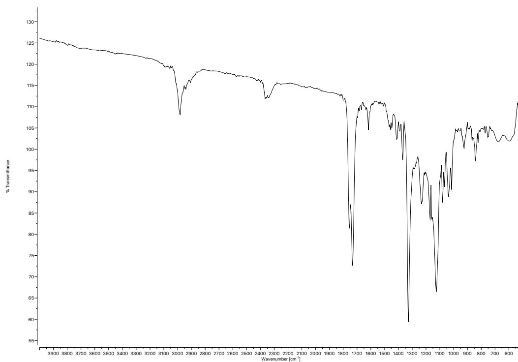
Figure A1.39 Infrared spectrum (Thin Film, NaCl) of compound 32j .
