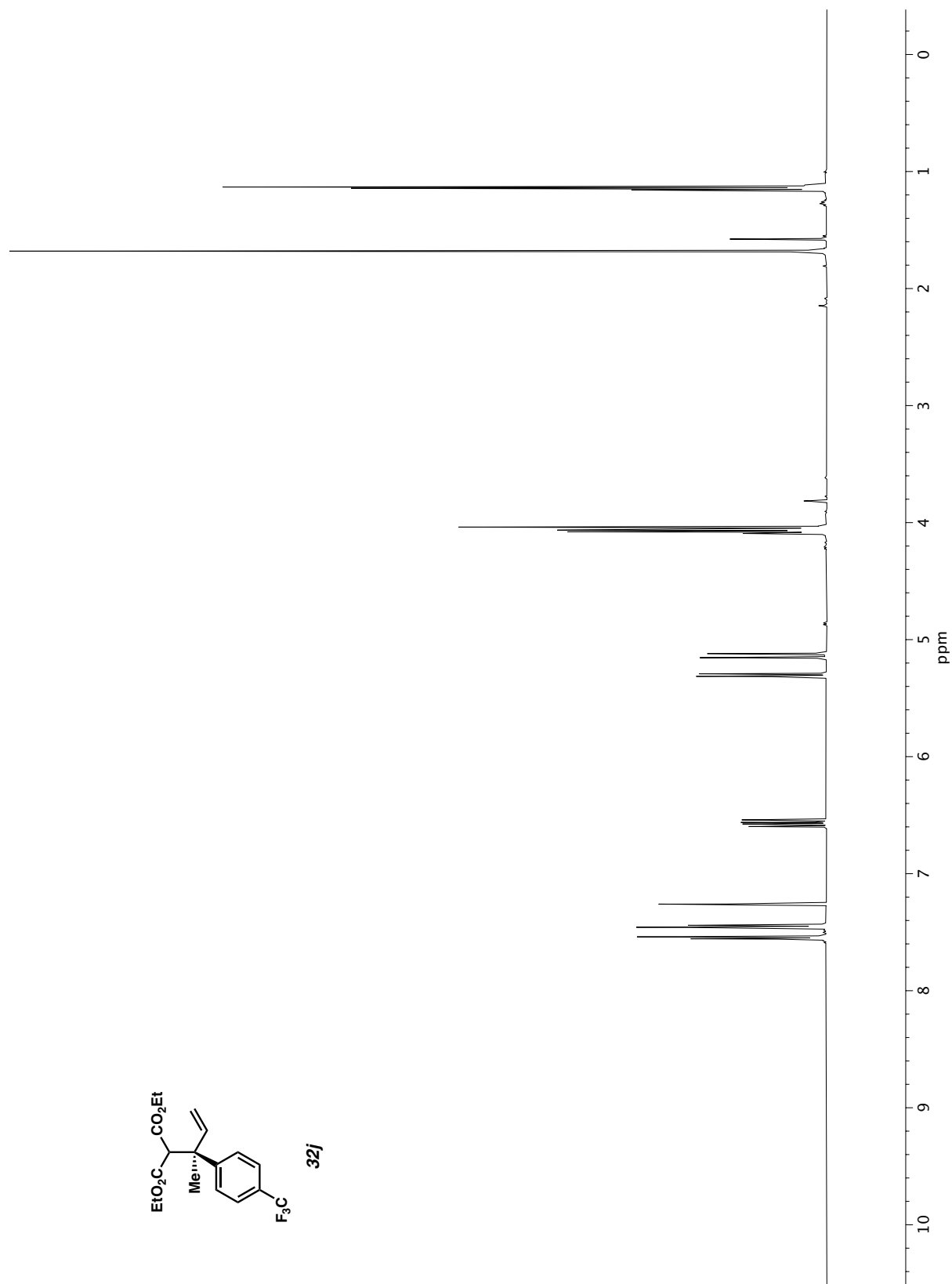
Figure A1.38 ^1\text{H} NMR (500 MHz, \text{CDCl}_3 ) of compound 32j .
