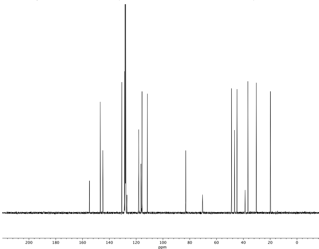
Figure A3.81 13 C NMR (100 MHz, C 6 D 6 ) of compound 107 .
