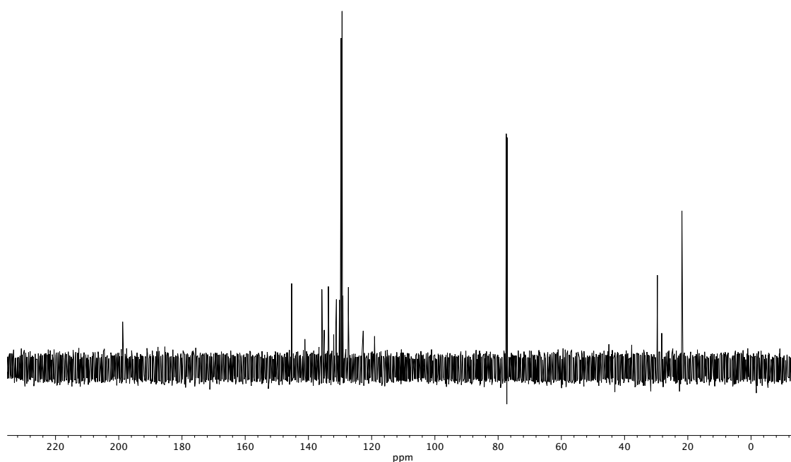
Figure A3.66 13 C NMR (125 MHz, CDCl 3 ) of compound 101 .
