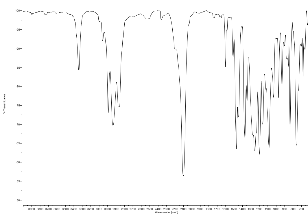
Figure A5.47 Infrared spectrum (Thin Film, NaCl) of compound 160 .
