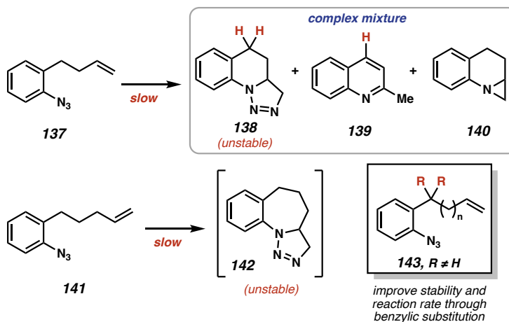
Scheme 3.2.1 Initial attempts to synthesize simplified bicyclic N -aryl aziridines
