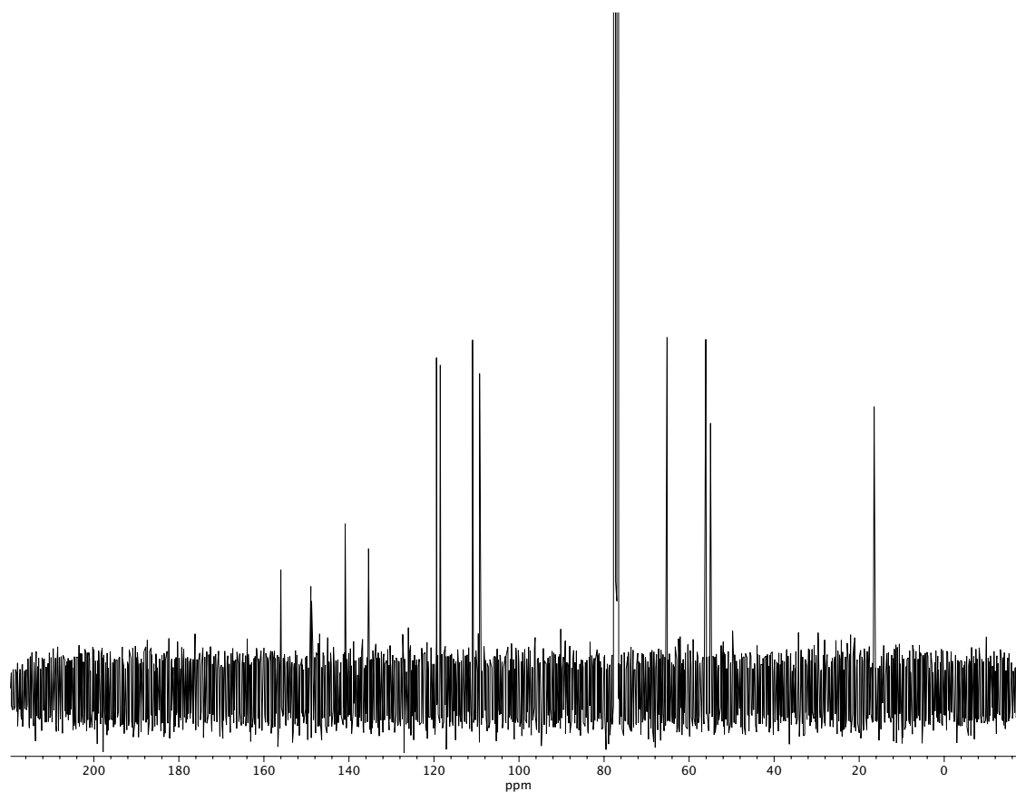
Figure A1.98 13 C NMR (100 MHz, CDCl 3 ) of compound 31I .
