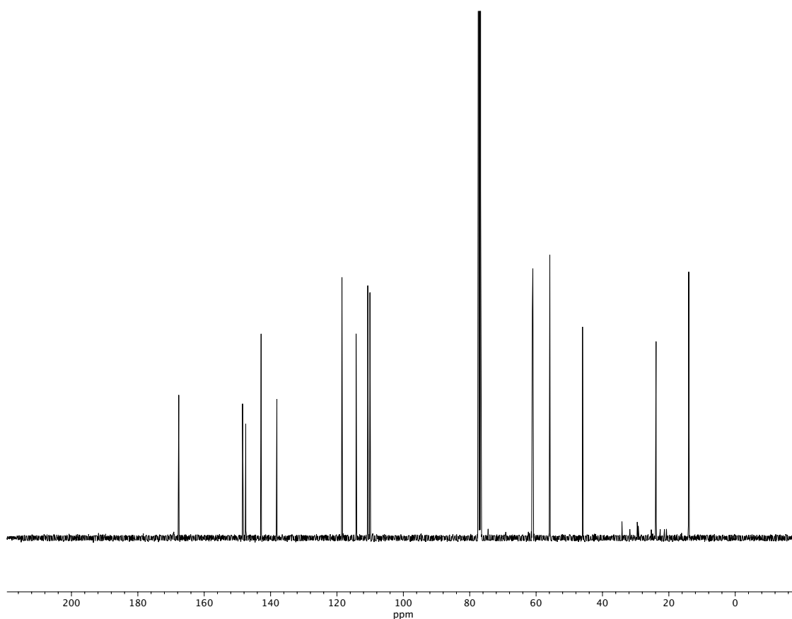
Figure A1.47 13 C NMR (100 MHz, CDCl 3 ) of compound 32I .
