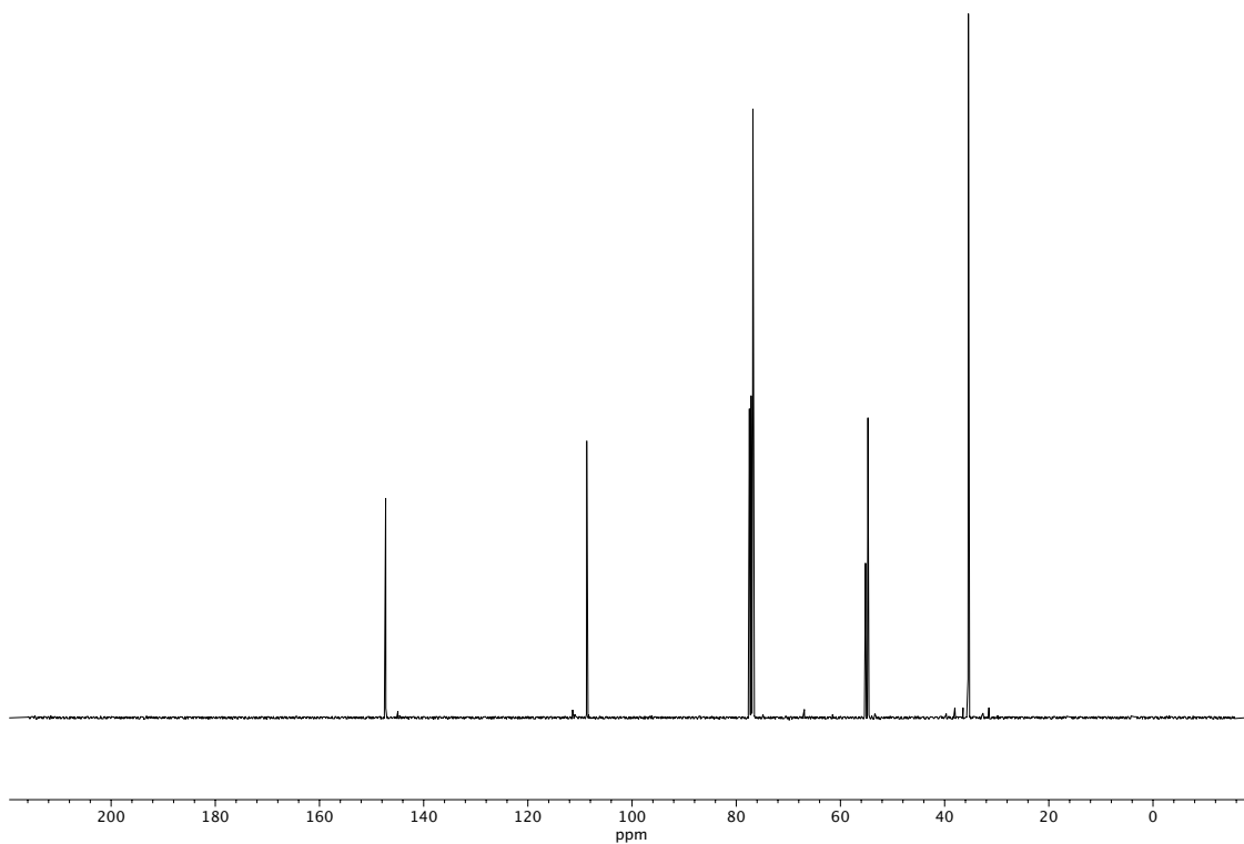
Figure A1.21 13 C NMR (100 MHz, CDCl 3 ) of compound 81 .
