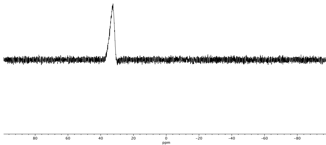
Figure A5.15 ^{11}\text{B} NMR spectrum (128 MHz, \text{CDCl}_3 ) of compound 150 .
