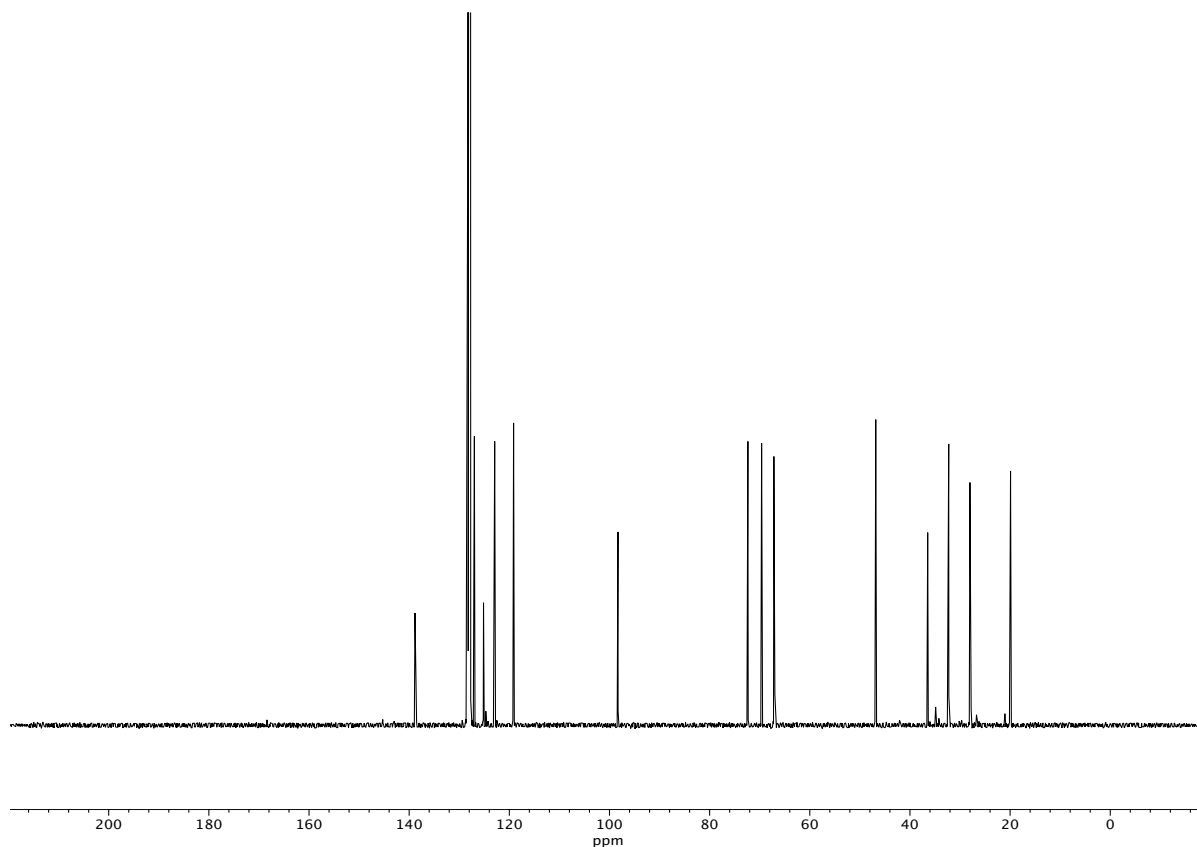
Figure A5.24 13 C NMR (100 MHz, C 6 D 6 ) of compound 155 .
