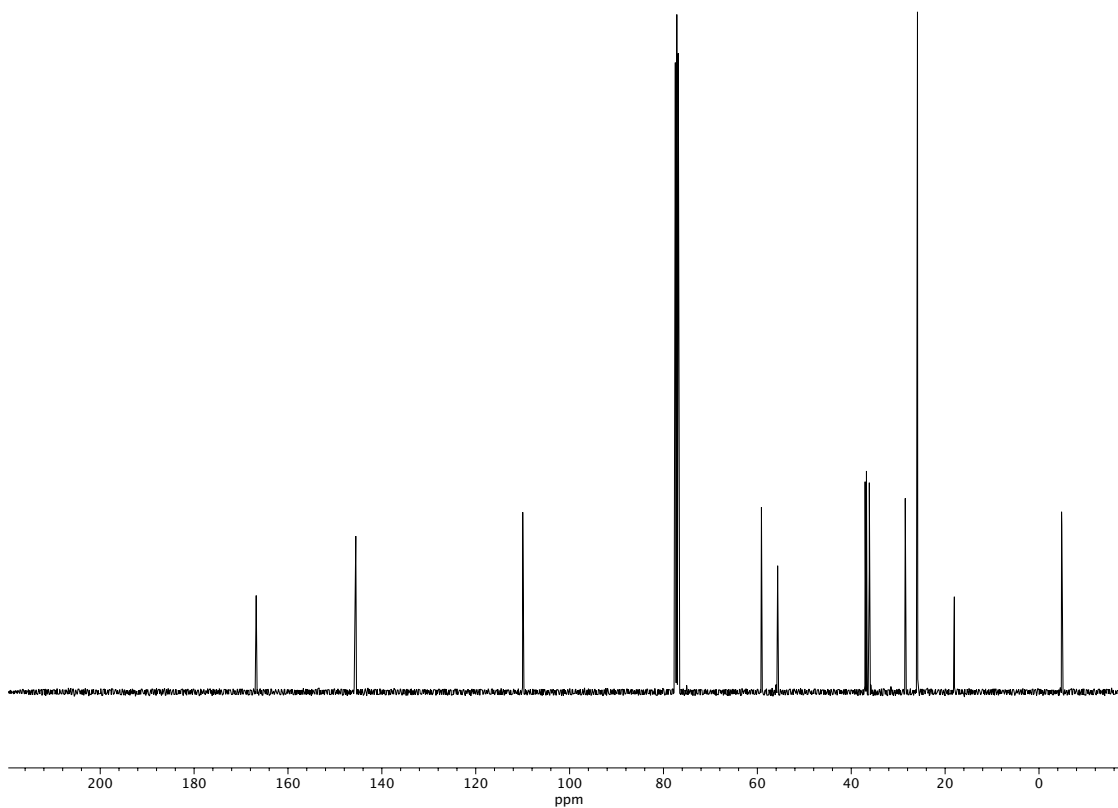
Figure A3.36 13 C NMR (100 MHz, CDCl 3 ) of compound (E)-86.
