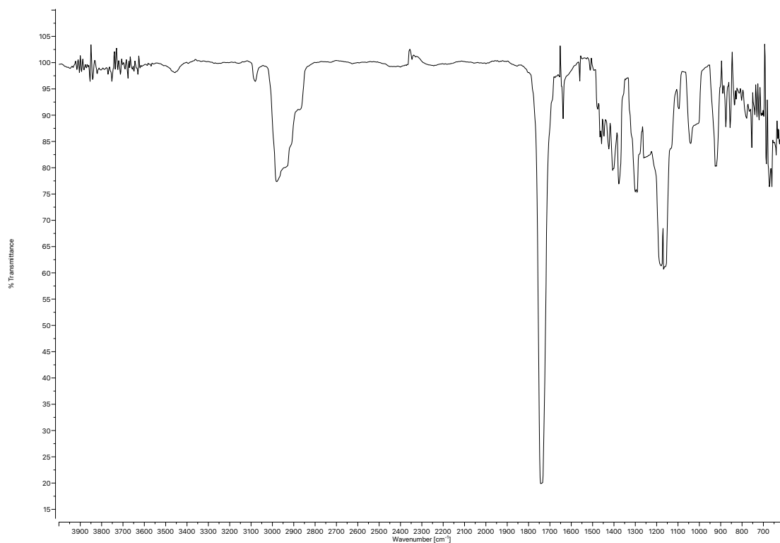
Figure A3.11 Infrared spectrum (Thin Film, NaCl) of compound 80 .
