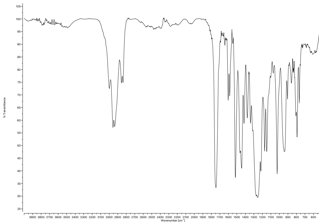
Figure A1.97 Infrared spectrum (Thin Film, NaCl) of compound 31I .
