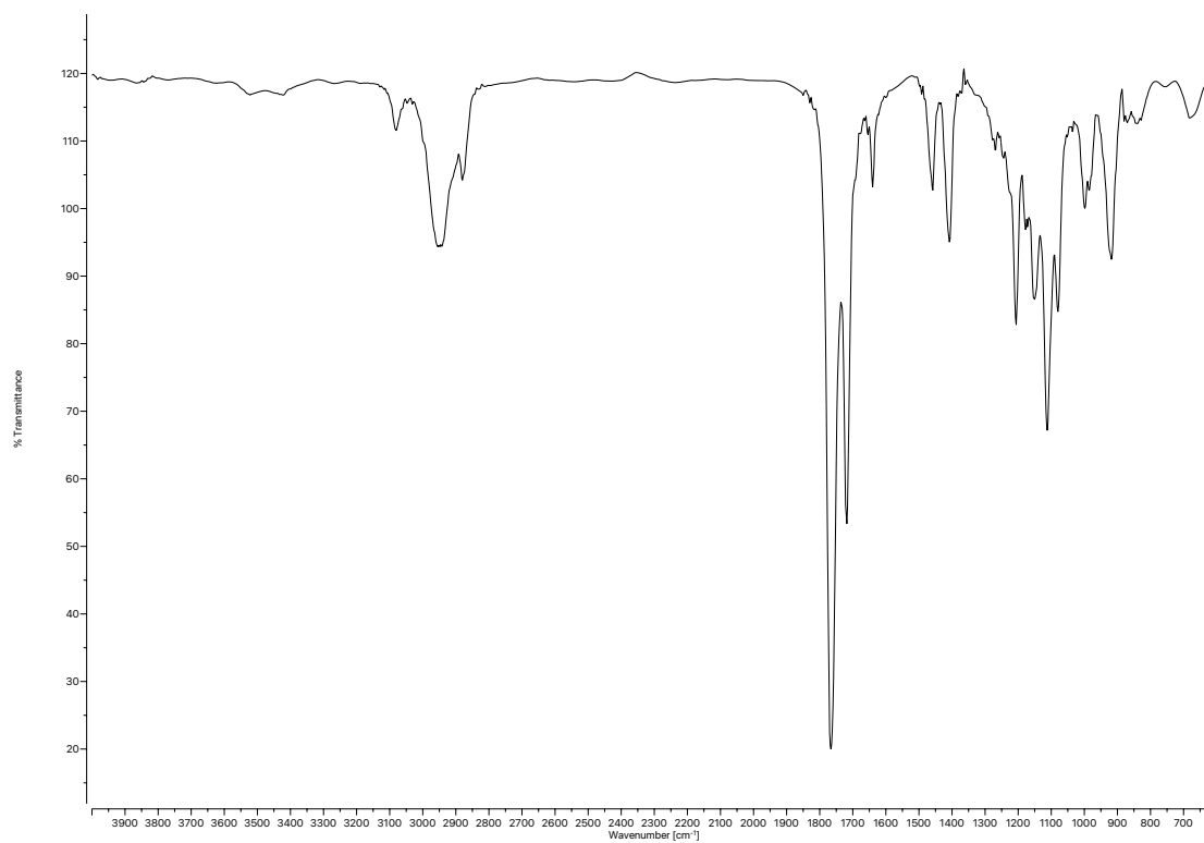
Figure A3.14 Infrared spectrum (Thin Film, NaCl) of compound 68 .
