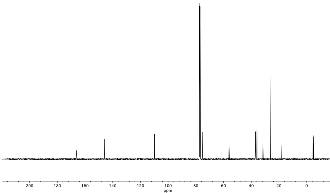
Figure A3.33 13 C NMR (100 MHz, CDCl 3 ) of compound (Z)-86.
