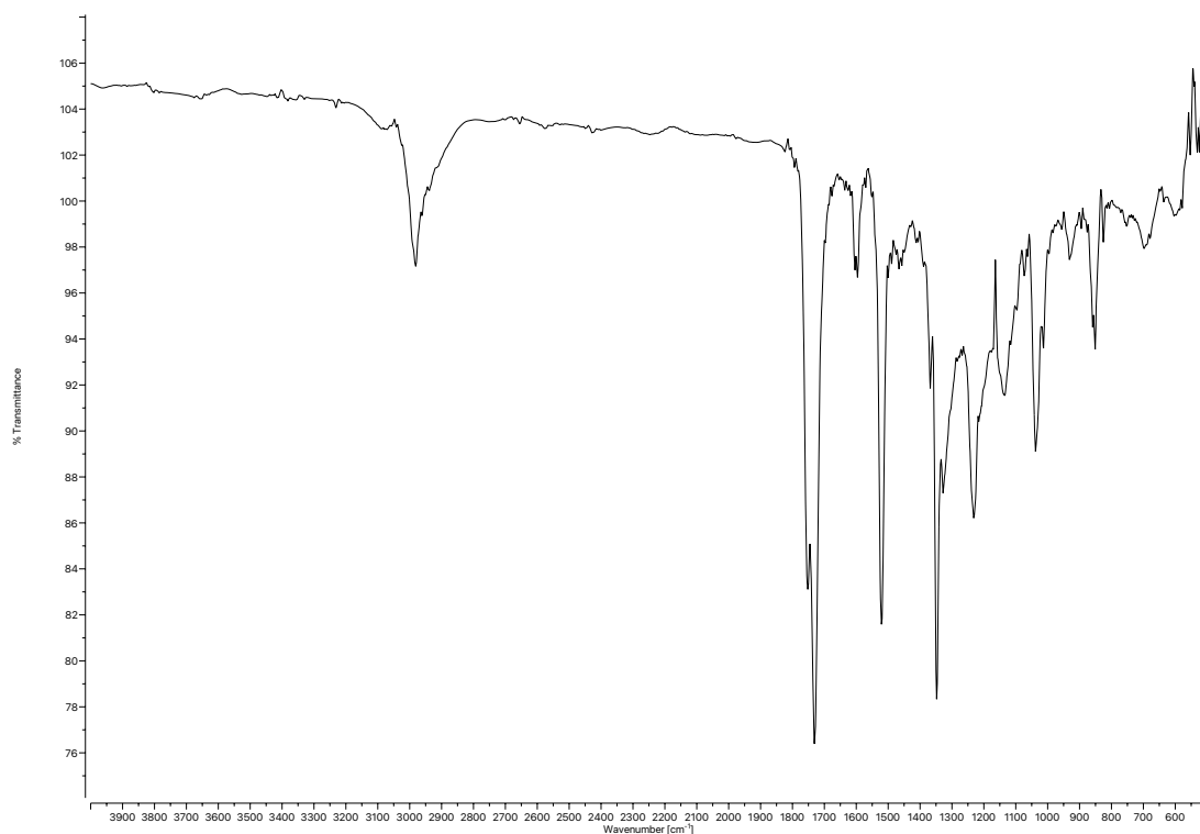
Figure A1.43 Infrared spectrum (Thin Film, NaCl) of compound 32k .
