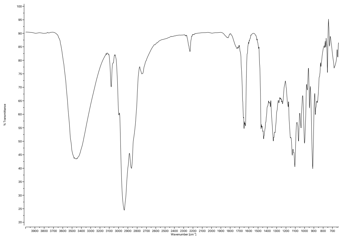
Figure A3.41 Infrared spectrum (Thin Film, NaCl) of compound 88 .
