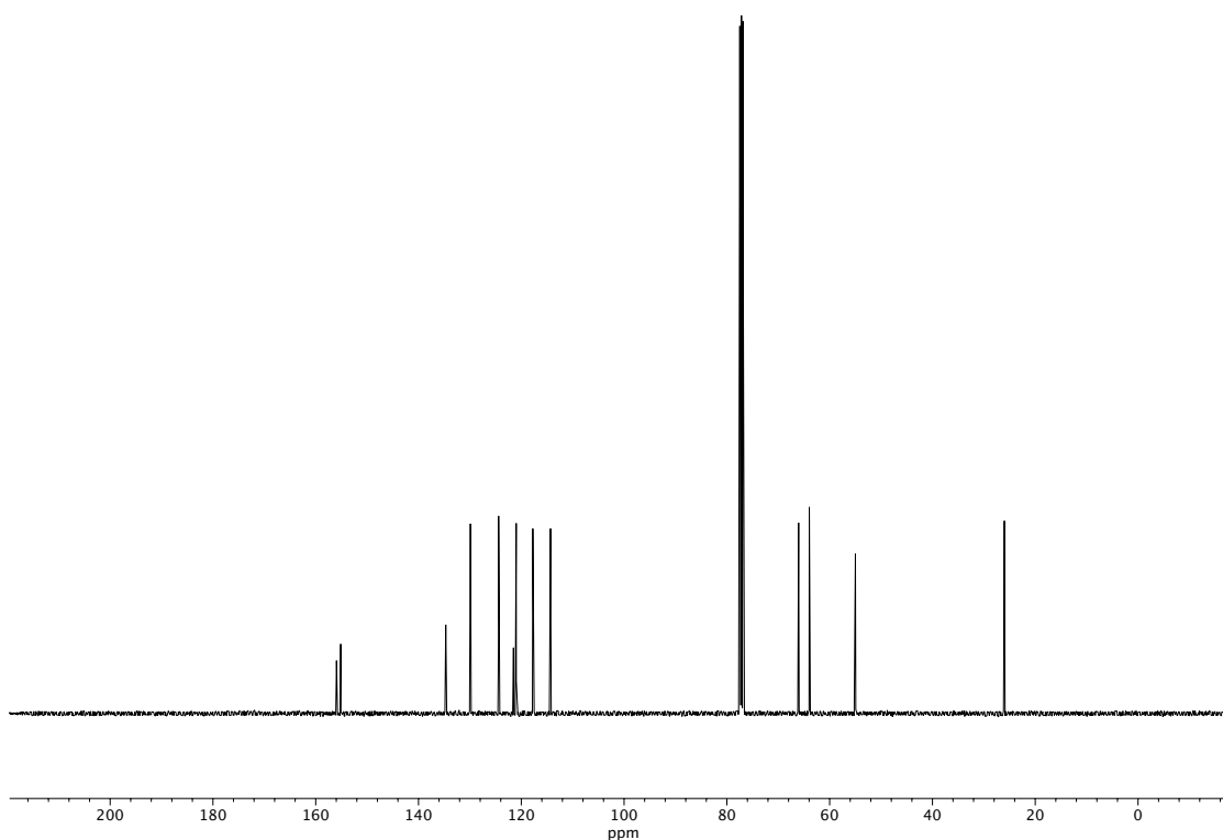
Figure A1.119 ^{13}\text{C} NMR (100 MHz, \text{CDCl}_3 ) of compound 31s .
