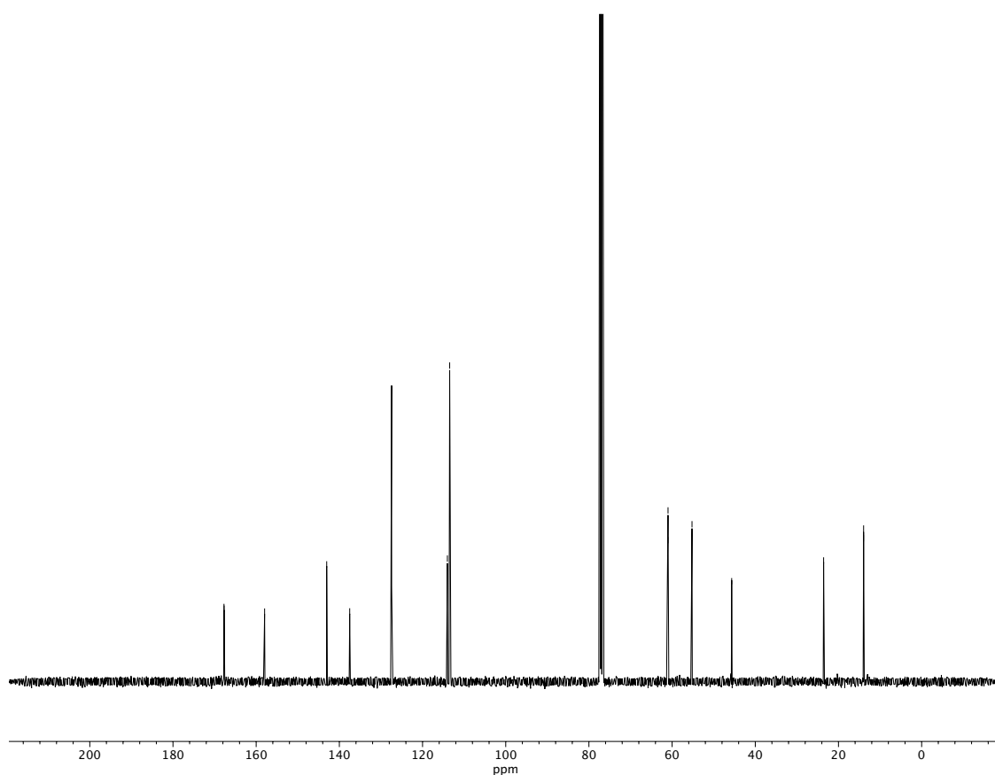
Figure A1.24 13 C NMR (100 MHz, CDCl 3 ) of compound 32e .
