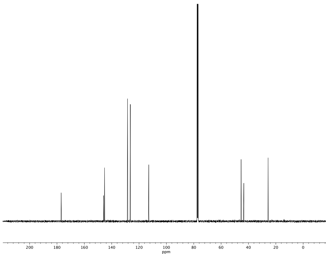
Figure A1.71 13 C NMR (100 MHz, CDCl 3 ) of compound 40 .
