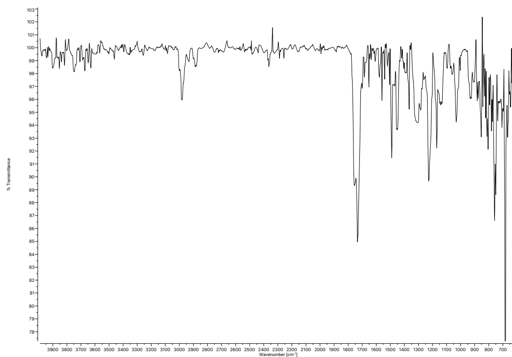
Figure A1.61 Infrared spectrum (Thin Film, NaCl) of compound 32s .
