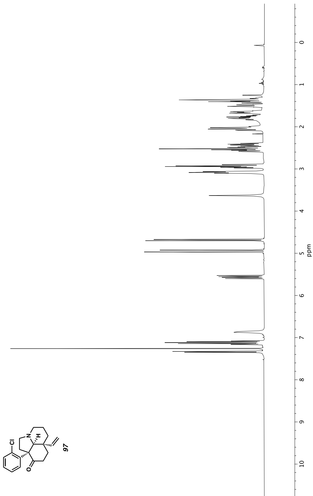
Figure A3.61 ^1\text{H} NMR (400 MHz, \text{CDCl}_3 ) of compound 97 .
