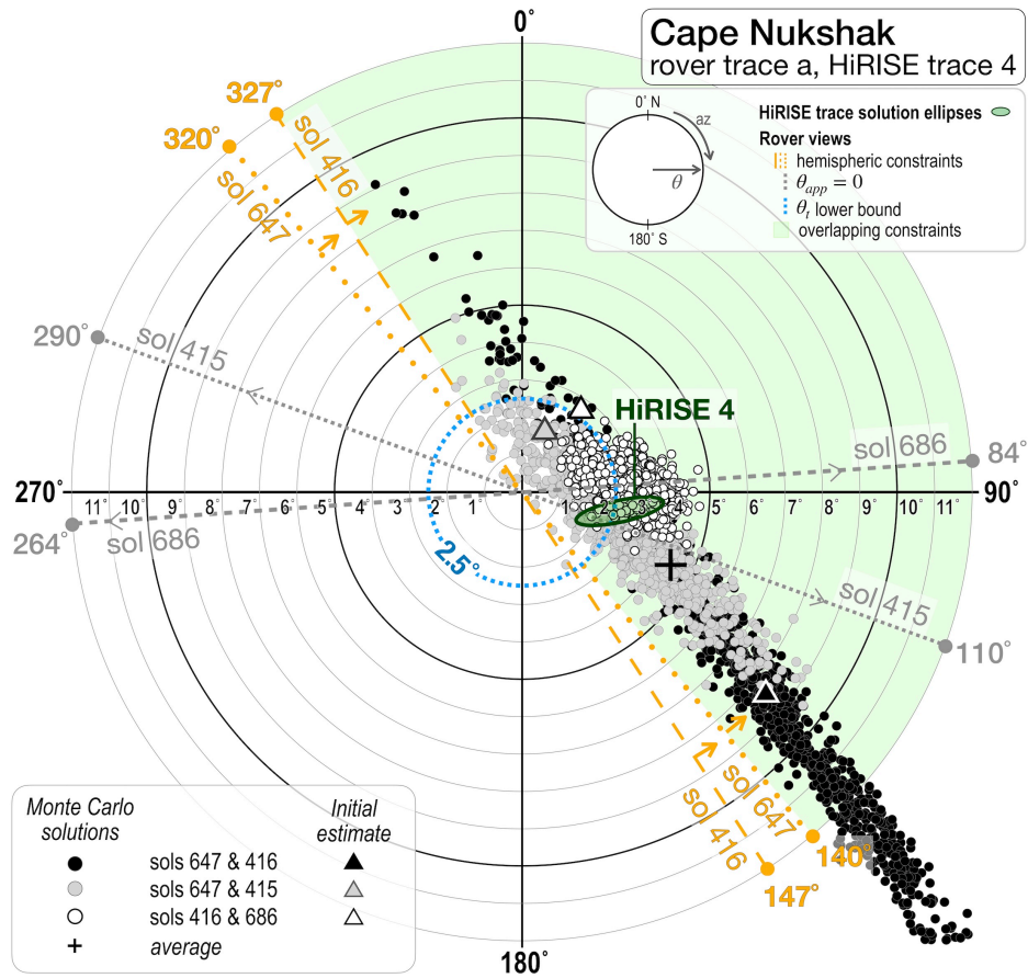
Figure 4: Rover-based orientation constraints (shaded light green) from \alpha_{z_{app}} and \theta_{app, max} (dotted blue line), rover-based Monte Carlo simulations (cloud of dots), and orbital-based HiRISE plane fits (shaded green ellipse) for Cape Nukshak. Triangles show the \alpha_{z_t} and \theta_t calculated from the initial estimates ( \theta_{app_0} ) for each image pair. “+” marks the average of the Monte Carlo solutions. Orange lines (dashed or dotted) demarcate lines of sight for Mastcam-Z images in which the trace appears inclined, with orange arrows indicating the direction of \alpha_{z_{app}} . Gray lines (dashed or dotted) show the line of sight for images in which the traced surface appears horizontal.
