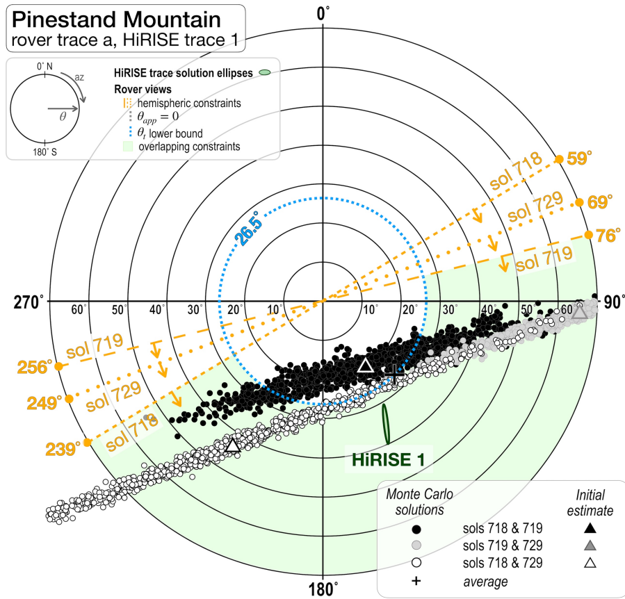
Figure 14: Rover-based orientation constraints (shaded light green) from \alpha_{z_{app}} and \theta_{app, max} (dotted blue line), rover-based Monte Carlo simulations (clouds of dots), and orbital-based HiRISE plane fits (shaded green ellipse) for Pinestand Mountain rover trace a . Triangles show the \alpha_{z_t} and \theta_t calculated from the initial estimates ( \theta_{app_0} ) for the image pairs. “+” marks the average of the Monte Carlo solutions. Orange lines (dashed or dotted) demarcate lines of sight for Mastcam-Z images in which the trace appears inclined, with orange arrows indicating the direction of \alpha_{z_{app}} .
