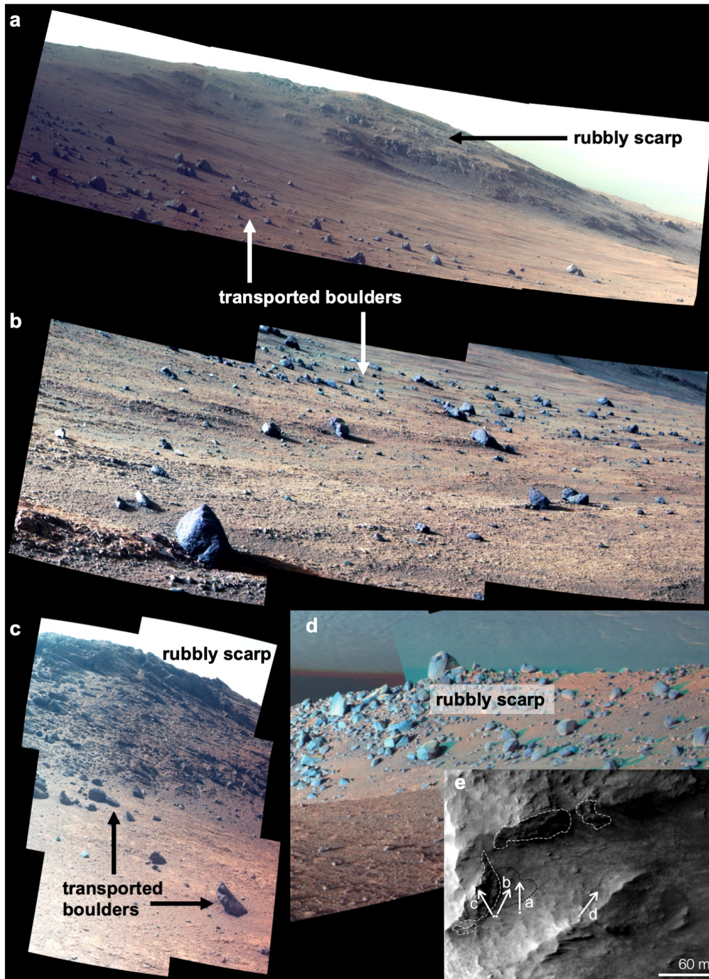
Figure 6: Pancam images of rubbly scarps and transported boulders in Marathon Valley. All images are of enhanced color to highlight subtle differences. a: Sol 4104, north wall of Marathon Valley. b: Sol 4092, rock survey near head of Marathon Valley. c: Sol 4082, north wall. d: Sol 4267 (cropped), ridge on southeast rim of the valley. Rover locations and approximate look directions are in e , which uses HiRISE image ESP_018701_1775 and the same extent as Figure 4c .
