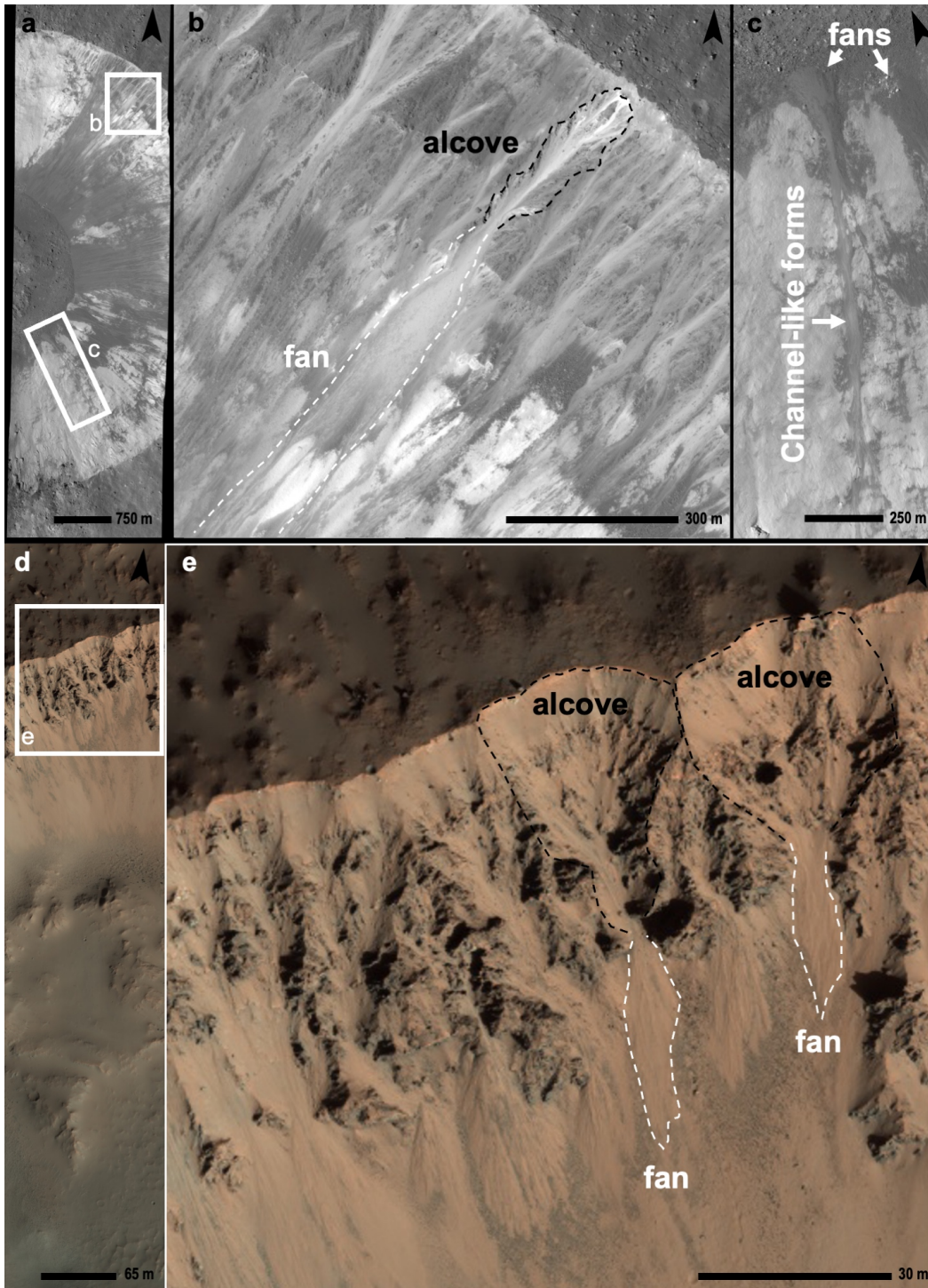
Figure 1: Examples of chute morphologies on the Moon and Mars. Panels a , b , and c show alcoves, chutes and fans in a low-latitude lunar crater captured in LROC image M152451994R. Panels d and e show alcoves, bedrock chutes and fans on the rim of a martian crater captured by HiRISE image ESP_019120_1585, centered at \sim 21^\circ latitude.
