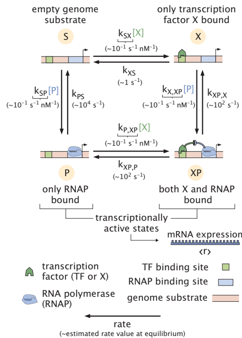
Figure 4.1: Structure of a fundamental gene-regulatory motif. A square cycle of four-states emerges when up to two molecules (such as a transcription factor X and polymerase P ) can bind to a common substrate (say a genome). Output observables \langle r \rangle are linear combinations of the state probabilities; for instance, mRNA production scales with the probabilities of transcriptionally active states where polymerase is bound to the genome (states P and XP ). These outputs vary with the control parameter [X] , here schematized as the concentration of a transcription factor. (Numerical values of rate constants underneath edges are biologically plausible values, as inferred in the SI §2B.)
