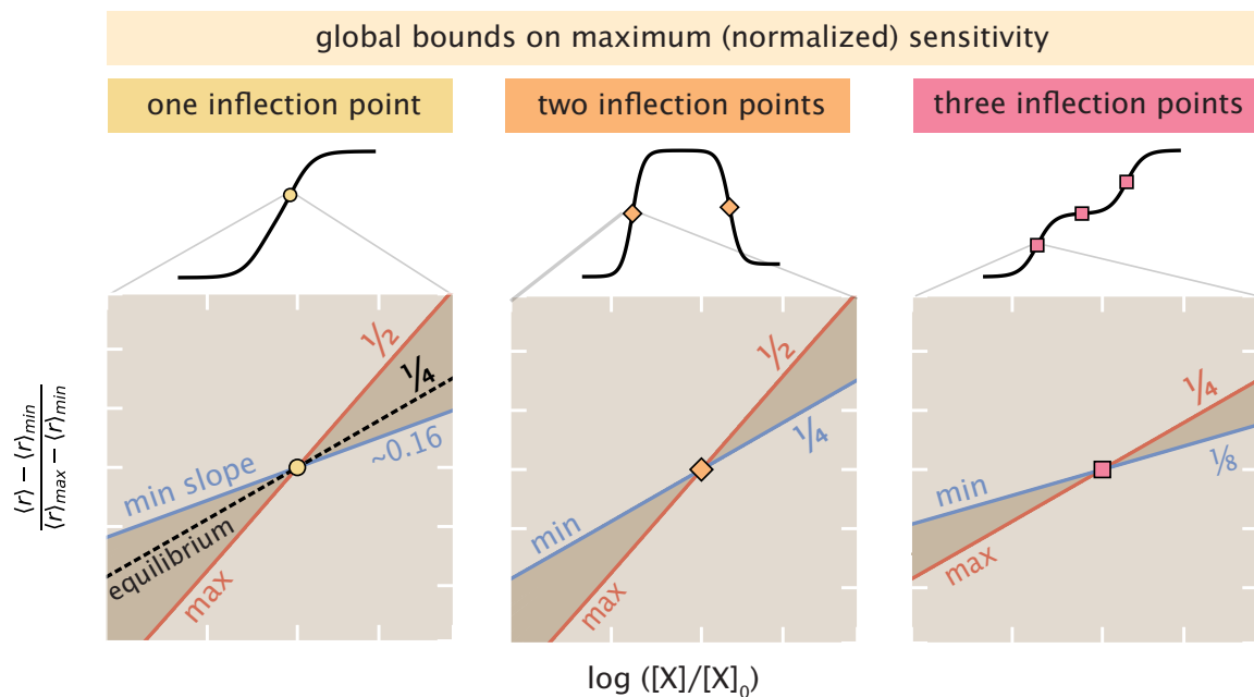
Figure 4.4: Global bounds, in or out of equilibrium, restrict maximal (normalized) response sensitivity (with respect to input concentrations [X] on a log scale). The normalized responses \frac{\langle r \rangle - \langle r \rangle_{\min}}{\langle r \rangle_{\max} - \langle r \rangle_{\min}} are plotted near points of inflection that maximize slope, separated by shape phenotype. When the output has one inflection point (left), the maximal sensitivity is bounded between a minimum of 0.16 (blue line) and a maximum of 1/2 (red line) for any set of rate values or any dissipation; this subsumes the equilibrium case, whose normalized sensitivity is fixed at 1/4 (black dotted line). When the output has two inflections (middle), the maximal sensitivity is bounded between 1/4 and 1/2 . When the output has three inflections (right), the maximal sensitivity is bounded between 1/8 and 1/4 .
