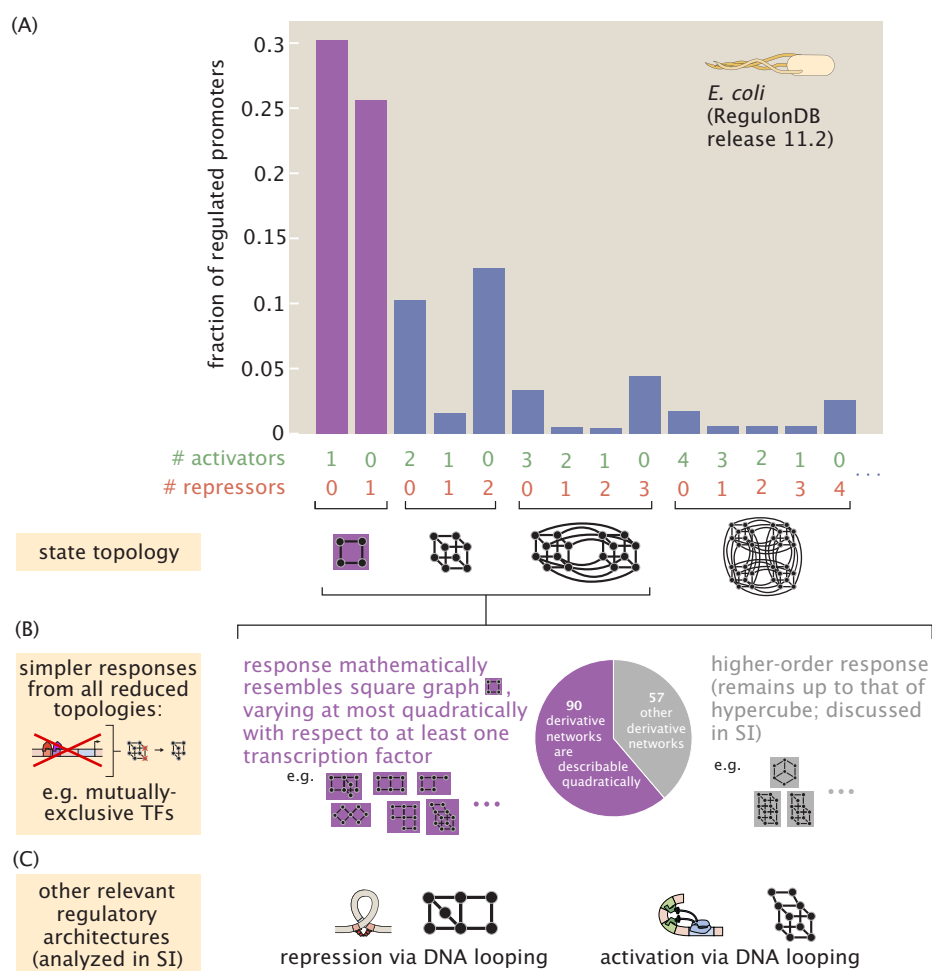
Figure 4.2: Incidence of regulatory architectures for transcription, where a square cycle's response is common. (A) Regulatory architectures reported in E. coli , organized by the numbers of activating and repressing transcription factors associated with each regulated promoter, according to data in the RegulonDB database [19] release 11.2. Over half of these regulated promoters are reported to be regulated by the most common architecture of a single transcription factor (purple bars), and thus can be described by a square graph of states (Fig. 4.1). Less common network architectures with multiple transcription factors form hypercubic state spaces whose complete responses are analysed in the Supporting Information (SI). (B) While larger binding networks can generically show more complex regulatory responses than the square cycle, simpler topologies and responses result from restrictions like overlapping binding site (see SI §3D). Over half of all nontrivial transcriptionally-potent derivative networks formed by up to three transcription factors show a response that resembles the square graph with respect to at least one transcription factor. (C) Transcriptional regulation by DNA looping accomplishes distinct responses, whose properties are analyzed algebraically and numerically in the SI.
