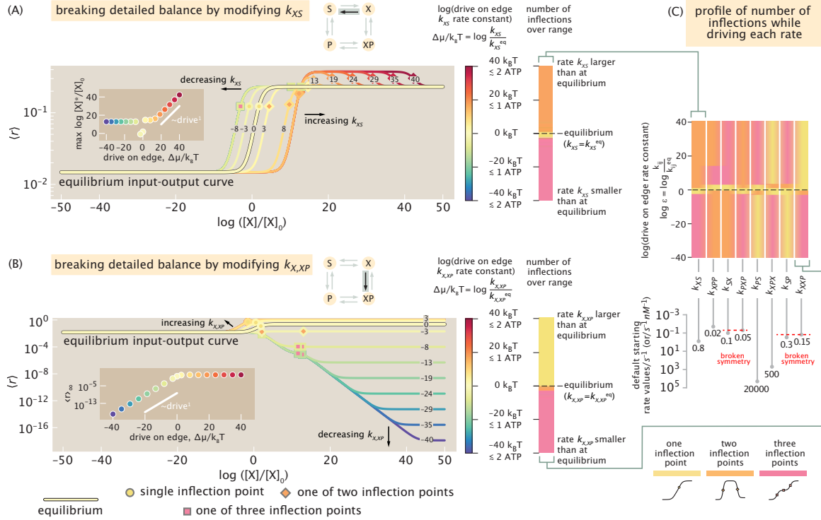
Figure 4.5: Systematically breaking detailed balance edge-by-edge. (A) Example of how spending energy to modify a single rate (here, k_{XS} )—while the seven other rates remain fixed—changes the response curve away from default equilibrium behavior (pale yellow curve labeled “o” net drive and outlined in black). Responses from rate values larger than (or smaller than) at equilibrium are shown in increasingly red (or blue) colors, respectively; curves are also labeled with the numerical values of the net drive that generated them in k_B T units (positive for an increase; negative for a decrease). Each curve’s resulting inflection points are marked by yellow, orange, or pink markers, denoting one to three inflection points (respectively), and summarized in the associated one-dimensional (shape phenotypic) phase-diagram with the same colors on the right. Inset: the position of the final inflection point \max \ln [X]^{*}/[X]_0 versus net drive (power law exponent is \sim 1 ). (B) Another representative behavior is displayed when k_{X,XP} is instead the rate varied. Inset: the saturation \langle r \rangle_{\infty} versus net drive (power law exponent is \sim 1 ). (C) Summary of how all eight rates respond to energy expenditure to realize different regulatory shape phenotypes. Below, stem plots give precise values of each default rate constant at equilibrium. (These rates satisfy initial “broken symmetries” that violate the conditions in Eq. 4.5 by default, facilitating more ready access to nonmonotonicity. The SI §2K documents the impact of departing from different default starting rates that instead satisfy Eq. 4.5, in addition to the impacts of driving all other edges.) (Here, the reference concentration scale setting the horizontal offset of the concentration axis is [X]_0 \equiv 1 \text{ nM} .)
