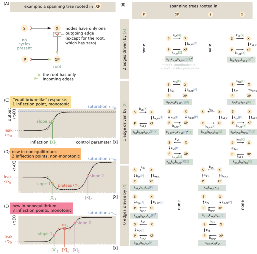
Figure 4.3: Nonequilibrium response of the four-state fundamental transcriptional motif. (A) An example of a spanning tree (rooted in state XP) like those that define steady-state probabilities via the Matrix Tree Theorem. (B) All 16 directed, rooted spanning trees of the four-state cycle in 1(A): trees are grouped by the root state (in columns) and by how many participating edges depend on the control parameter X (in rows). As guaranteed by the Matrix Tree Theorem, the steady-state probability of any state—in or out of equilibrium—is given by the sum of the weights of these spanning trees, introducing up to a quadratic dependence in X in any output, as represented by Eq. 4.1. (C-E) Three universal output behaviors ( regulatory shape phenotypes ) can result from this architecture. A monotonic “equilibrium-like” output (C) manifests a Hill-like or MWC-like response, behavior familiar from equilibrium thermodynamic models. However, exclusively out of equilibrium, new multiply-inflected regulatory shape phenotypes become possible. Under drive, outputs can (D) vary non-monotonically and reach two inflection points with the control parameter; or show three inflection points and vary monotonically (E). These richer phenotypes show a wider set of properties that characterize each curve: these include the “leak” value of the observable when the control variable is absent ( \langle r \rangle_0 = \langle r \rangle([X] = 0) , in orange; the saturation asymptotic limit as the control variable is maximally present ( \langle r \rangle_\infty = \lim_{[X] \rightarrow \infty} \langle r \rangle ; in light blue); the observable’s values at intermediate plateau regions ( \langle r \rangle_* ; in red); and slopes 1 and 2 at inflection points [X]_1 and [X]_2 when they are defined (in green and purple, respectively).
