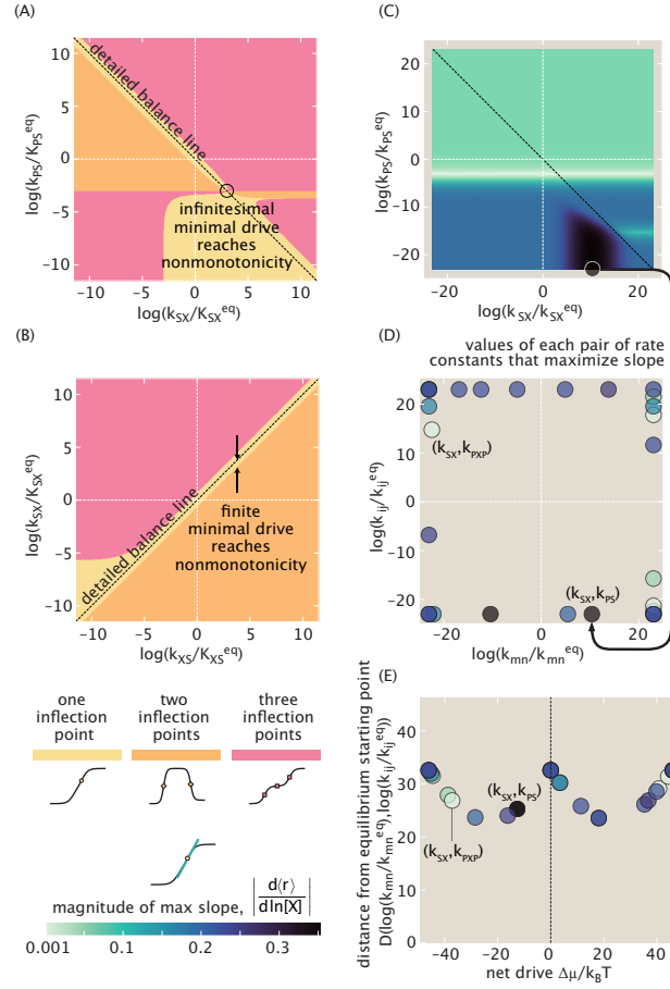
Figure 4.6: Breaking detailed balance along two edges unlocks higher sensitivity and multiply-inflected outputs with smaller drive than required for breaking detailed balance along single edges. (A) Adjusting the rate pair (k_{SX}, k_{PS}) —while fixing the other six rates at their default biological values at equilibrium (of Figure 4.3A and Figure 4.5C’s stem plot)—varies the number of inflection points (light yellow: one inflection, orange: two inflections, pink: three inflections), in a 2D analog of Figure 3. Specifically, this rate pair illustrates a case where nonmonotonic two-inflection curves can be reached with only an infinitesimal net drive. (B) In contrast, when tuning (k_{XS}, k_{SX}) , a finite minimum drive is needed to access nonmonotonicity; numerical sampling reveals that this total drive is the same as required while only tuning one edge at a time. (C) Maxima of raw slope d\langle r \rangle / d \ln [X] / [X]_0 over the same modulations (axes) of the rate pair (k_{SX}, k_{PS}) shown in (A), with slope-maximizing rates within the permissible rate space indicated with a circle. [X]_0 \equiv 1 nM is a reference concentration. (D) Overlaying the same positions of maximal slope for all twenty-eight rate pairs emphasizes that optimal slopes are found at the boundary of the permissible rate space. Marker colors reflect the maximal slope achieved for each rate pair. Panel (E) summarizes the behavior of panel (D) by representing each optimal rate pair value with two important natural parameters: the net drive \Delta\mu/k_B T (either the log ratio or log product of each rate’s difference from their equilibrium starting values, depending on the relative (counter)clockwise orientation of the rates in a pair); and the net total distance the optimal values are found from their starting values in
