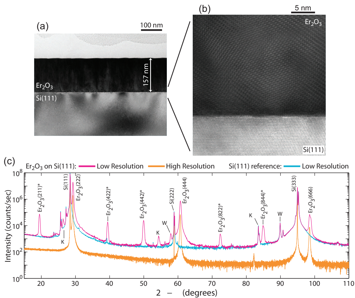
Figure 4.2: \text{Er}_2\text{O}_3 grown via ALE on \text{Si}(111) . (a) TEM image of an \text{Er}_2\text{O}_3 layer on \text{Si}(111) . (b) High-resolution TEM image of \text{Er}_2\text{O}_3 -Si interface showing a sharp boundary between the two materials. (c) XRD spectrum for \text{Er}_2\text{O}_3 on \text{Si}(111) and a reference \text{Si}(111) sample; the (*) peaks designate strained layers as described in the text.
