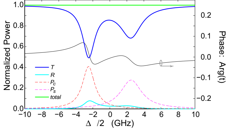
Figure 1.5: Power conservation and phase shift for the transmitted field ( \mathbf{t} ) as a function of detuning for a waveguide coupled to a doublet resonance with \{\gamma_e, \gamma_{c,i}, \gamma_{s,i}, |\kappa_{cb}|\}/2\pi = \{0.5, 1.25, 2.5, 2.5\} GHz. The total power dissipated by the j th mode is P_j = \gamma_{j,i}|a_j|^2 .
