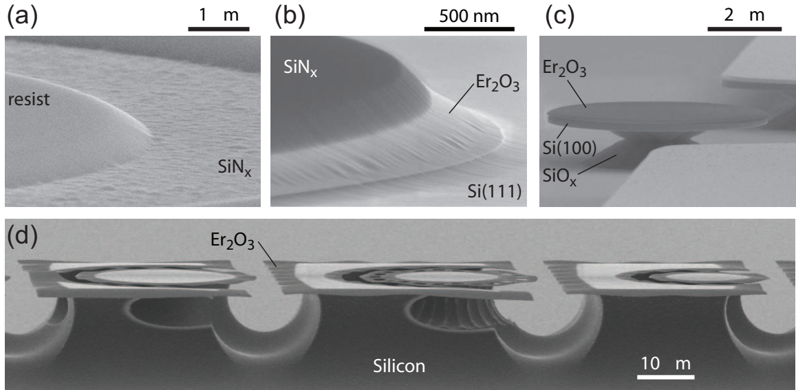
Figure 4.3: Processing Er 2 O 3 microdisk cavities. (a) A reflowed resist mask on an early sample develops small pseudopodia as the ZEP clings to features in the SiN x that are transferred up from an irregular Er 2 O 3 layer. (b) Er 2 O 3 microdisk edge prior to the SF 6 undercut. (c) Hybrid Er 2 O 3 -Si microdisk (78 nm Er 2 O 3 , 188 nm Si, 1 \mu\text{m} SiO x ) after the final HF undercut of the buried oxide. (d) SEM image of the final microdisk cavities showing the effects of the relaxed strain and the SF 6 undercut. These devices are isolated for use with a straight taper.
