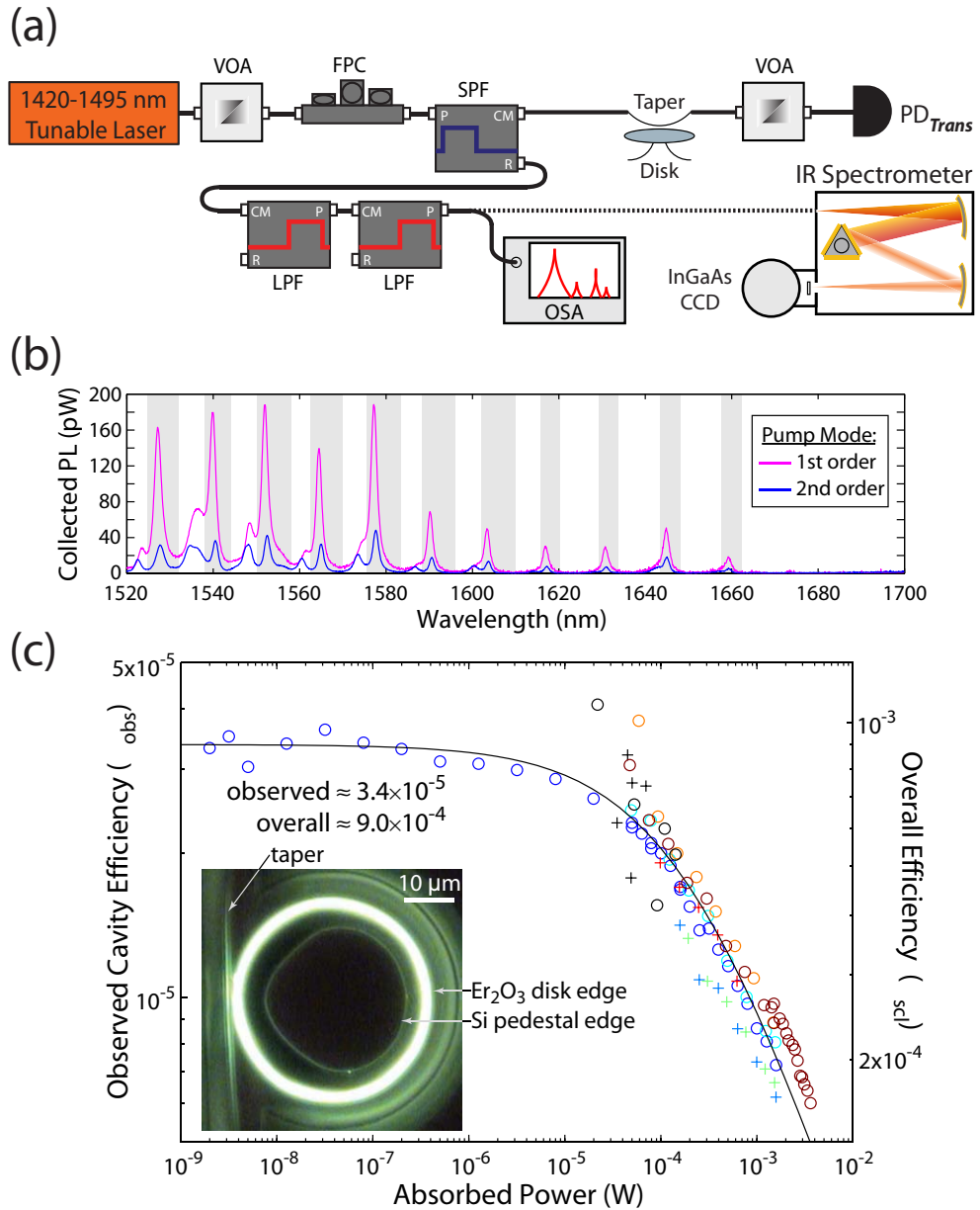
Figure 4.9: (a) Setup for measuring C/L-band PL and \eta_{obs} . (b) Observed cavity-coupled PL for the device in Fig. 4.4; the TE p=1 modes are highlighted in gray. (c) Power-dependent radiative efficiency of the ^4I_{13/2} \rightarrow ^4I_{15/2} transition. The marker color indicates the pump-mode wavelength from blue (1460.9 nm) to dark red (1494.5 nm) while (o) and (+) designate first- and second-order radial pump modes, respectively. Black markers represent data from devices on another wafer processed with wet chemical etching and using first- and second-order pump modes (spanning 1437.6–1490.9 nm). The inset shows green upconverted luminescence from a TE p=1 mode [35].
