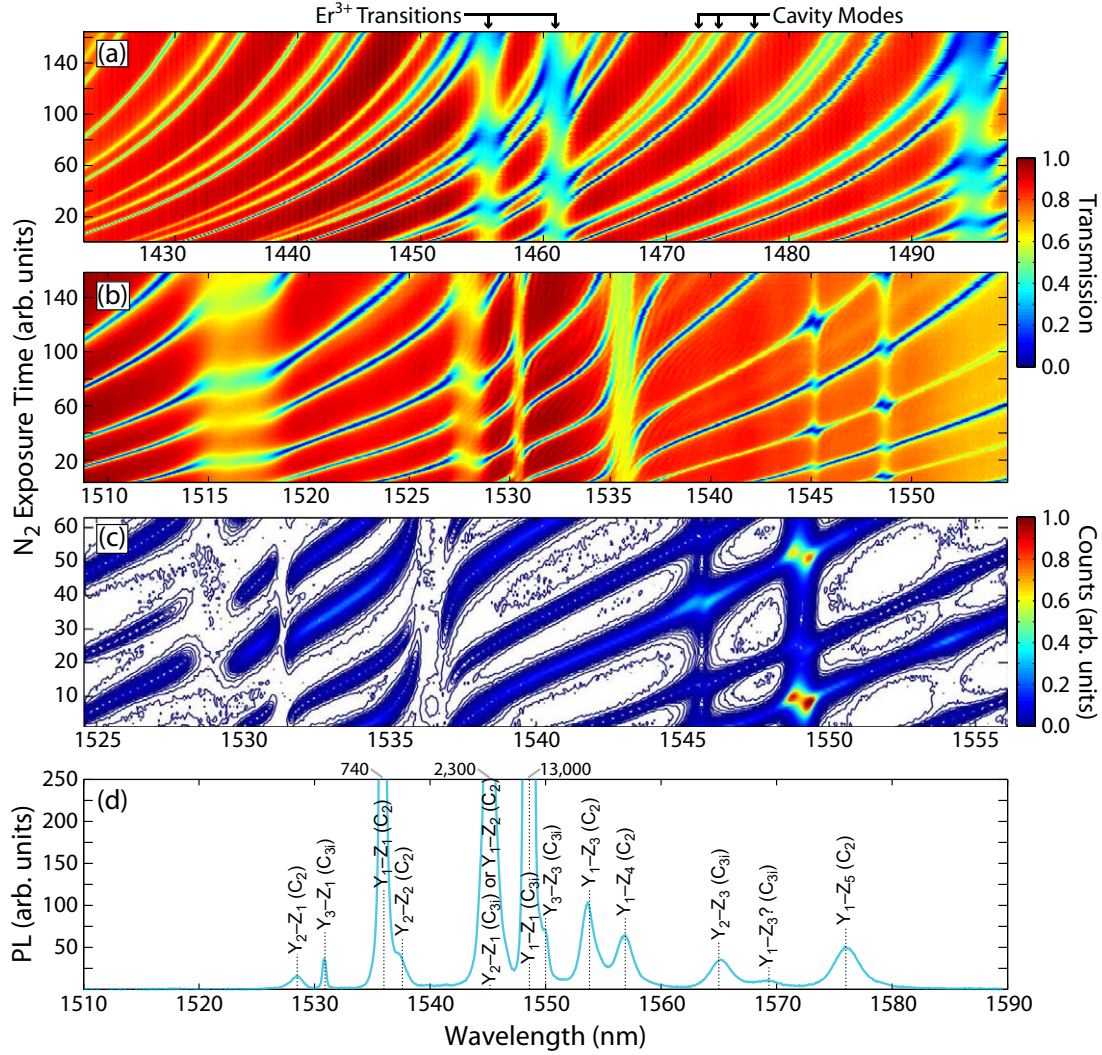
Figure 4.10: Cavity transmission spectra in the (a) S-band and (b) C-band at 8.6 K tuned using N_2 deposition. The shallow background ripple is residual-etalon noise from the tunable lasers or ringing from the notch filters used to filter out that noise. (c) Taper-collected PL spectrum as the cavity is tuned. Equal spaced contours ( \Delta = 0.002 ) are used to display low-intensity features. The Er^{3+} ions are excited by resonantly pumping a WGM near 1480 nm. (d) Identified transitions in the bulk PL spectrum at 8.6 K.
