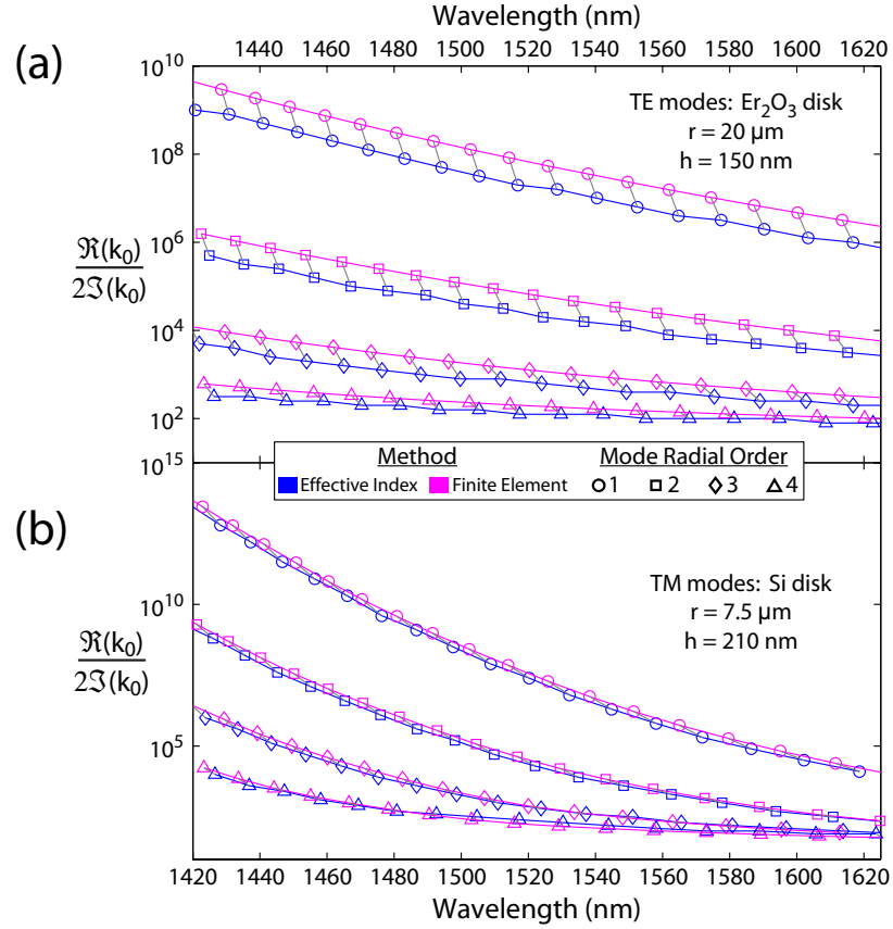
Figure 1.3: Comparison of the eigenvalues ( k_o ) found using effective-index and finite-element models for (a) TE modes in a \text{Er}_2\text{O}_3 disk and (b) TM modes in a Si disk plotted against free-space wavelength [ \lambda_o = 2\pi/\Re(k_o) ]. The solutions for the two models giving the same QNM are connected by grey lines.
