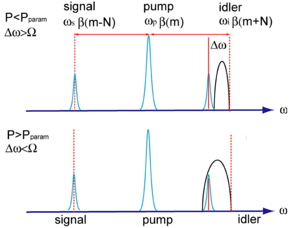
Figure A.1: Schematic of the effect of cavity detuning on the occurrence of parametric oscillation. For \Delta\omega > 0 , parametric oscillation can only occur if the detuning \Delta\omega = 2\omega_p - \omega_s - \omega_i is less than the parametric band-width (given by 0 < \Delta\omega < \Omega ). Note that the parametric band-width exists only for positive detuning, due to the shift of resonant frequency caused by XPM and SPM.
