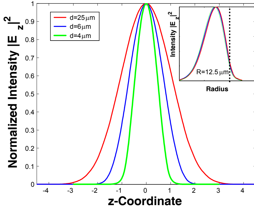
Figure 7.12: Radial (inset) and polar (main figure) intensity distribution for a microsphere ( D = d = 25\mu m ) and toroid microcavities ( d = 6\mu m, d = 4\mu m ). The polar scan is taken at a radial position corresponding to the maximum intensity.
