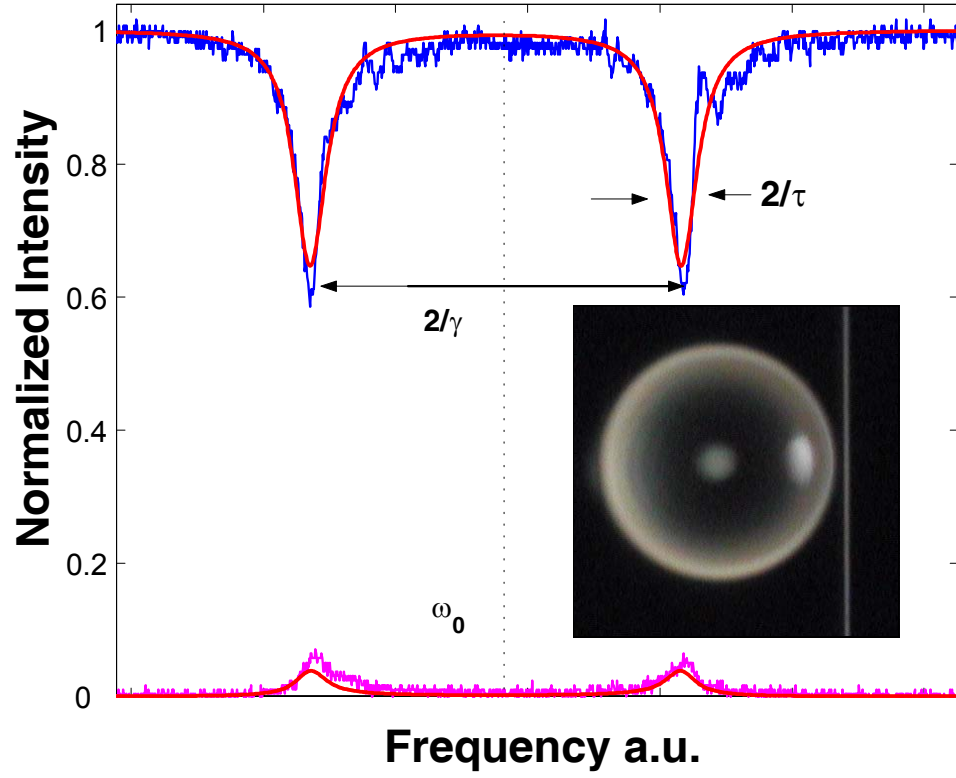
Figure 4.2: Spectral transmission and reflection properties of a 70 \mu\text{m} sphere with Q_0 = 1.2 \cdot 10^8 [50] in the regime of strong modal coupling with \Gamma = 10 . The solid line represent a fit using the presented model from equation 1. The inset shows a microsphere coupled to a tapered fiber.
