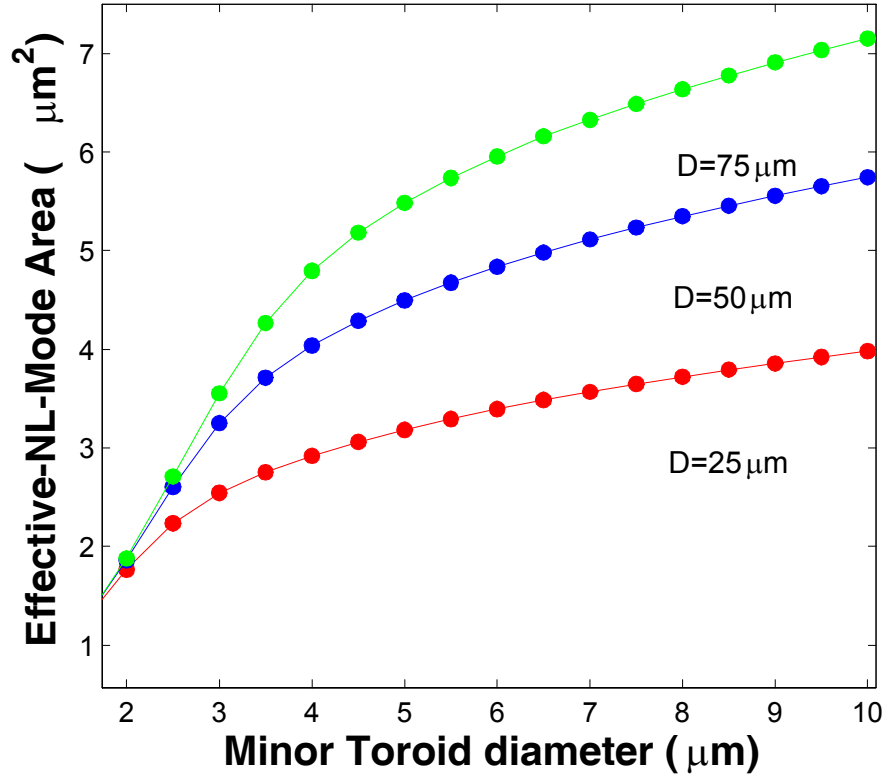
Figure 9.5: Effective mode area A_{eff} for a toroid microcavity as a function of minor toroid diameter ( d ), for three different principal diameters (25, 50, 75 \mu\text{m} ). The resonance wavelength in this simulation was adjusted to the 1550 nm band.
