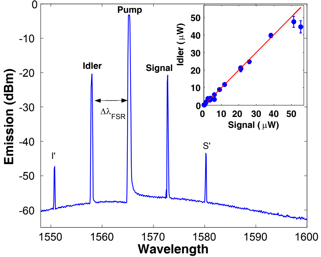
Figure 10.3: Parametric-oscillation spectrum measured for a 67\text{-}\mu\text{m} -diameter toroidal micro-cavity. The pump is located at 1565 nm and power levels are far above threshold. The signal and idler are modes with successive angular mode numbers and are spaced by twice the free spectral range ( 2 \times 7.6 nm). The subsidiary peaks (denoted I', S') only appeared at high pump powers and are due to a combination of nonlinear effects, such as parametric oscillation (of signal and idler) as well as four-wave-mixing involving the idler, pump and signal. Inset: idler emission power plotted versus the signal emission power, recorded for different pump powers. The idler-to-signal power ratio is 0.97 \pm 0.03 . For higher pump powers deviation is observed due to appearance of secondary oscillation peaks (I', S') (compare main figure).
