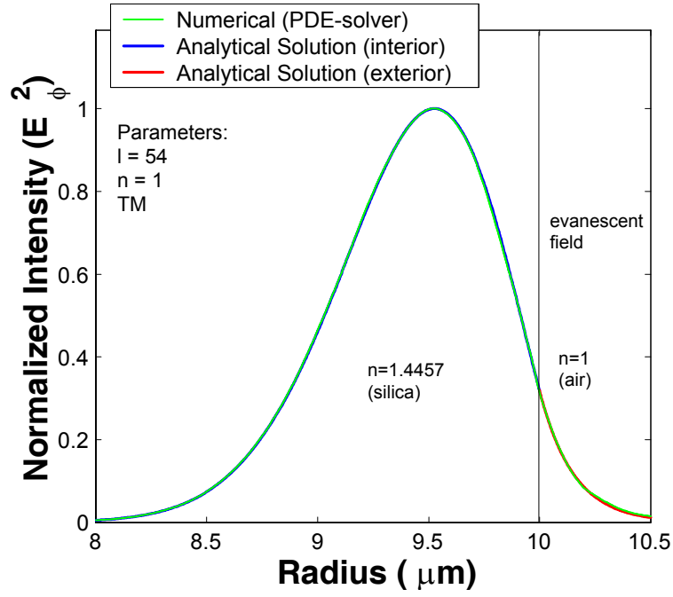
Figure B.2: Comparisson of the analytical and numerically calculated intensity distribution of the |E_\phi|^2 component plotted in the radial direction, for a microsphere of 10 \mu m radius. The numerical and analytical models show excellent agreement.
