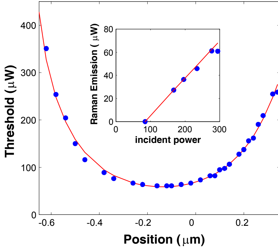
Figure 5.5: Coupling gap and size dependence of the Raman threshold. Main figure, Raman oscillation threshold vs. taper-sphere gap for a 40- \mu\text{m} -diameter sphere ( Q_0=10^8 ). Position is measured from the critical coupling point, where negative values correspond to the undercoupled regime. The minimum threshold occurs with the microsphere about 0.15 \mu\text{m} undercoupled, and corresponds to a transmission of 12%. Solid line, a theoretical fit to the threshold equation. Inset shows Raman power output (sum of forward and backward emission) vs. incident pump power. Differential quantum efficiency is 36%.
