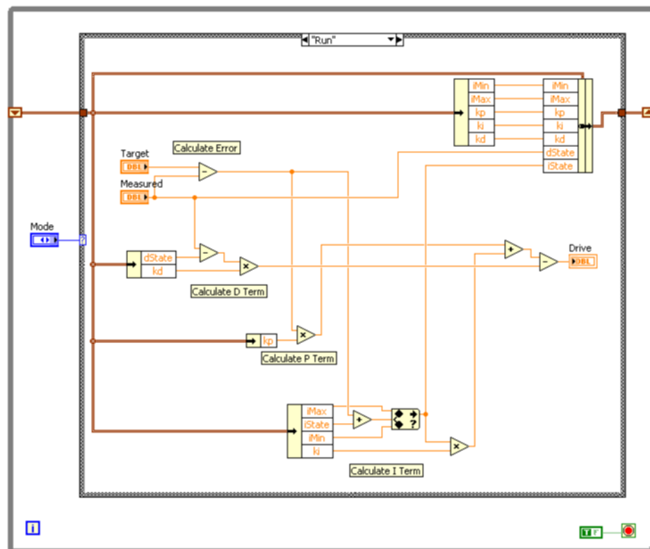
Figure B.3. PID algorithm implementation.
