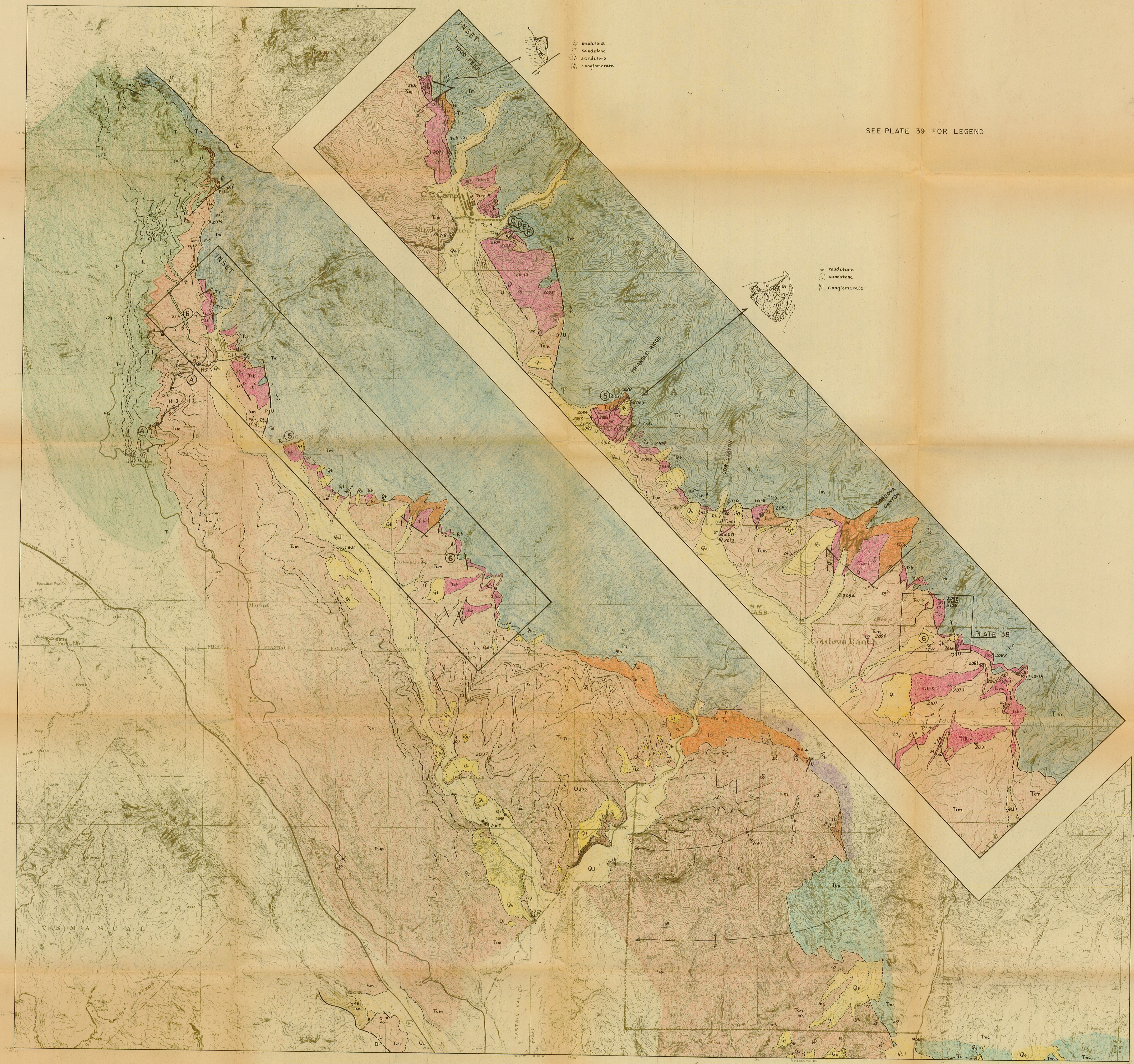
GEOLOGIC MAP OF THE CASTAIC FORMATION (NORTHERN MAP)
